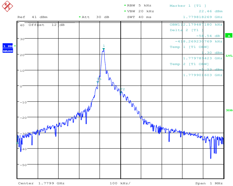
NB-IoT In-band band 66 132671 QPSK(99%)
