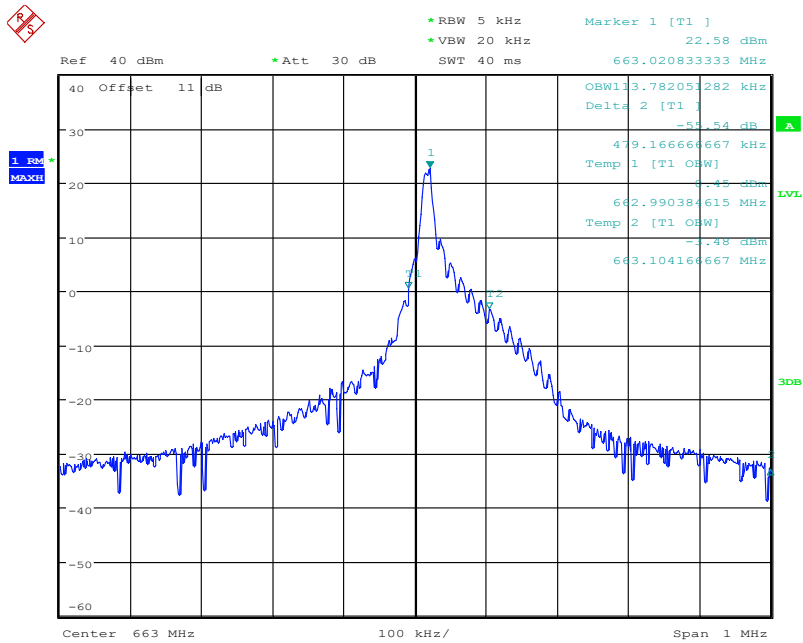
NB-IoT standalone band 71 133122 QPSK(99%)
