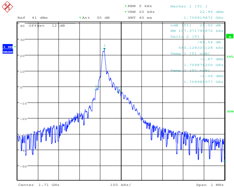
NB-IoT standalone band 66 131972 QPSK(26dB)
