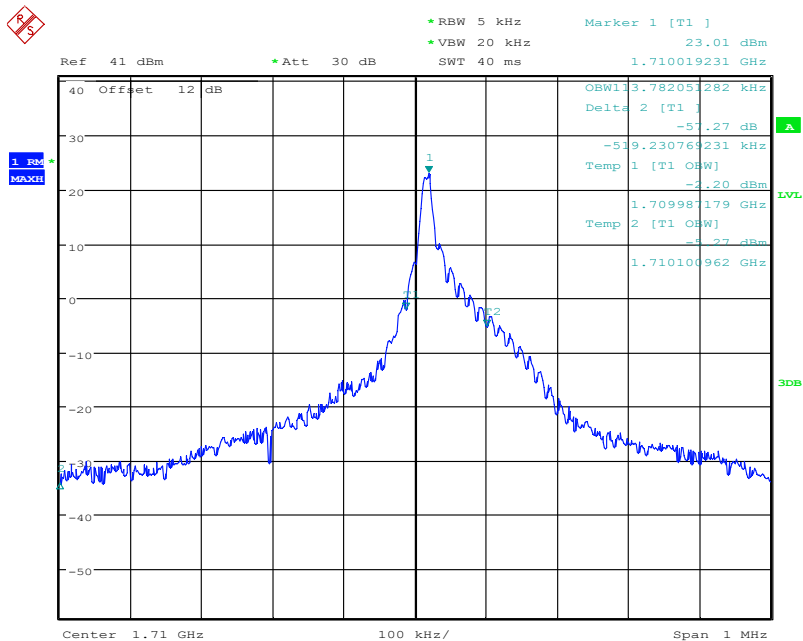
NB-IoT Guard-band band 66 131972 QPSK(99%)
