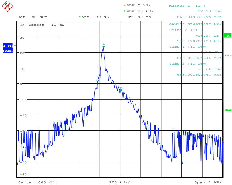
NB-IoT In-band band 71 133122 QPSK(99%)
