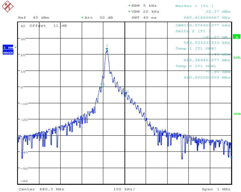
NB-IoT In-band band 71 133297 QPSK(99%)
