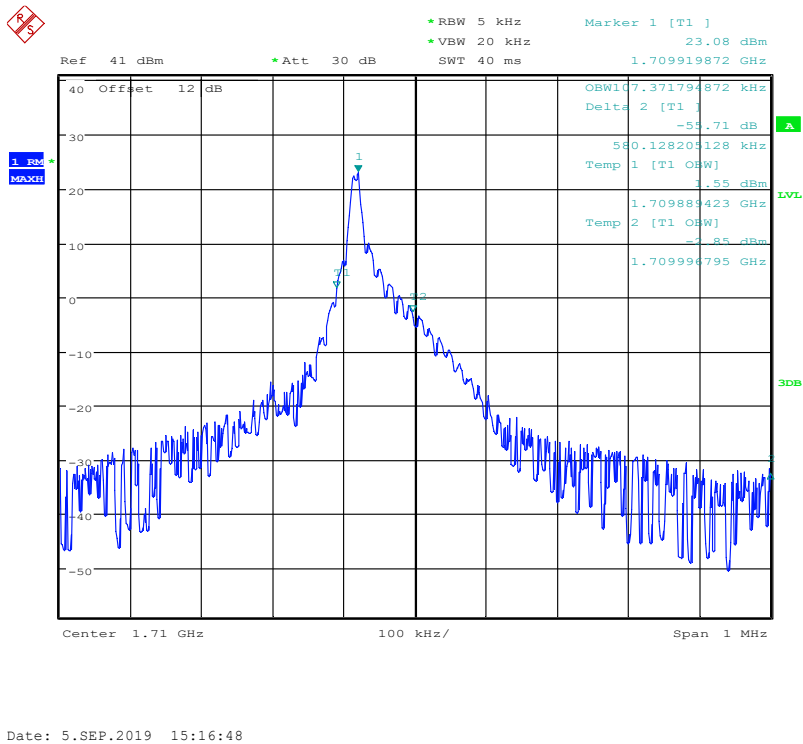
NB-IoT standalone band 66 131972 BPSK(99%)
