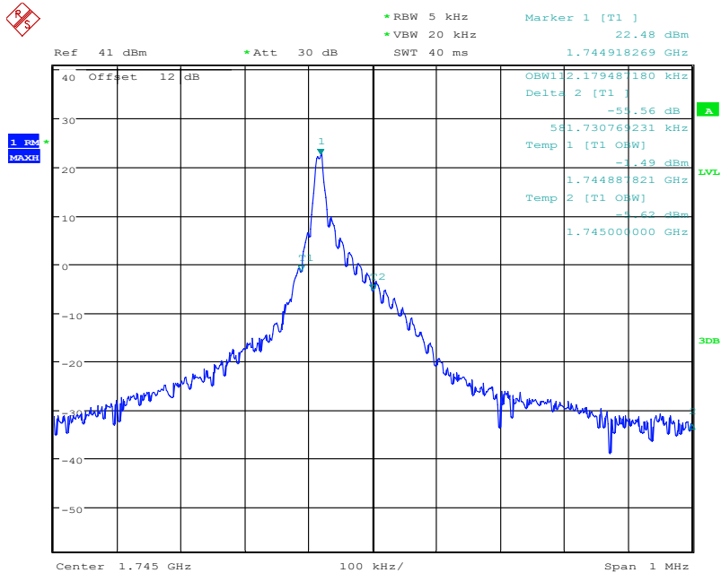
NB-IoT In-band band 66 132322 QPSK(99%)
