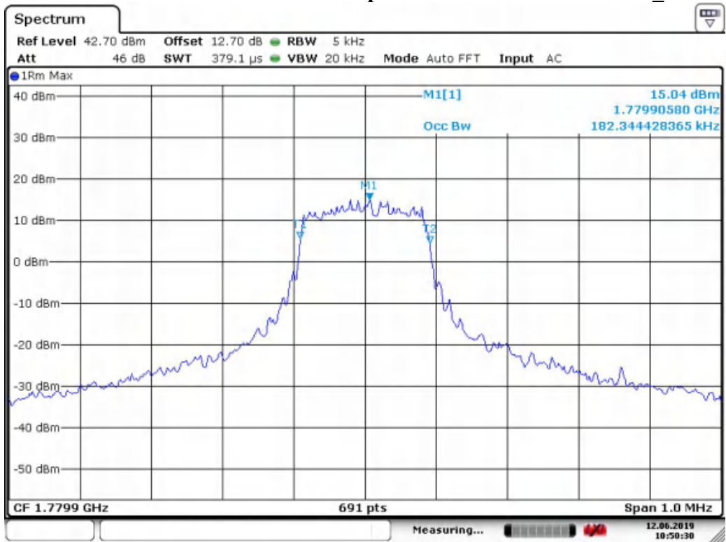
NB-IoT In-band band 66 132671 QPSK(99%)
