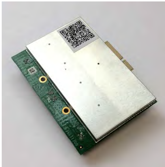
Figure 6 – Top View of the 802.11ac WiFi Radio Module - Samtec IP5 connectors
