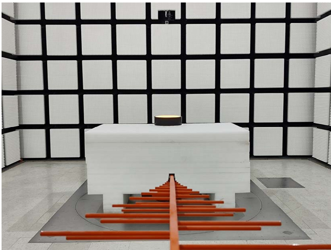
Radiated Emission Below 1GHz Rear View- Without Dimmer
