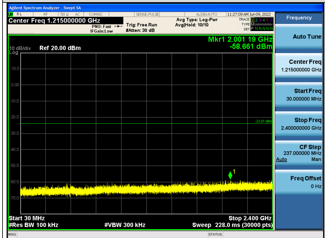
Test Graph LE1M ANT1 2480 1Mbps Lower Band Emissions
