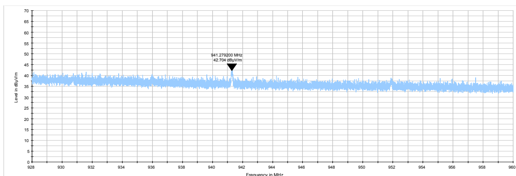
Plot 7.6.9 Radiated emission measurements from 928 to 960 MHz at the mid carrier frequency
