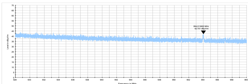
Plot 7.6.10 Radiated emission measurements from 928 to 960 MHz at the high carrier frequency
