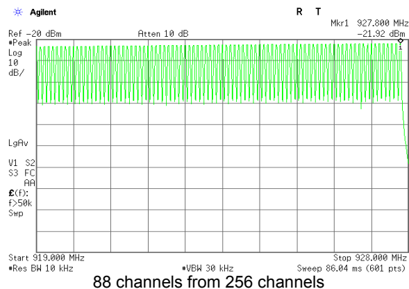
Plot 7.3.2 Number of hopping frequencies GFSK
