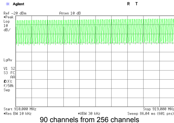
Plot 7.3.2 Number of hopping frequencies 2FSK
