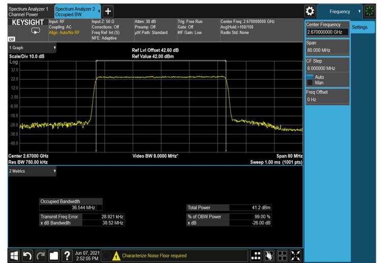
Figure 160: output 64QAM 40MHz B.W.; 2670.0MHz, 60kHz
