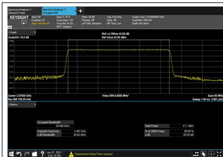
Figure 173: output 256QAM 40MHz B.W.; 2670.0MHz, 15kHz
