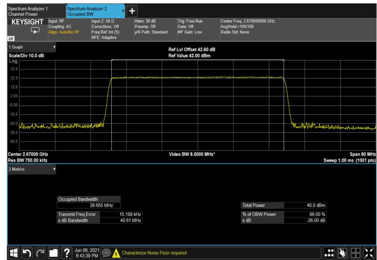
Figure 158: output 64QAM 40MHz B.W.; 2670.0MHz, 15kHz
