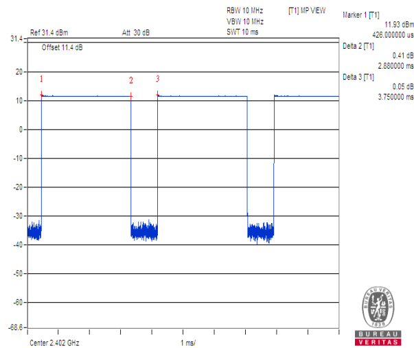
Time-domain plot for Bluetooth transmission signal
