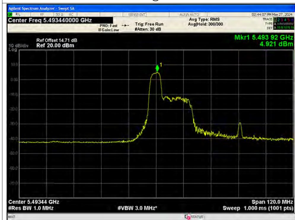
PSD NVNT ax80 52@37 5530MHz Ant1
