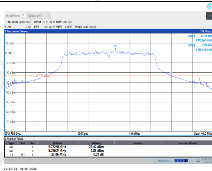
11N20MIMO Ant2 5785
