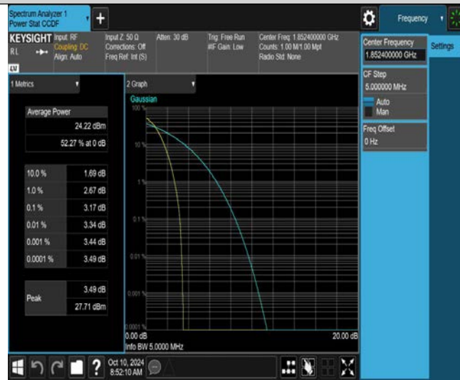
Band2-9262-2
