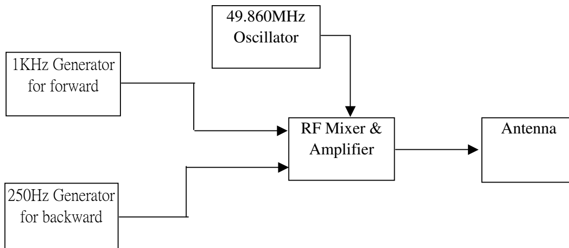
Wiggie RC Car 49.860MHz Tx Block Diagram
