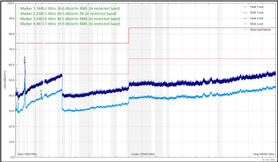
Figure 45 - 2437 MHz (CH6), HT20, Core 0 and 5204 MHz, HDR8, ePA, Core 1, 1 GHz to 40 GHz, Vertical
