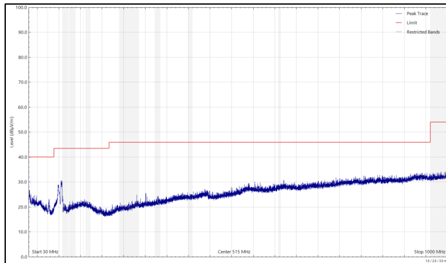
Figure 56 - 2437 MHz (CH6), HT20, Core 1 and 5788 MHz, HDR4, ePA, Core 0, 30 MHz to 1 GHz, Vertical (Peak)
