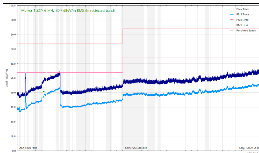
Figure 55 - 2437 MHz (CH6), HT20, Core 1 and 5788 MHz, HDR4, ePA, Core 0, 1 GHz to 40 GHz, Horizontal
