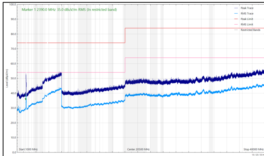
Figure 51 - 2437 MHz (CH6), HT20, Core 0 and 5788 MHz, HDR4, ePA, Core 1, 1 GHz to 40 GHz, Horizontal
