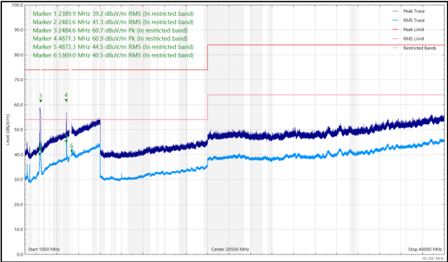
Figure 49 - 2437 MHz (CH6), HT20, Core 1 and 5204 MHz, HDR8, ePA, Core 0, 1 GHz to 40 GHz, Vertical
