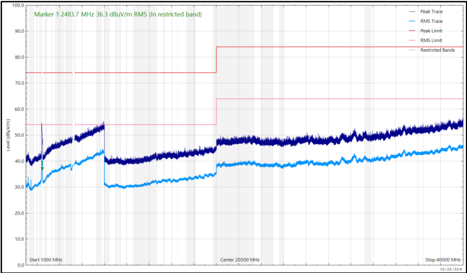
Figure 43 - 2437 MHz (CH6), HT20, Core 0 and 5204 MHz, HDR8, ePA, Core 1, 1 GHz to 40 GHz, Horizontal
