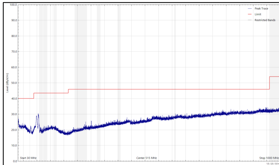
Figure 52 - 2437 MHz (CH6), HT20, Core 0 and 5788 MHz, HDR4, ePA, Core 1, 30 MHz to 1 GHz, Vertical (Peak)
