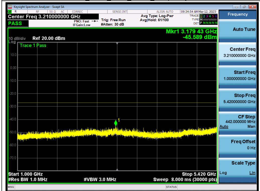
802.11n40_ANT1_5510_MCS0_Frequency Band 2
