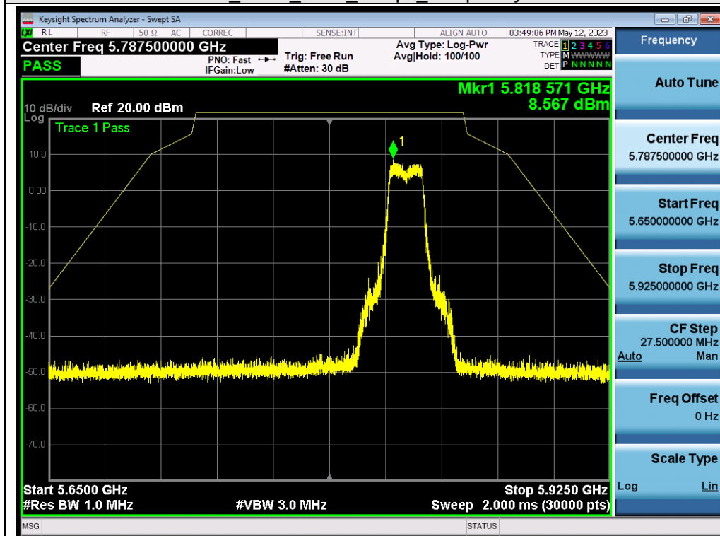
802.11a ANT1 5825 6Mbps Frequency Band3
