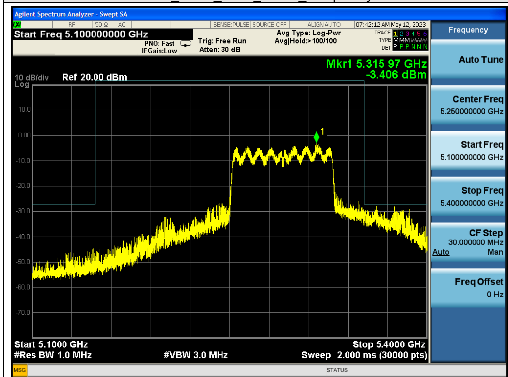
802.11ac80 ANT1_5290_MCS0 Frequency Band 3
