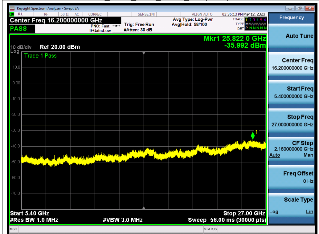
802.11n40_ANT1_5190_MCS0_Frequency Band 4
