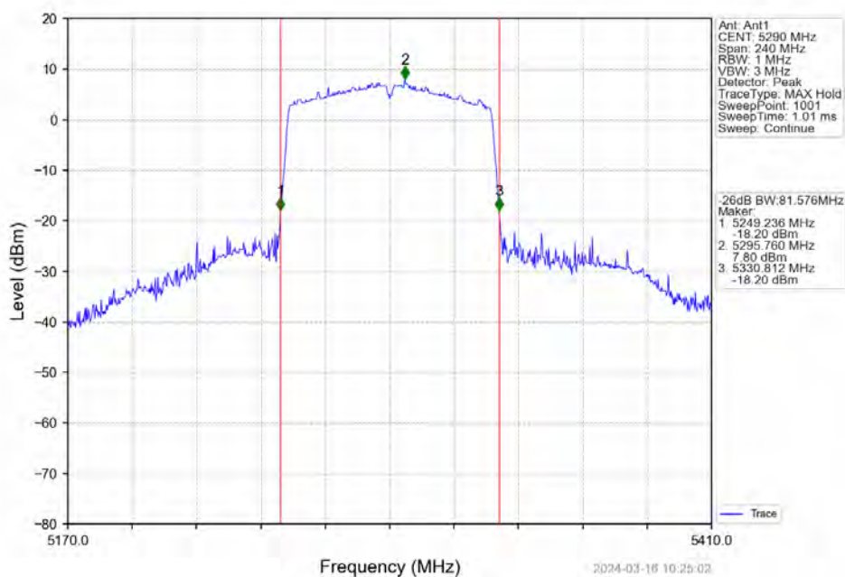
802.11ac(VHT80)_MCH_5290MHz_Ant7_NTNV
