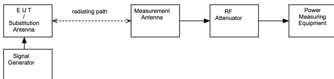
Figure vii Test Setup
