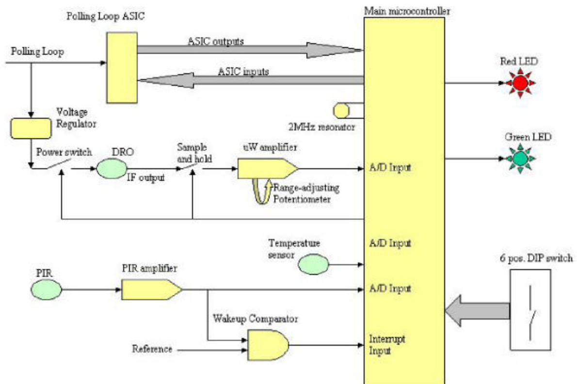
Quest2260SN Block Diagram
