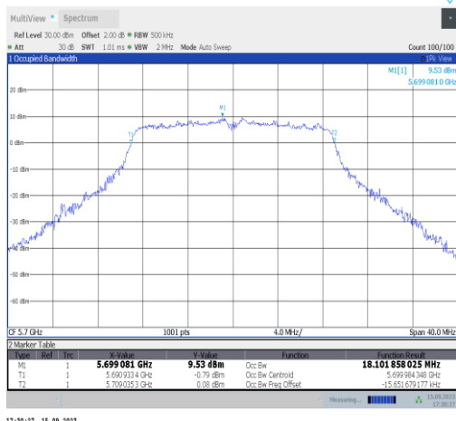
11n20SISO-Ant1-5700
