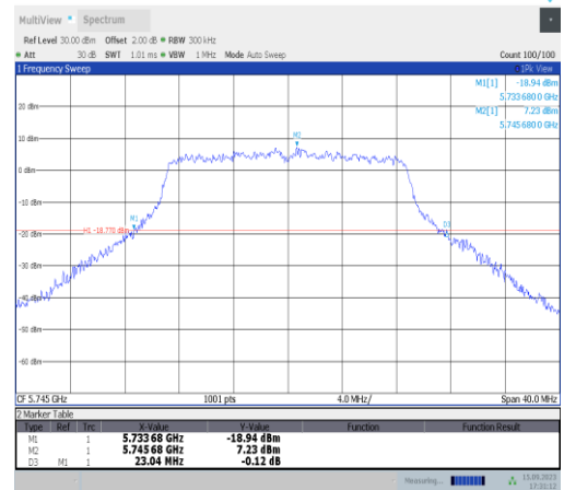
11n20SISO-Ant1-5745
