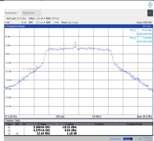
11n20SISO-Ant1-5580
