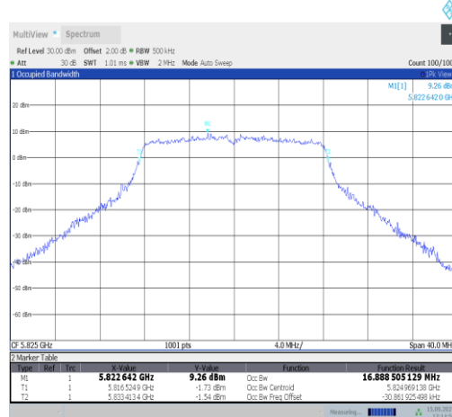
11a-Ant1-5825
