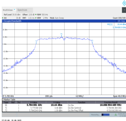
11n20SISO-Ant1-5785
