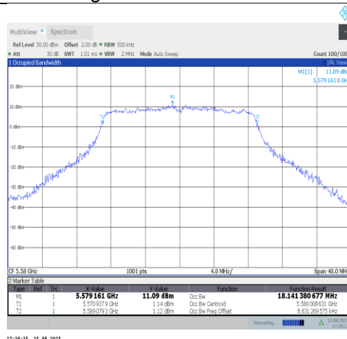
11n20SISO-Ant1-5580
