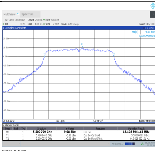
11n20SISO-Ant1-5500
