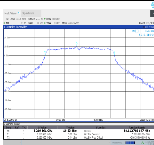
11n20SISO-Ant1-5220
