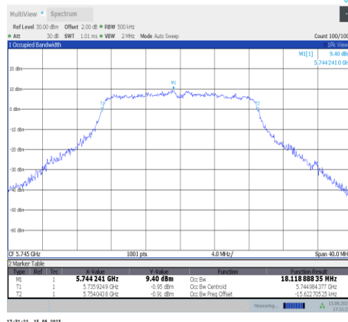
11n20SISO-Ant1-5745
