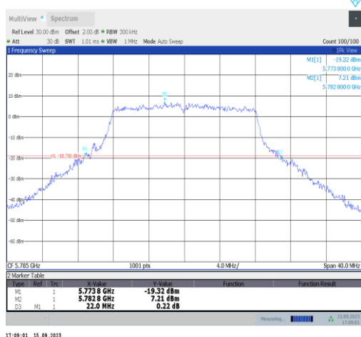
11a-Ant1-5785
