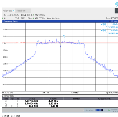
11a-Ant1-5745-PASS
