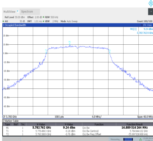
11a-Ant1-5785
