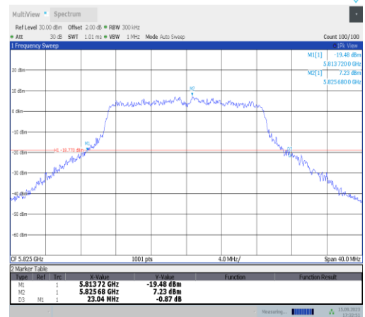
11n20SISO-Ant1-5825
