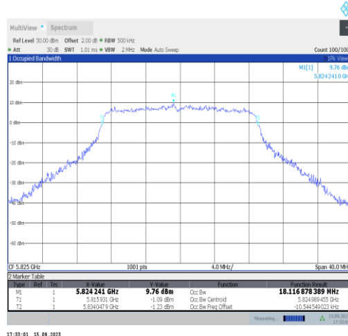
11n20SISO-Ant1-5825
