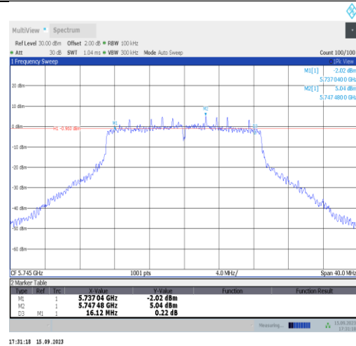
11n20SISO-Ant1-5745-PASS
