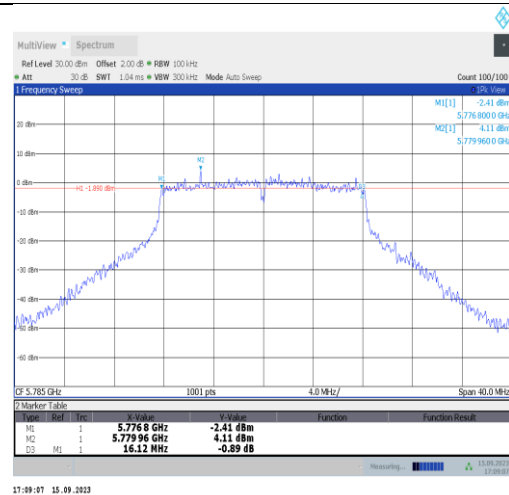
11a-Ant1-5785-PASS
