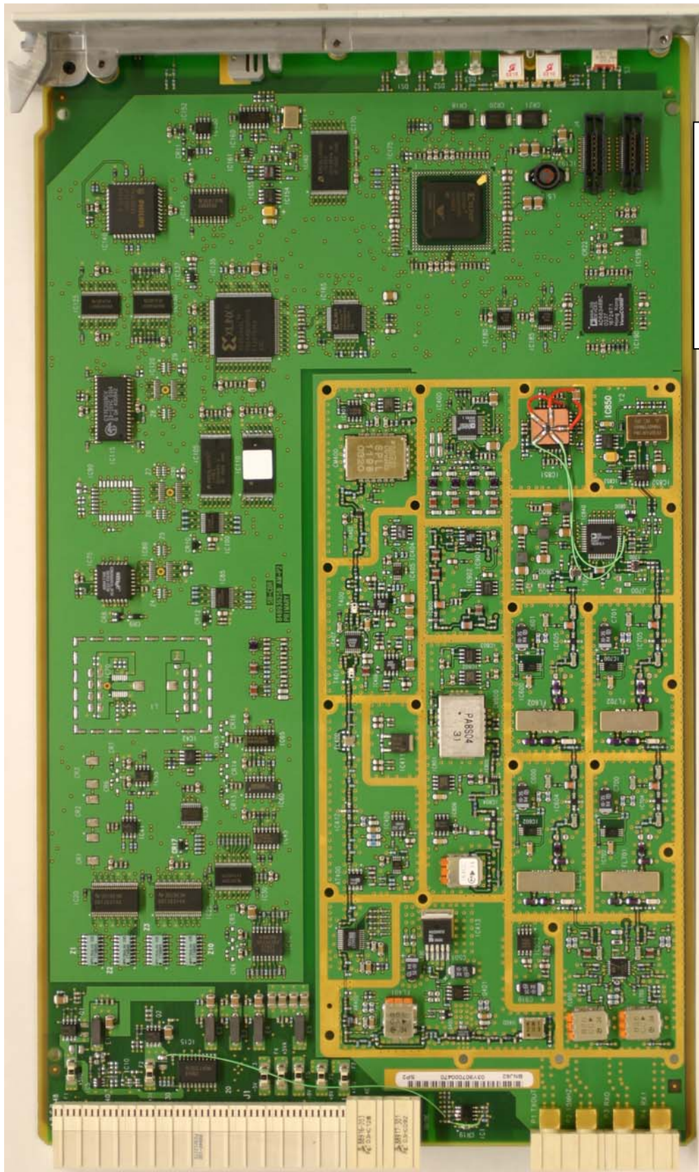
AS5CMP-46 SBCBR Transceiver Circuit Board Component Side View With Shielding Cover Removed
