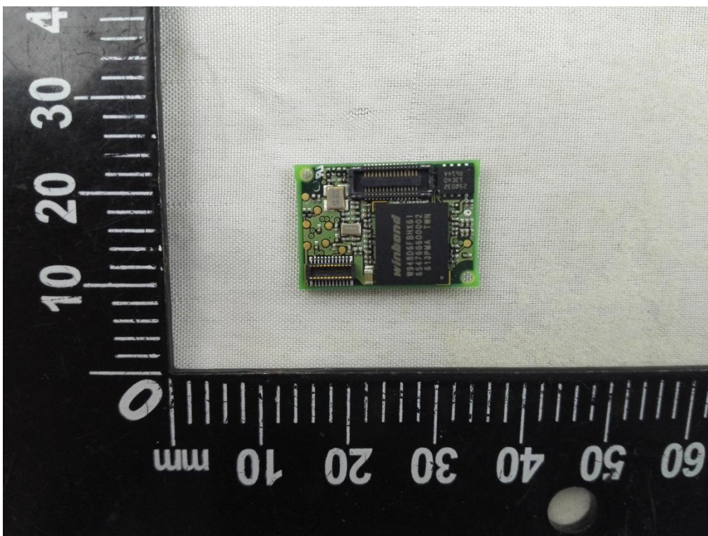
MAIN BOARD 5 TOP VIEW
