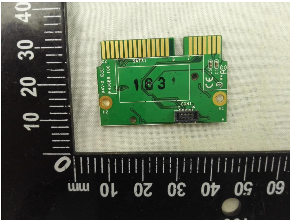
MAIN BOARD 9 TOP VIEW
