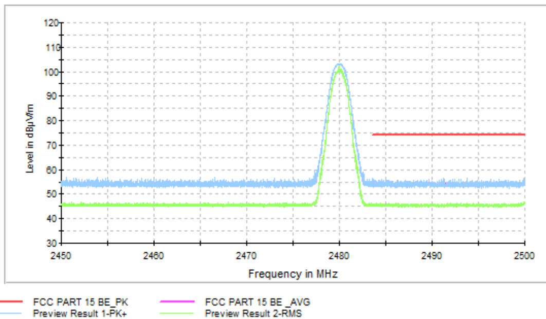
Fig.16. Frequency Band Edges: \pi/4 DQPSK, Channel 78, Hopping Off, 2.45 GHz - 2.50GHz
