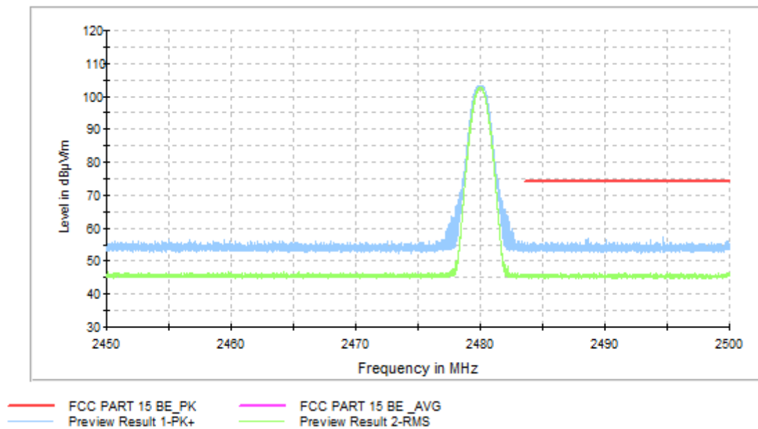
Fig.14. Frequency Band Edges: GFSK, Channel 78, Hopping Off, ch11, 2.45 GHz - 2.50GHz
