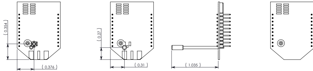
WIRE WHIP
