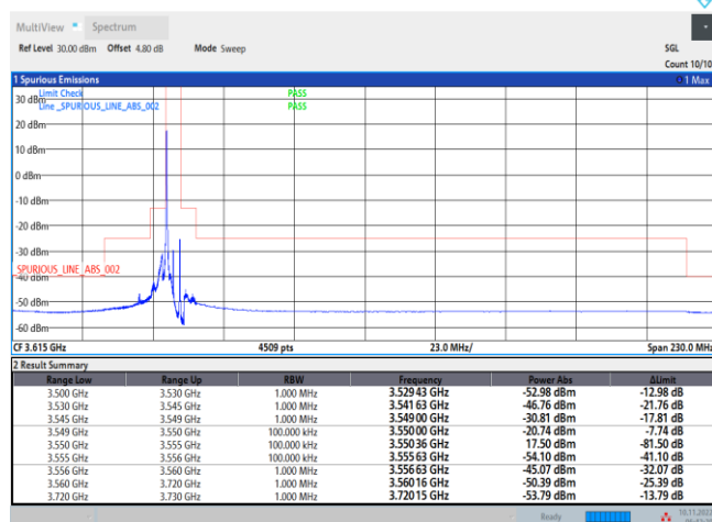
Band48-5MHz-QPSK-55265-25RB#0
