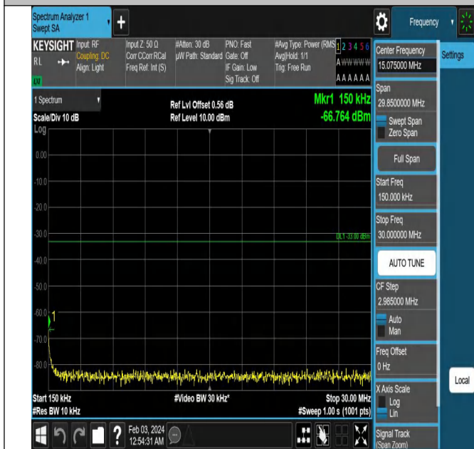
Band2_1.4MHz_QPSK_18900_1RB#0_0.15~30_0.15~30
