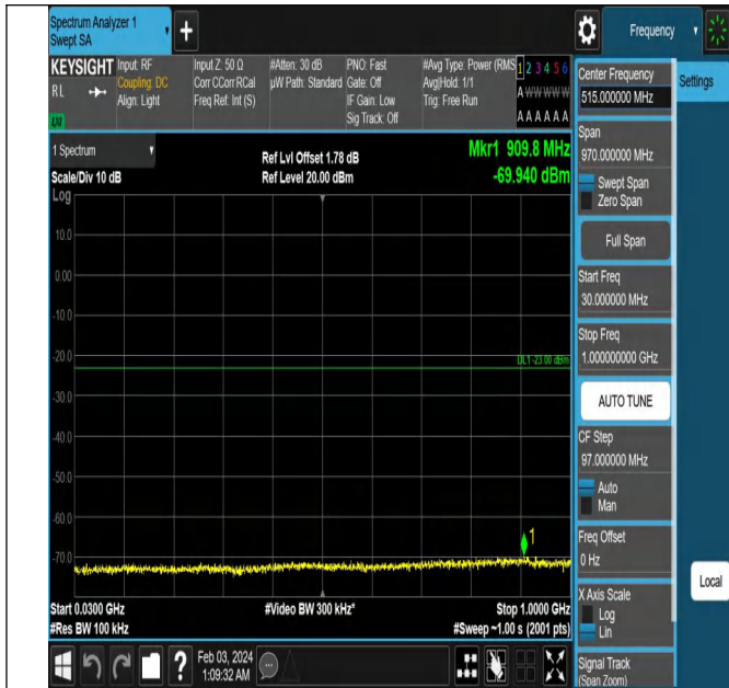
Band2_10MHz_QPSK_18900_1RB#0_30~1000_30~1000
