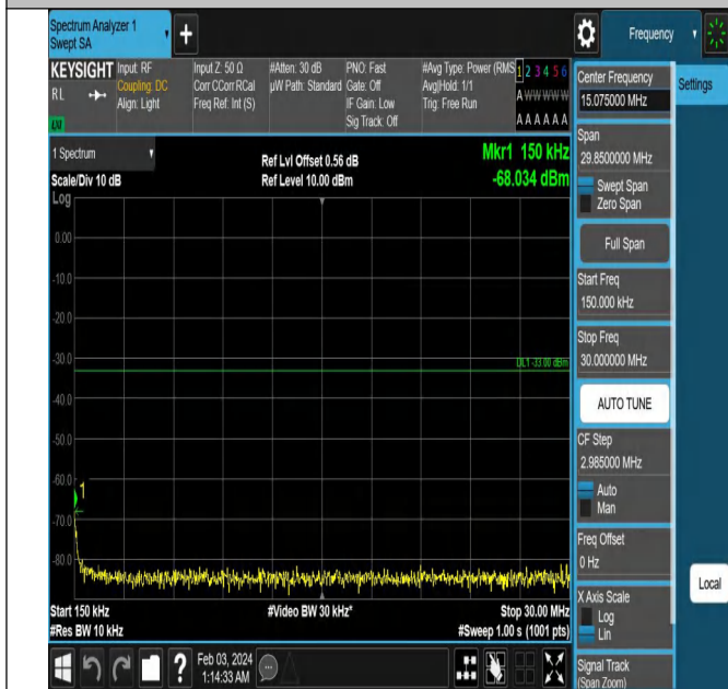
Band2_15MHz_QPSK_18900_1RB#0_0.15~30_0.15~30
