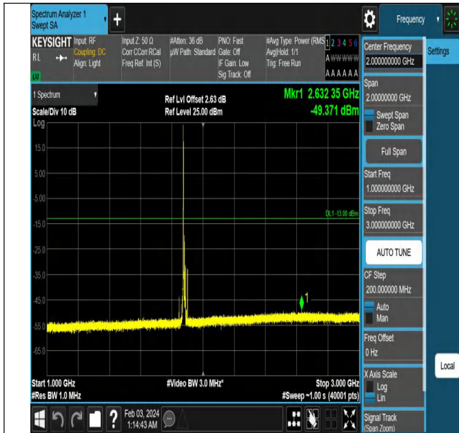
Band2_15MHz_QPSK_18900_1RB#0_1000~3000_1000~300
