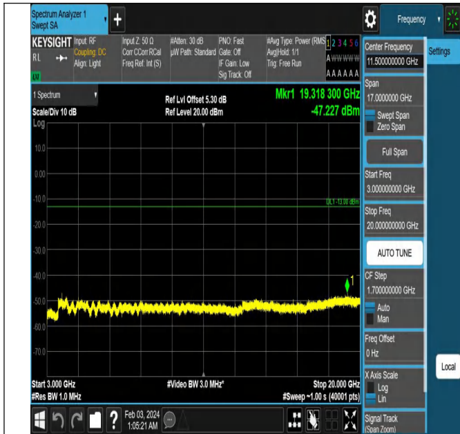
Band2_5MHz_QPSK_19175_1RB#0_3000~20000_3000~200
