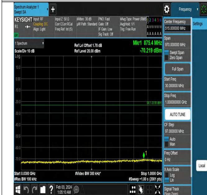
Band2_5MHz_QPSK_19175_1RB#0_30~1000_30~1000
