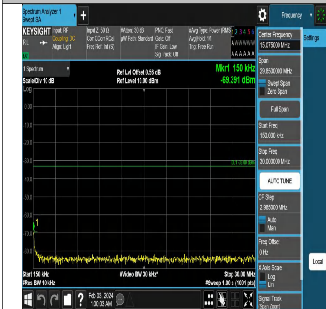
Band2_3MHz_QPSK_19185_1RB#0_0.15~30_0.15~30
