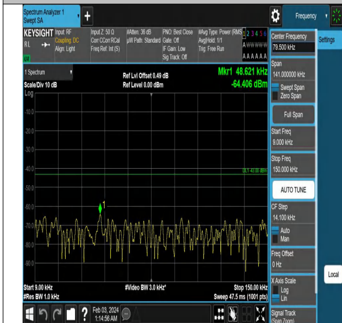
Band2_15MHz_QPSK_19125_1RB#0_0.009~0.15_0.009~0.1
