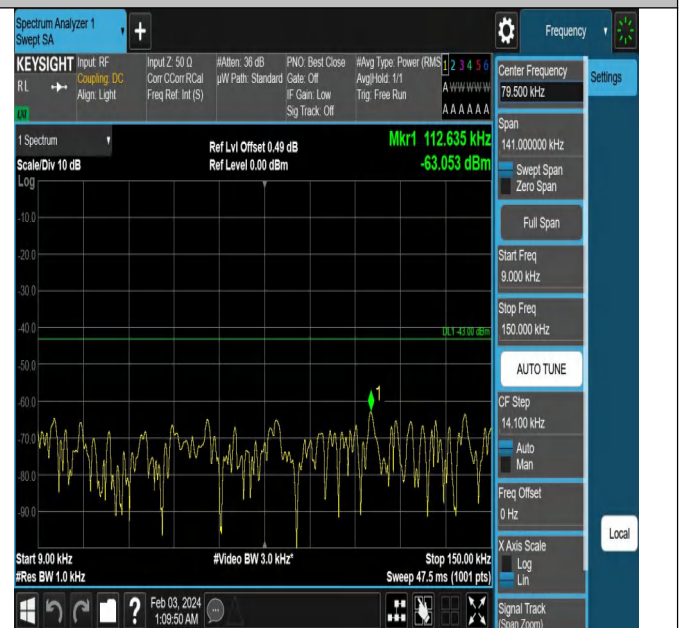
Band2_10MHz_QPSK_19150_1RB#0_0.009~0.15_0.009~0.1 5
