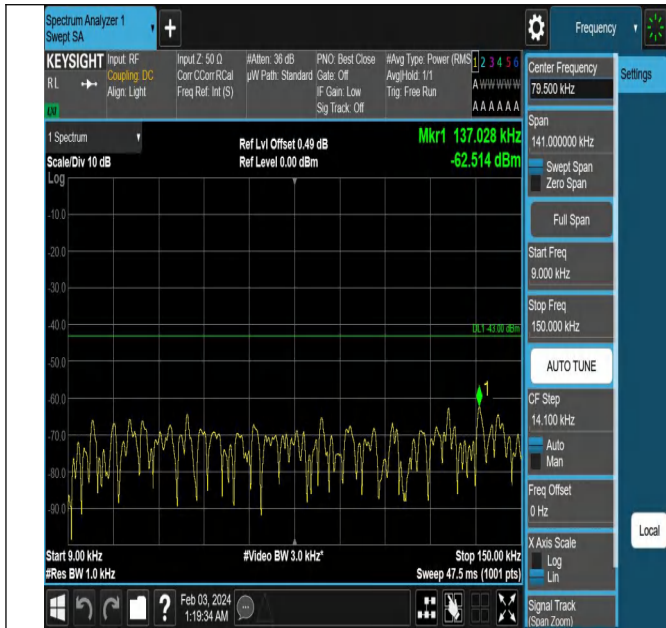
Band2_20MHz_QPSK_18900_1RB#0_0.009~0.15_0.009~0.1
