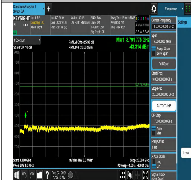
Band2_15MHz_QPSK_19125_1RB#0_3000~20000_3000~20 000
