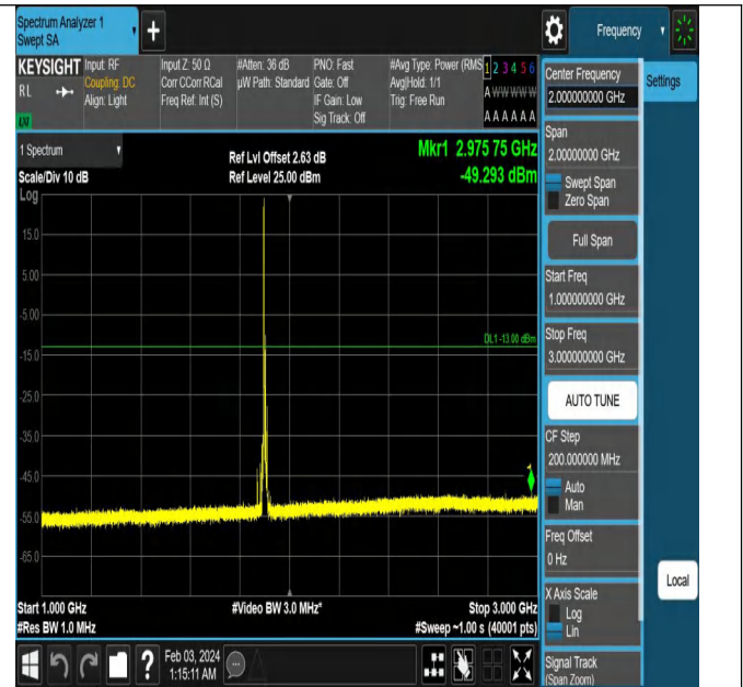
Band2_15MHz_QPSK_19125_1RB#0_1000~3000_1000~300 0
