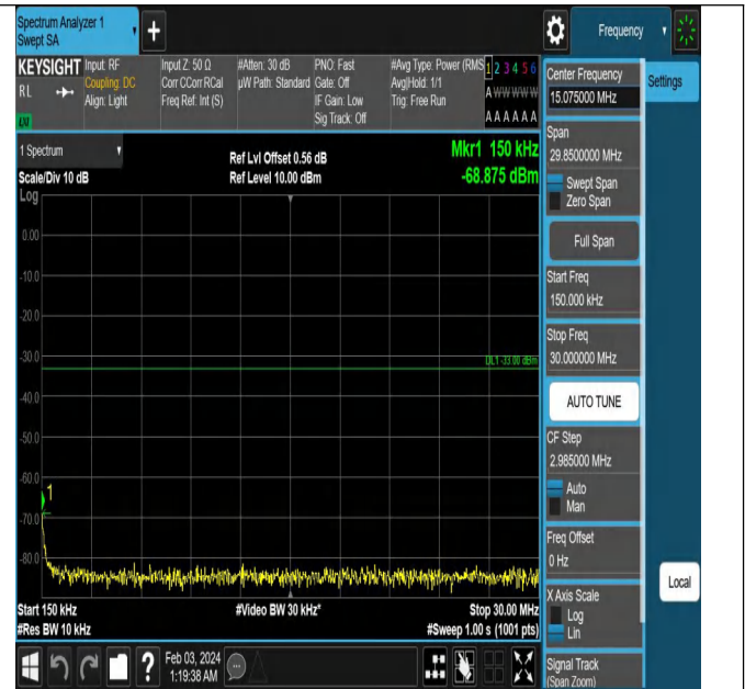
Band2_20MHz_QPSK_18900_1RB#0_0.15~30_0.15~30
