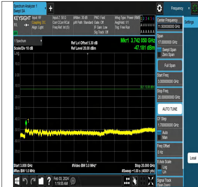
Band2_20MHz_QPSK_18900_1RB#0_3000~20000_3000~20000
