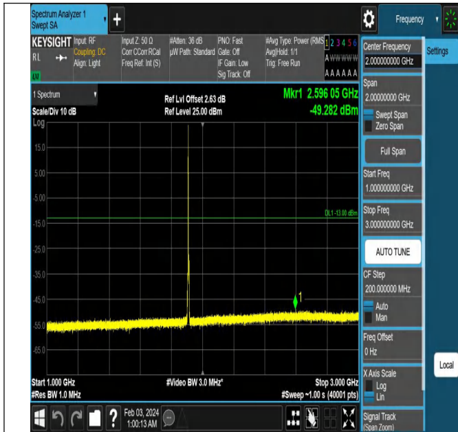
Band2_3MHz_QPSK_19185_1RB#0_1000~3000_1000~3000
