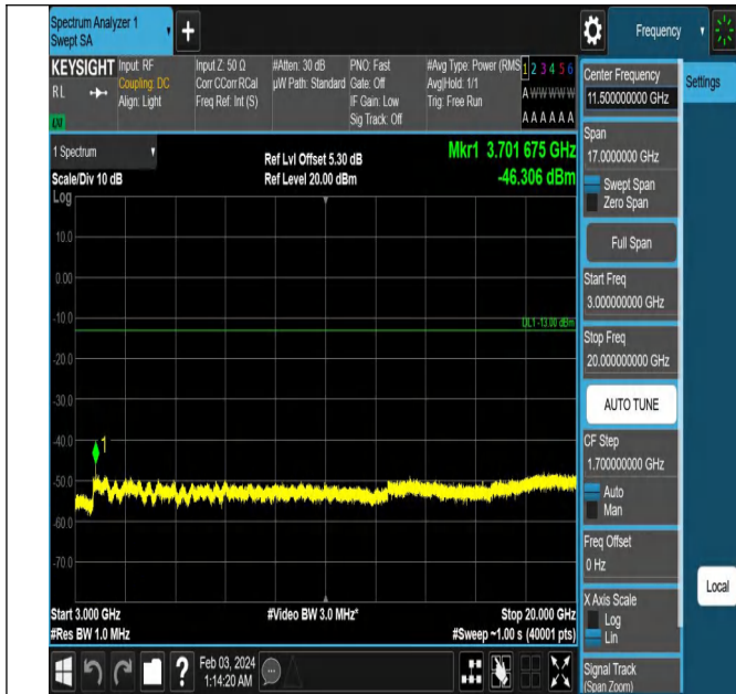
Band2_15MHz_QPSK_18675_1RB#0_3000~20000_3000~20000
