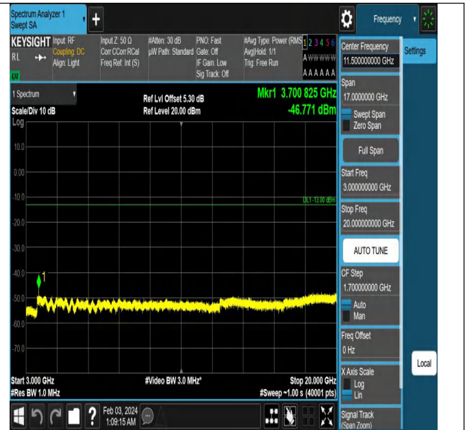
Band2_10MHz_QPSK_18650_1RB#0_3000~20000_3000~20
