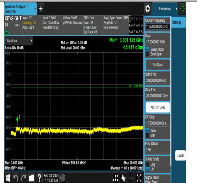
Band2_10MHz_QPSK_19150_1RB#0_3000~20000_3000~20
