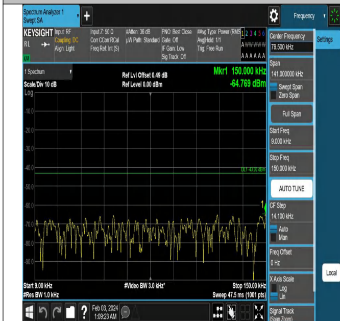
Band2_10MHz_QPSK_18900_1RB#0_0.009~0.15_0.009~0.1
