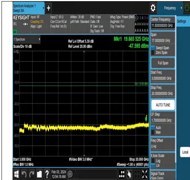
Band2_1.4MHz_QPSK_18607_1RB#0_3000~20000_3000~20000
