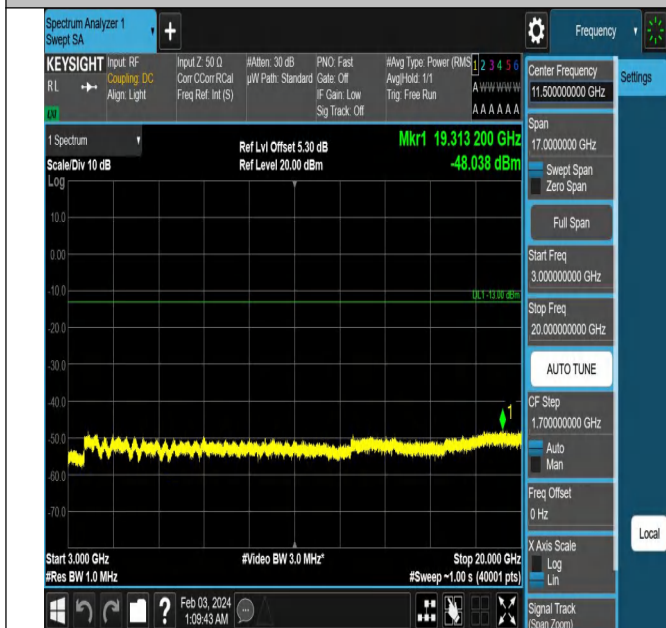
Band2_10MHz_QPSK_18900_1RB#0_3000~20000_3000~20 000
