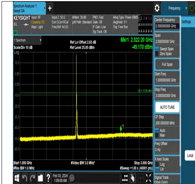
Band2_10MHz_QPSK_18650_1RB#0_1000~3000_1000~300
