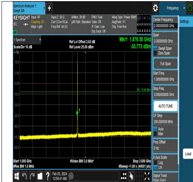
Band2_1.4MHz_QPSK_18900_1RB#0_1000~3000_1000~300
