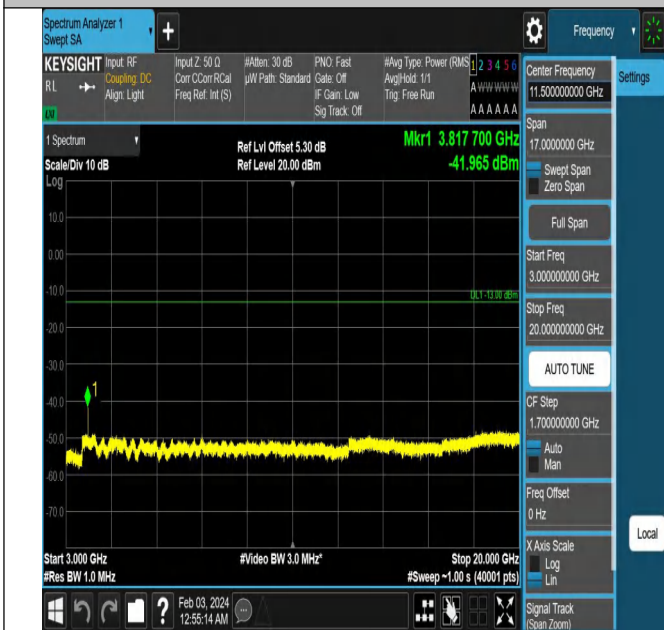
Band2_1.4MHz_QPSK_19193_1RB#0_3000~20000_3000~20000
