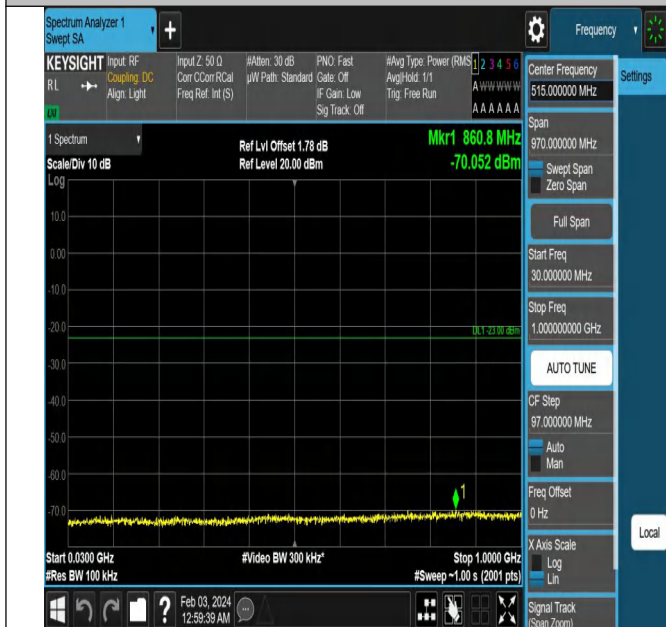
Band2_3MHz_QPSK_18900_1RB#0_30~1000_30~1000
