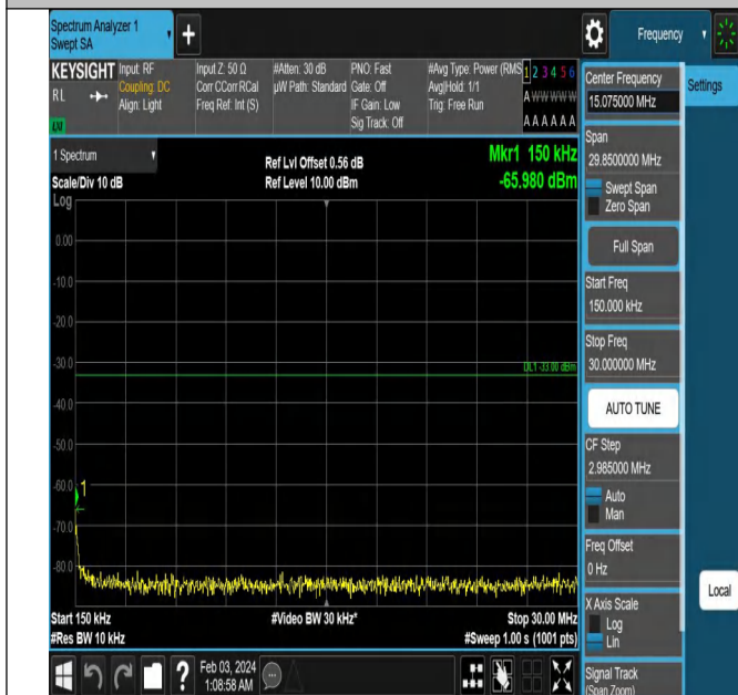
Band2_10MHz_QPSK_18650_1RB#0_0.15~30_0.15~30
