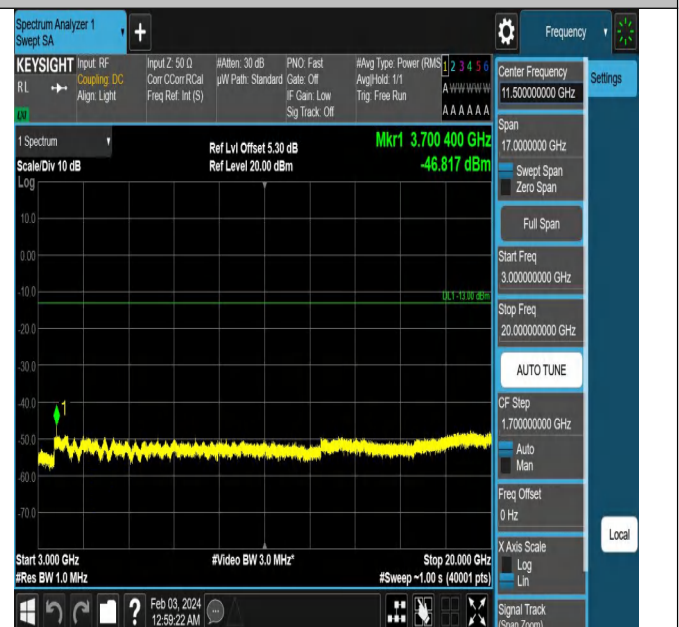
Band2_3MHz_QPSK_18615_1RB#0_3000~20000_3000~200
