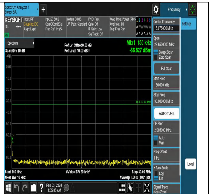
Band2_5MHz_QPSK_19175_1RB#0_0.15~30_0.15~30
