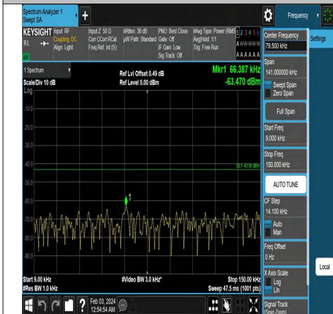
Band2_1.4MHz_QPSK_19193_1RB#0_0.009~0.15_0.009~0.1
