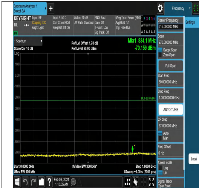
Band2_15MHz_QPSK_19125_1RB#0_30~1000_30~1000
