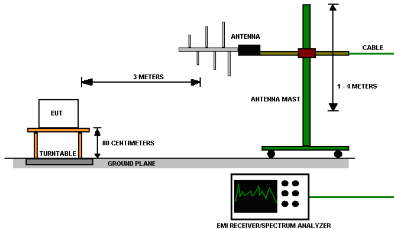
Figure 22 - Radiated Emissions Test Setup
