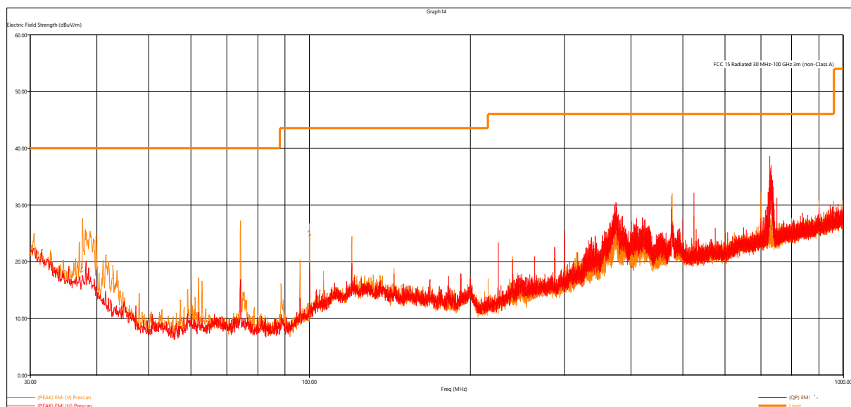
Figure 24 - Radiated Emissions Plot, Mid Channel
