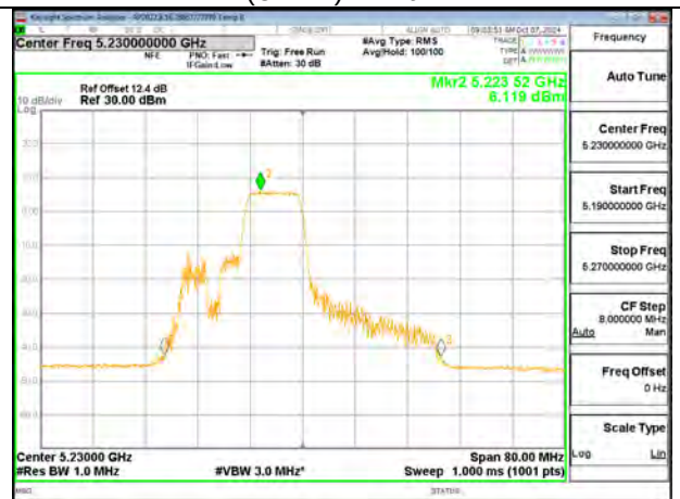
40MHz - High Channel – 106T RU54 (UNII-1) – Ant 2
