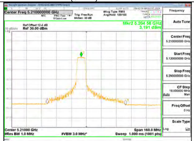
80MHz - Mid Channel – 106T RU56 (UNII-1) – Ant 2
