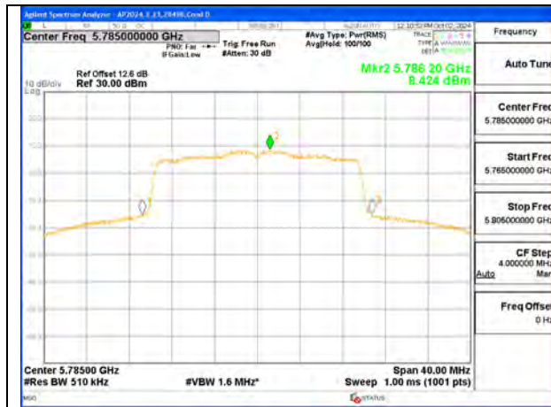
20MHz - Mid Channel – SU (UNII-3) – Ant 2
