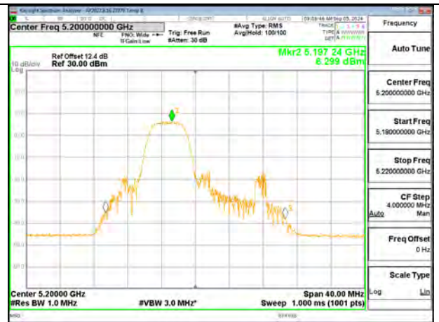
20MHz - Mid Channel – 52T RU38 (UNII-1) – Ant 2
