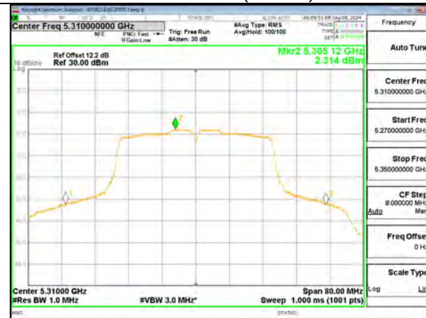
40MHz - High Channel (UNII-2a) – Ant 1
