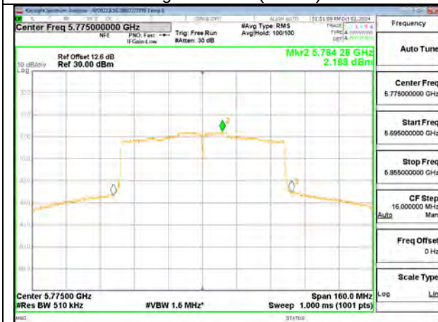
80MHz - Mid Channel (UNII-3) – Ant 2
