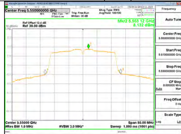
40MHz - Mid Channel (UNII-2c) – Ant 1
