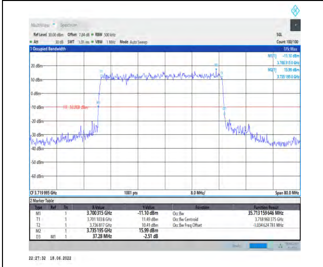
1-N77-3700-3980--30-40-L-1-DFT-QPSK-Outer_Full -100@0-Ant1-35.713-37.280-<40-PASS
