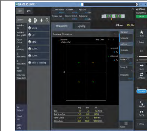
1-N77-3700-3980--30-100-M-1-DFT-PI2BPSK-Outer_Full-270@0-Ant1-see graph-PASS
