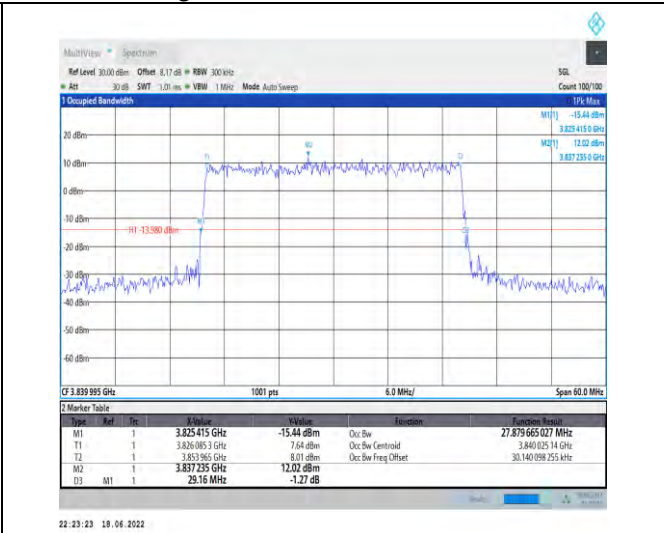
1-N77-3700-3980--30-30-M-6-CP-QPSK-Outer_Full-78@0-Ant1-27.88-29.160-<=30-PASS
