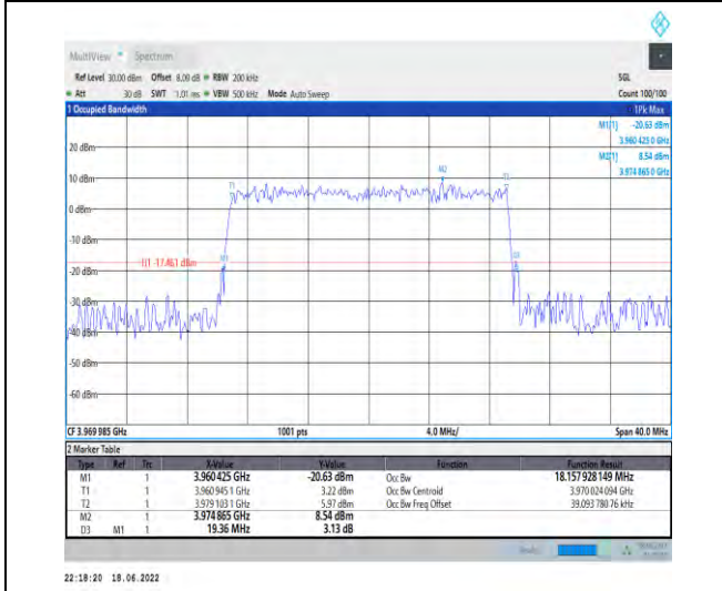
1-N77-3700-3980--30-20-H-9-CP-256QAM-Outer_F ull-51@0-Ant1-18.158-19.360-<=20-PASS
