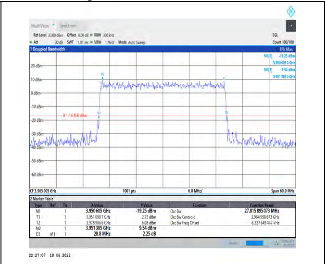
1-N77-3700-3980--30-30-H-9-CP-256QAM-Outer_Fu II-78@0-Ant1-27.816-28.800-<30-PASS
