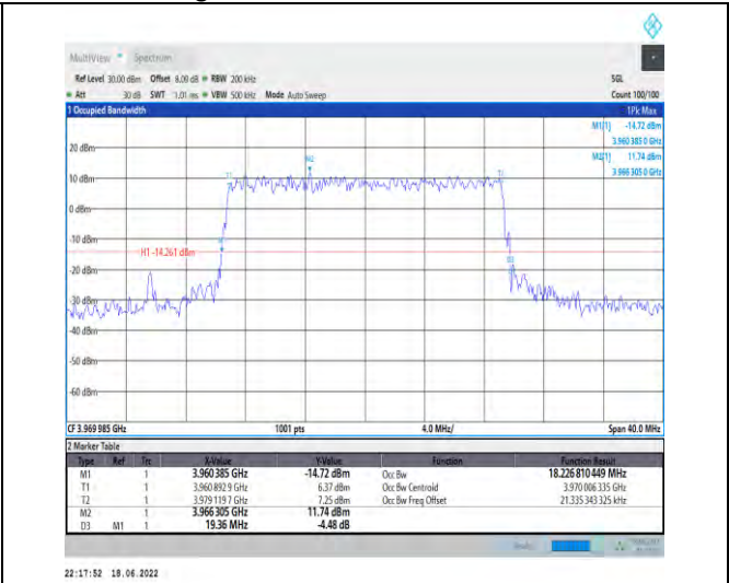
1-N77-3700-3980--30-20-H-8-CP-64QAM-Outer_Full -51@0-Ant1-18.227-19.360-<=20-PASS
