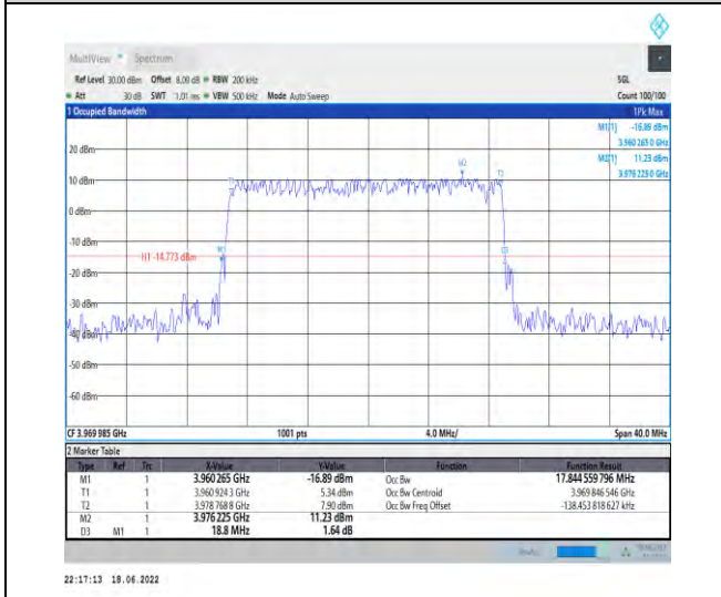
1-N77-3700-3980--30-20-H-5-DFT-256QAM-Outer_Full-50@0-Ant1-17.845-18.800-≤20-PASS
