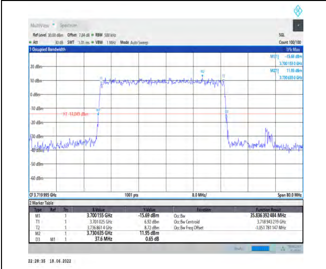
1-N77-3700-3980--30-40-L-5-DFT-256QAM-Outer_F ull-100@0-Ant1-35.836-37.600-<math>\leq 40</math>-PASS
