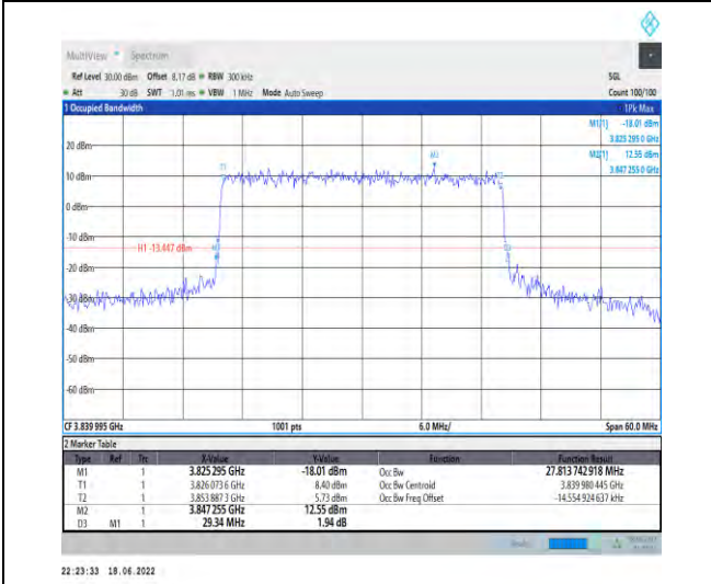
1-N77-3700-3980--30-30-M-7-CP-16QAM-Outer_Ful I-78@0-Ant1-27.814-29.340-<=30-PASS
