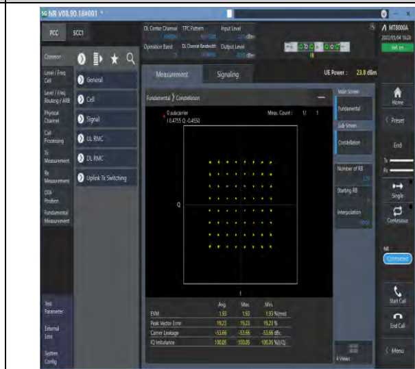
1-N77-3700-3980--30-100-M-4-DFT-64QAM-Outer_Full-270@0-Ant1-see graph-PASS
