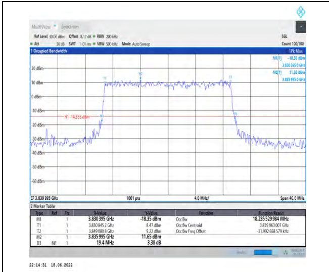
1-N77-3700-3980--30-20-M-8-CP-64QAM-Outer_Ful I-51@0-Ant1-18.236-19.400-<20-PASS
