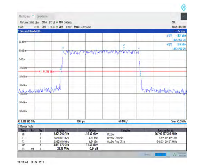
1-N77-3700-3980--30-30-M-5-DFT-256QAM-Outer_Full-75@0-Ant1-26.792-28.260-<=30-PASS
