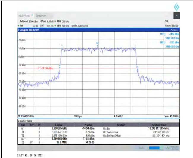
1-N77-3700-3980--30-20-H-7-CP-16QAM-Outer_Full I-51@0-Ant1-18.249-19.200-<=20-PASS
