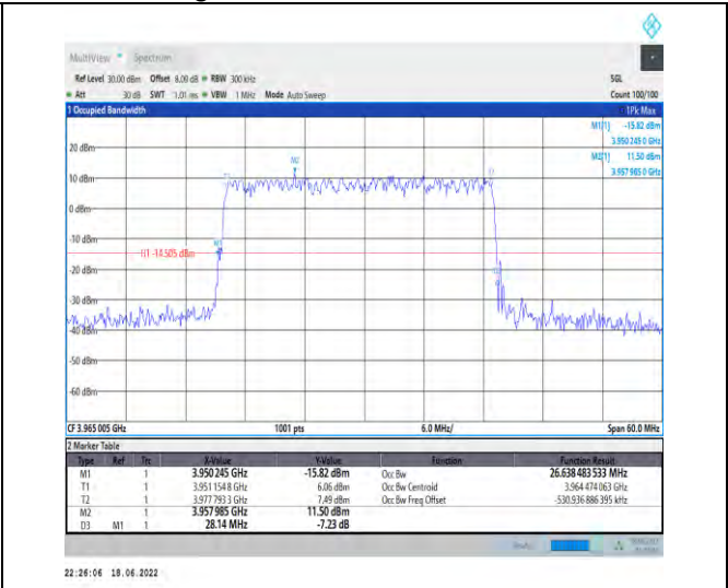
1-N77-3700-3980--30-30-H-5-DFT-256QAM-Outer_Full-75@0-Ant1-26.638-28.140-≤30-PASS
