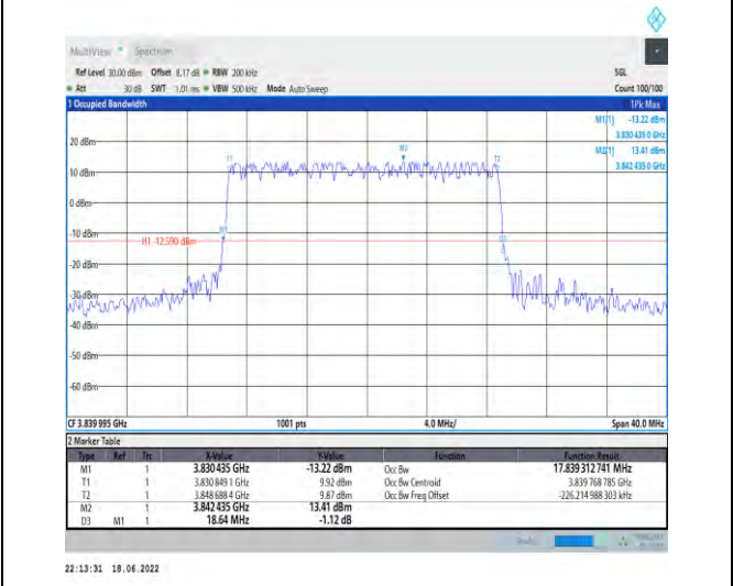
1-N77-3700-3980--30-20-M-3-DFT-16QAM-Outer_Full-50@0-Ant1-17.839-18.640-≤20-PASS
