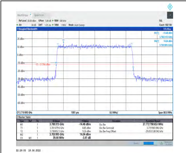
1-N77-3700-3980--30-40-L-7-CP-16QAM-Outer_Full -106@0-Ant1-37.773-39.440-≤40-PASS
