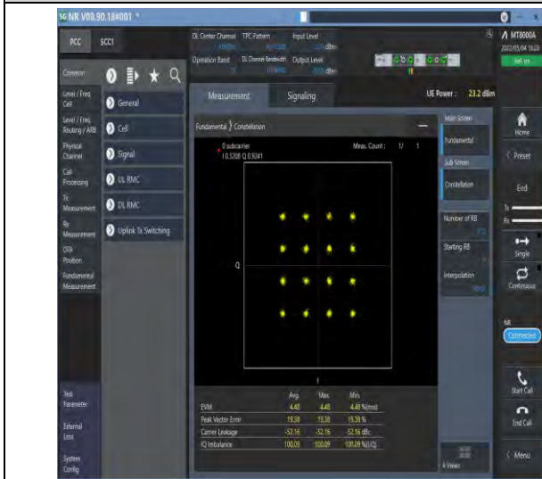
1-N77-3700-3980--30-100-M-7-CP-16QAM-Outer_Fu II-273@0-Ant1-see graph-PASS
