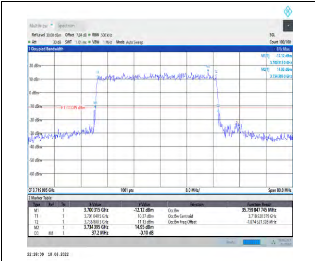
1-N77-3700-3980--30-40-L-3-DFT-16QAM-Outer_Fu ll-100@0-Ant1-35.76-37.200-<math>\leq 40</math>-PASS
