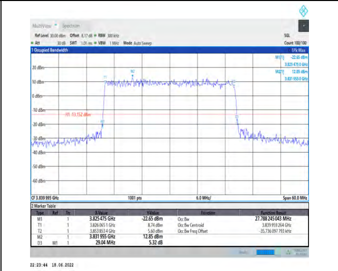
1-N77-3700-3980--30-30-M-8-CP-64QAM-Outer_Full -78@0-Ant1-27.788-29.040-<=30-PASS
