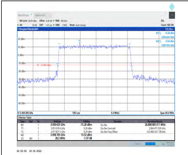
1-N77-3700-3980--30-30-H-4-DFT-64QAM-Outer_Full-75@0-Ant1-26.801-28.200-≤30-PASS
