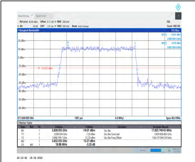
1-N77-3700-3980--30-20-M-4-DFT-64QAM-Outer_Full-50@0-Ant1-17.826-18.880-≤20-PASS
