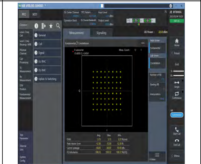
1-N77-3700-3980--30-100-M-8-CP-64QAM-Outer_Fu Full-273@0-Ant1-see graph-PASS
