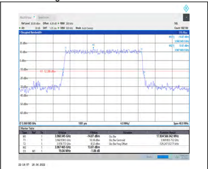
1-N77-3700-3980--30-20-H-4-DFT-64QAM-Outer_Full-50@0-Ant1-17.835-19.040-≤20-PASS
