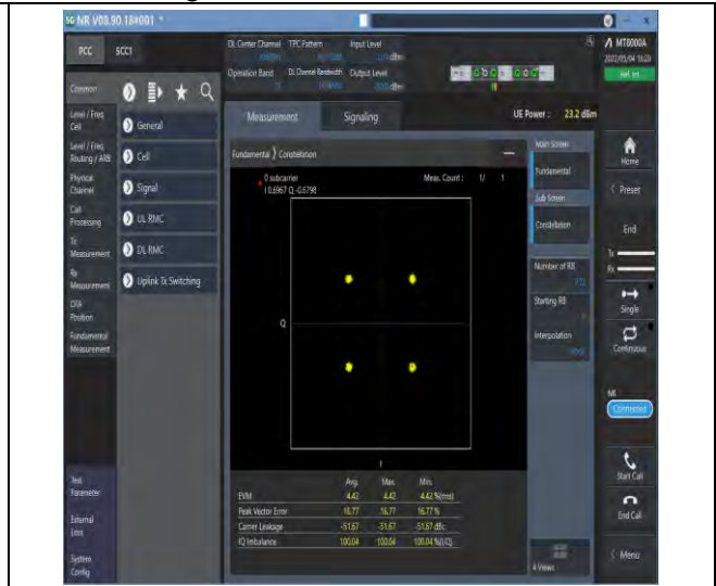
1-N77-3700-3980--30-100-M-6-CP-QPSK-Outer_Fu II-273@0-Ant1-see graph-PASS
