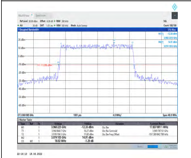
1-N77-3700-3980--30-20-H-1-DFT-QPSK-Outer_Full -50@0-Ant1-17.838-18.920-<20-PASS
