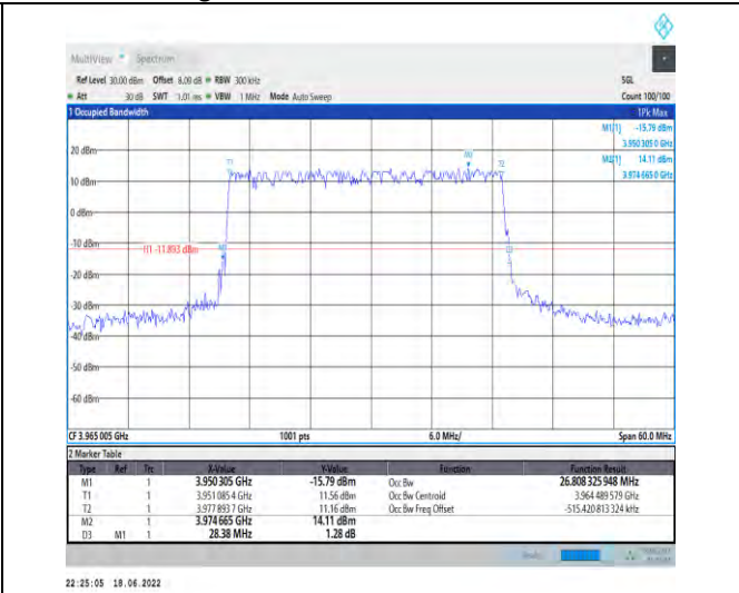
1-N77-3700-3980--30-30-H-1-DFT-QPSK-Outer_Full-75@0-Ant1-26.808-28.380-≤30-PASS
