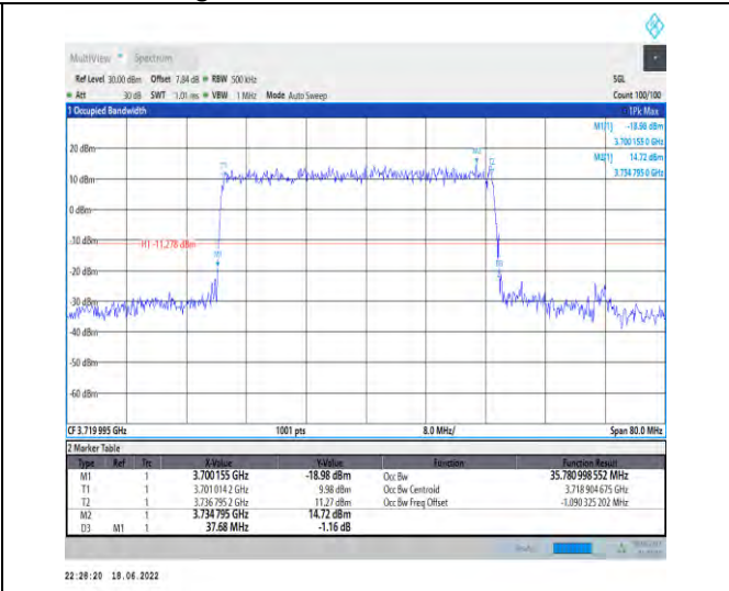
1-N77-3700-3980--30-40-L-4-DFT-64QAM-Outer_Ful l-100@0-Ant1-35.781-37.680-<math>\leq 40</math>-PASS
