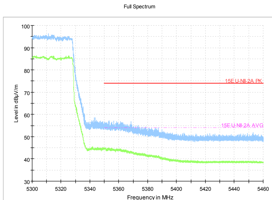
Fig.22 Band Edges (802.11ac-HT80, 5290MHz)
