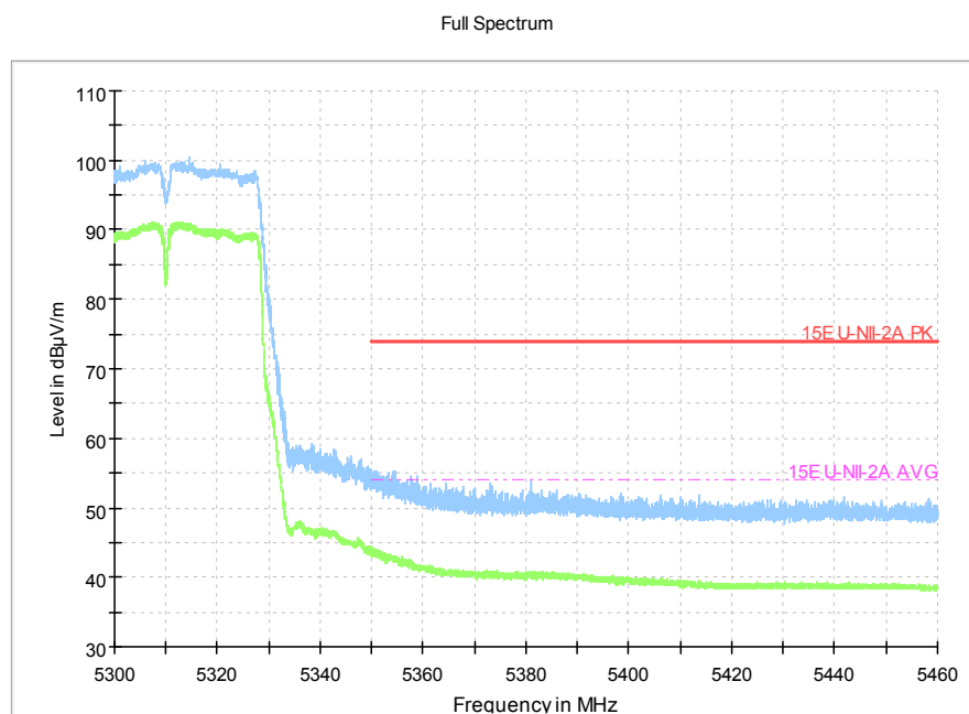
Fig.18 Band Edges (802.11ac-HT40, 5310MHz)
