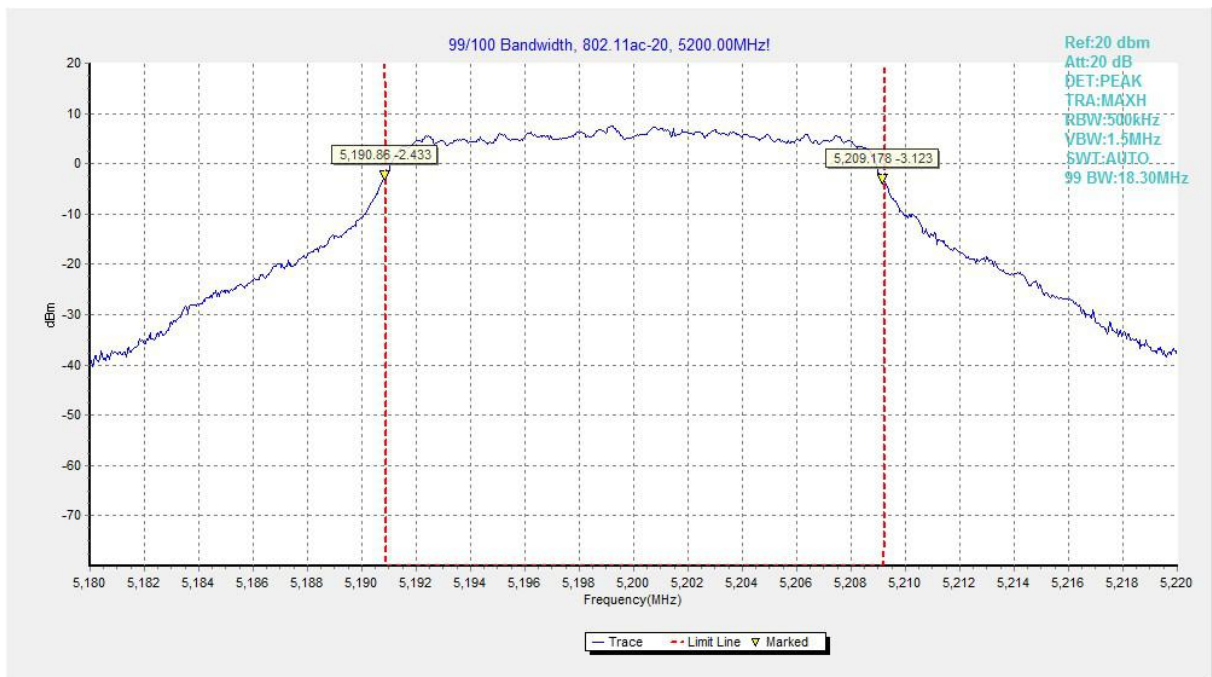
Fig.33 99% Occupied bandwidth (802.11ac-HT20, 5200MHz)
