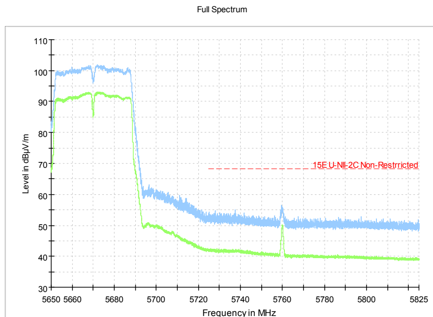
Fig.20 Band Edges (802.11ac-HT40, 5670MHz)
