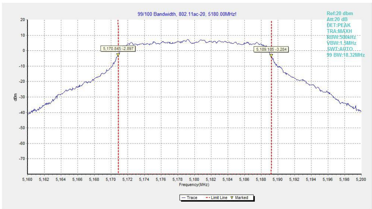
Fig.32 99% Occupied bandwidth (802.11ac-HT20, 5180MHz)
