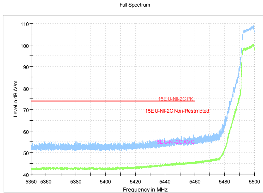
Fig.3 Band Edges (802.11a, 5500MHz)
