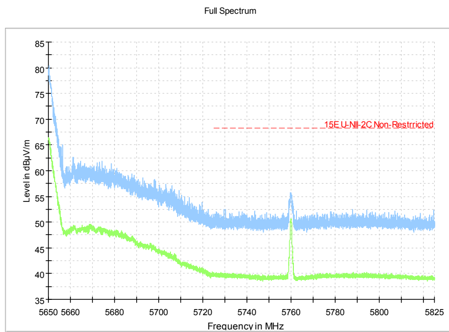
Fig.24 Band Edges (802.11ac-HT80, 5610MHz)
