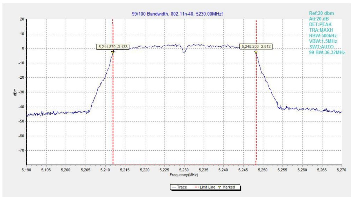
Fig.36 99% Occupied bandwidth (802.11n-HT40, 5230MHz)
