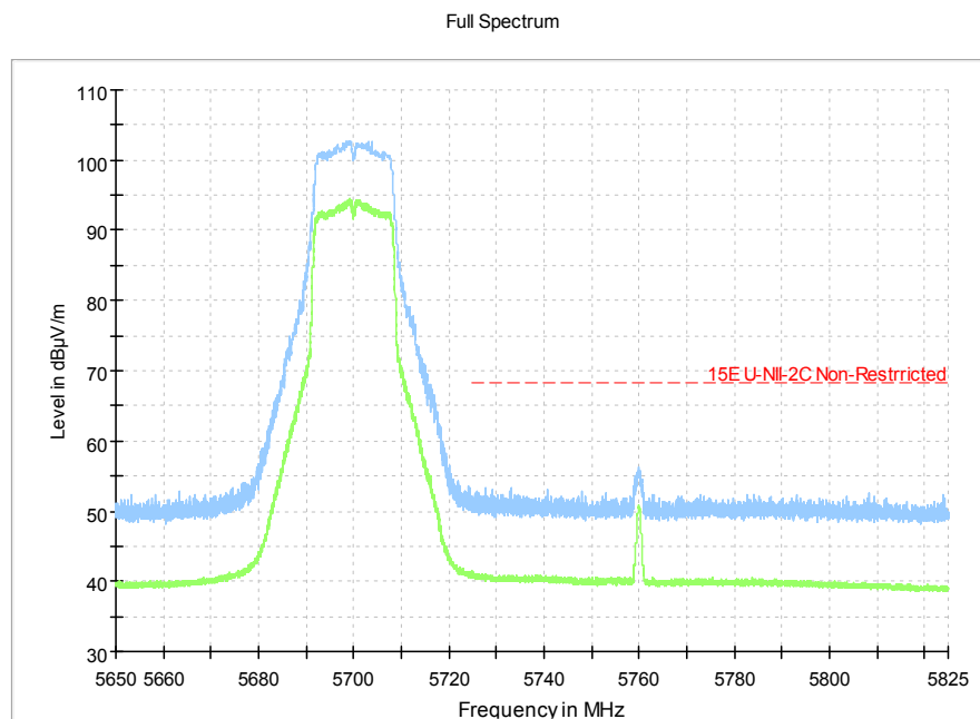
Fig.4 Band Edges (802.11a, 5700MHz)
