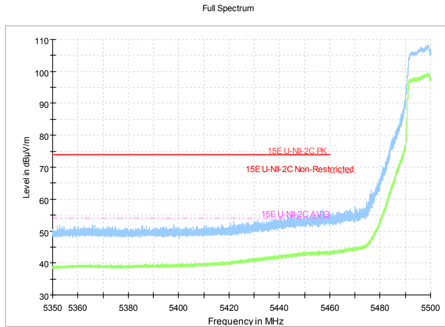
Fig.7 Band Edges (802.11n-HT20, 5500MHz)
