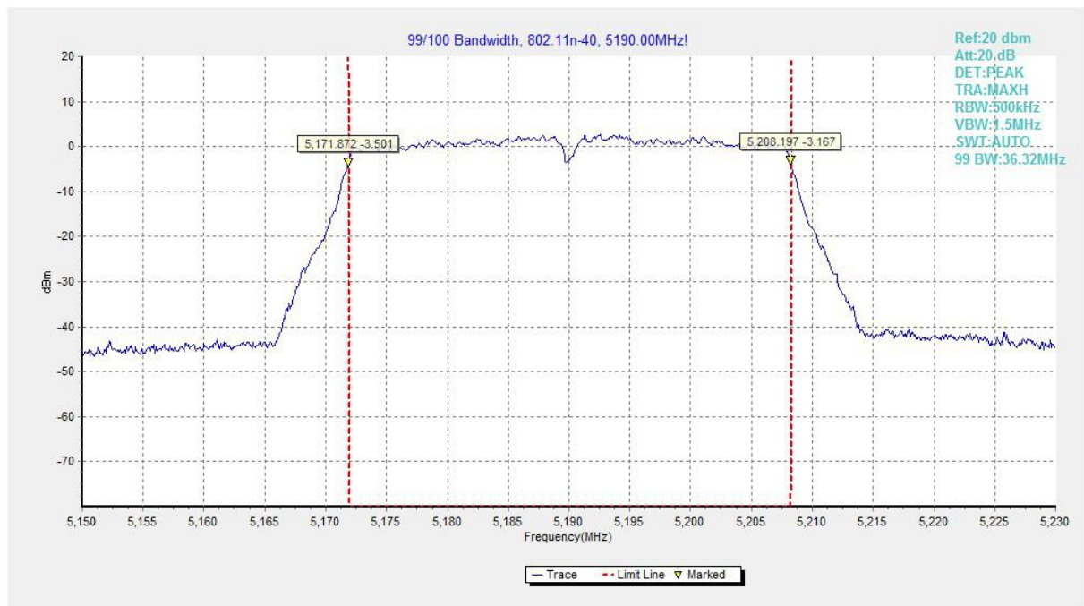
Fig.35 99% Occupied bandwidth (802.11n-HT40, 5190MHz)
