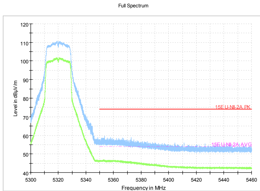
Fig.10 Band Edges (802.11ac-HT20, 5320MHz)
