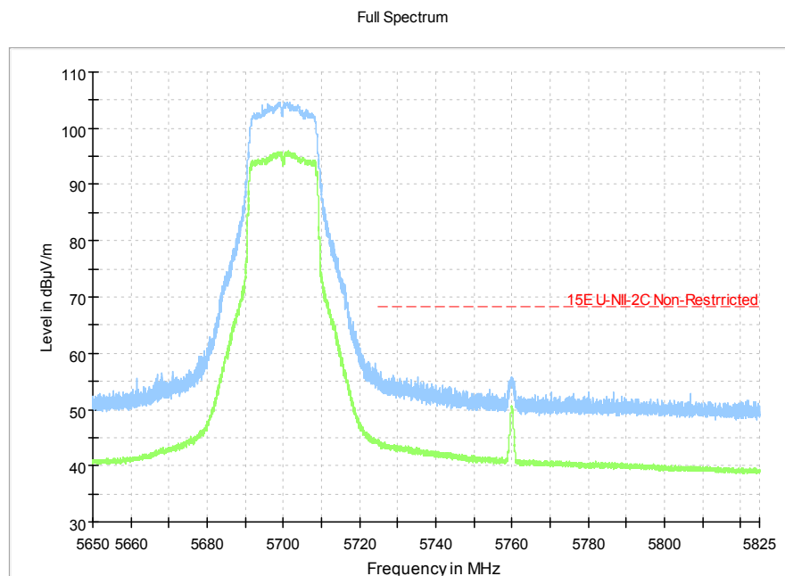
Fig.12 Band Edges (802.11ac-HT20, 5700MHz)
