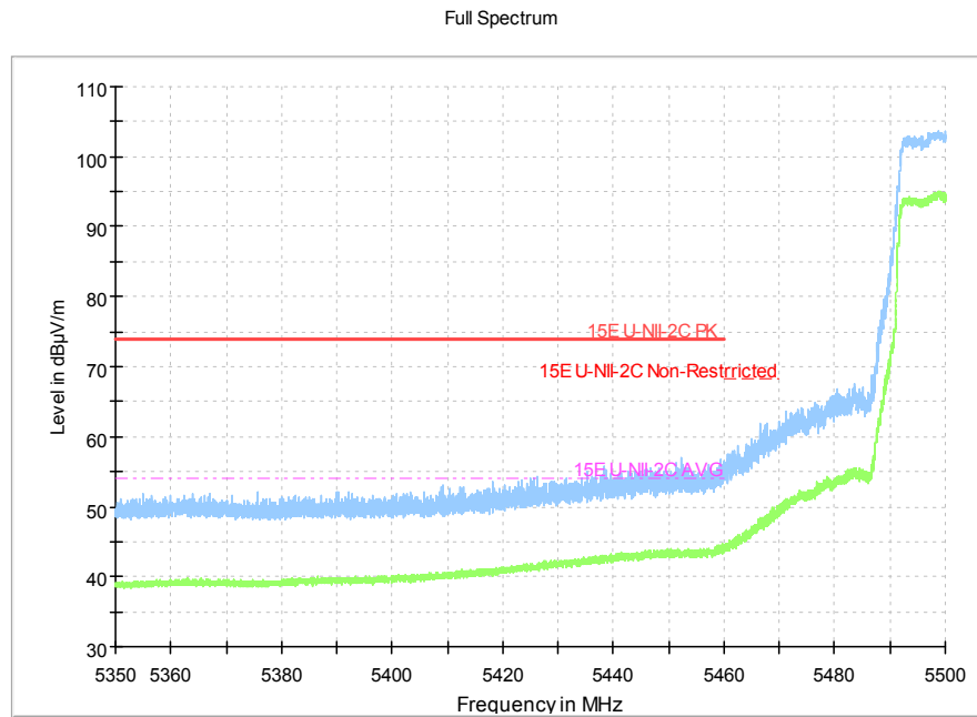
Fig.15 Band Edges (802.11n-HT40, 5510MHz)
