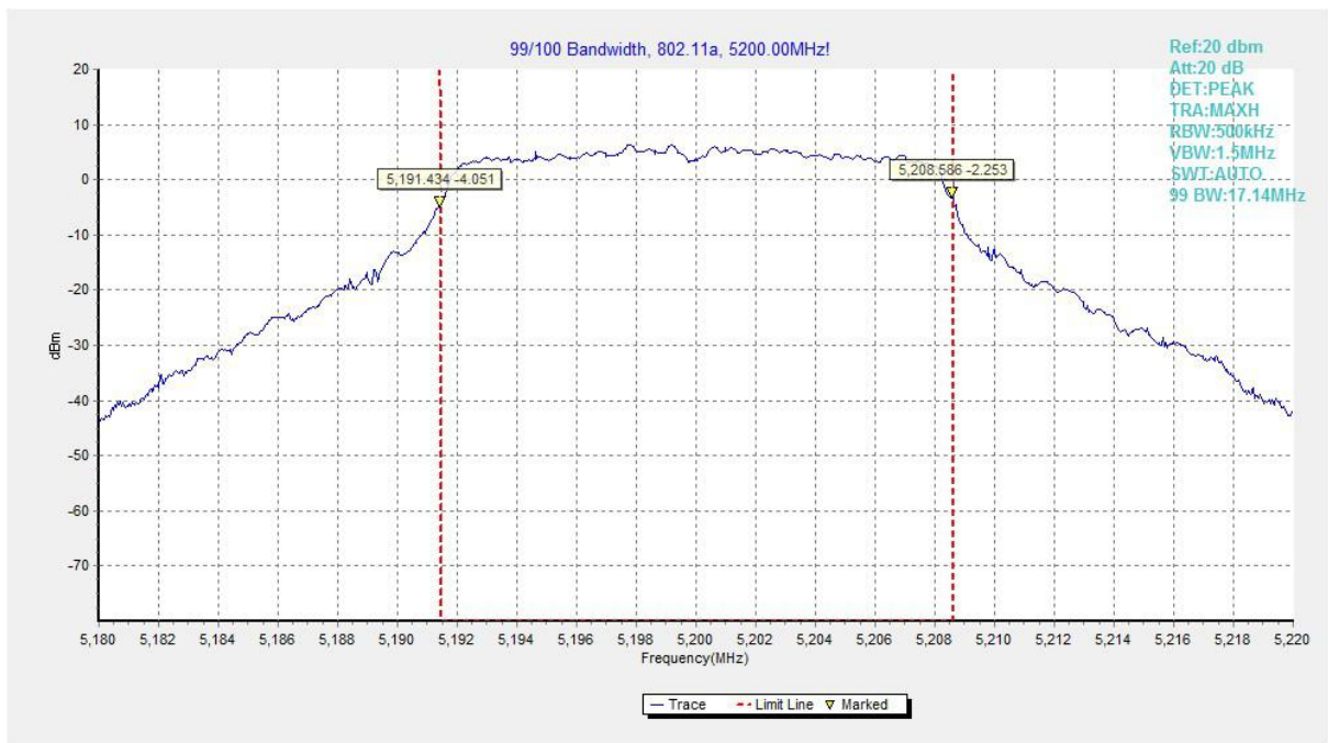
Fig.27 99% Occupied bandwidth (802.11a, 5200MHz)
