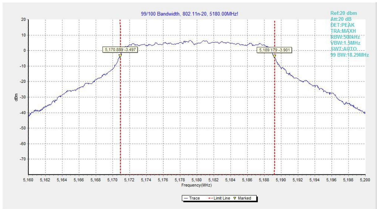
Fig.29 99% Occupied bandwidth (802.11n-HT20, 5180MHz)
