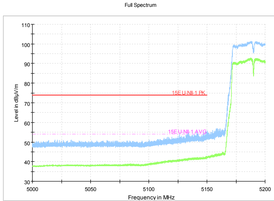
Fig.13 Band Edges (802.11n-HT40, 5190MHz)
