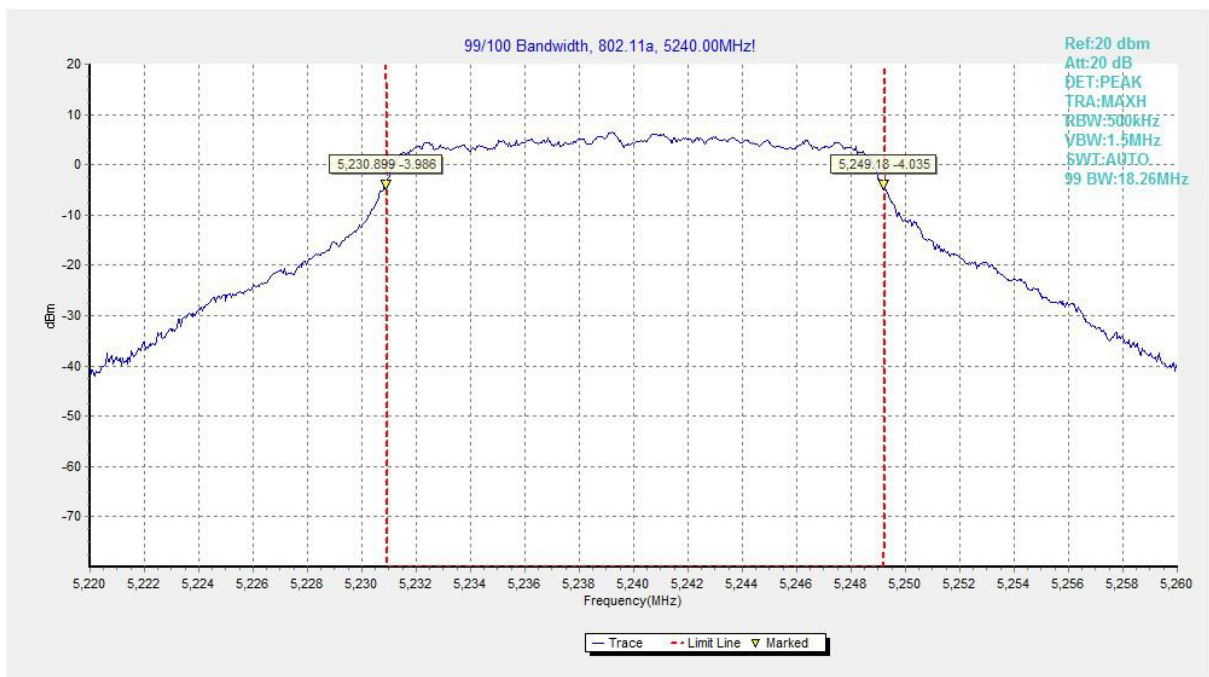
Fig.28 99% Occupied bandwidth (802.11a, 5240MHz)
