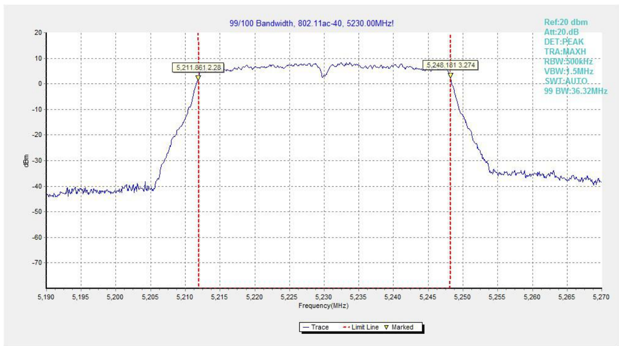
Fig.38 99% Occupied bandwidth (802.11ac-HT40, 5230MHz)
