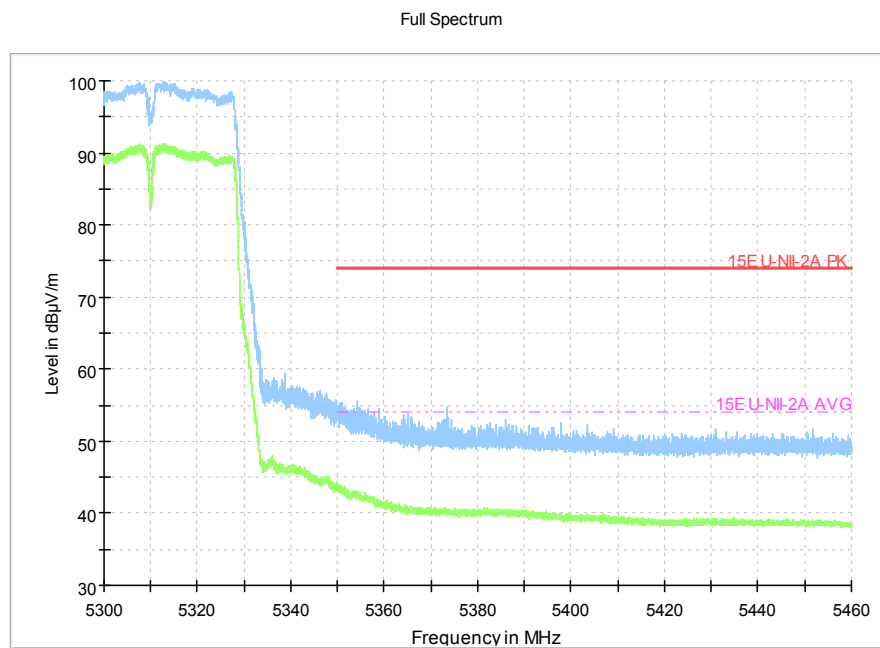
Fig.14 Band Edges (802.11n-HT40, 5310MHz)
