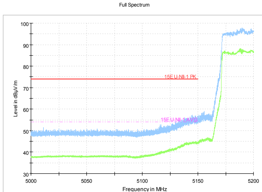
Fig.21 Band Edges (802.11ac-HT80, 5210MHz)
