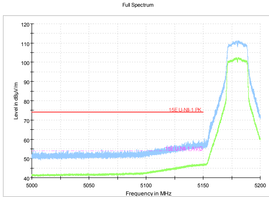
Fig.5 Band Edges (802.11n-HT20, 5180MHz)
