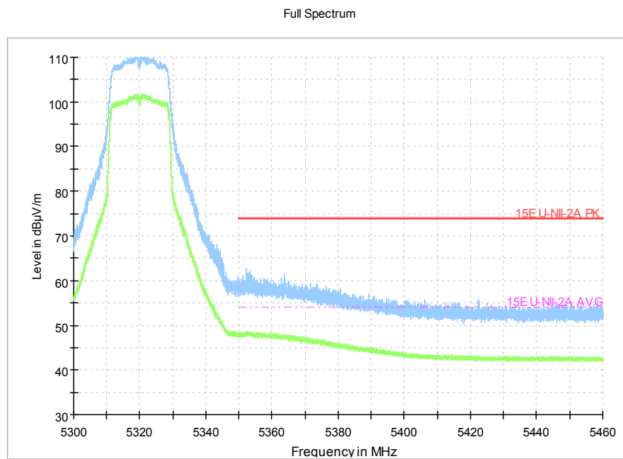
Fig.6 Band Edges (802.11n-HT20, 5320MHz)
