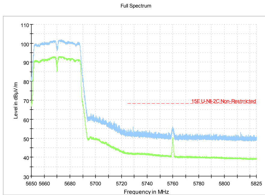
Fig.16 Band Edges (802.11n-HT40, 5670MHz)
