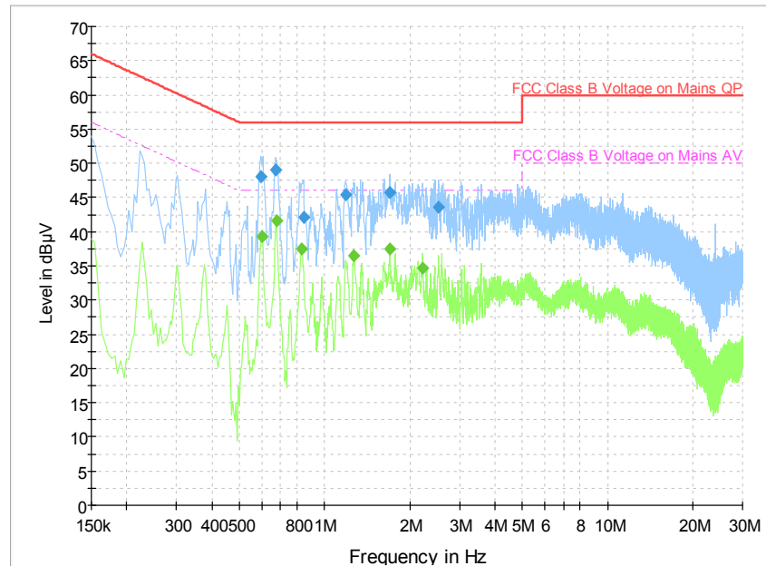
Fig.26 Conducted Emission (802.11a, Ch36, TX)
