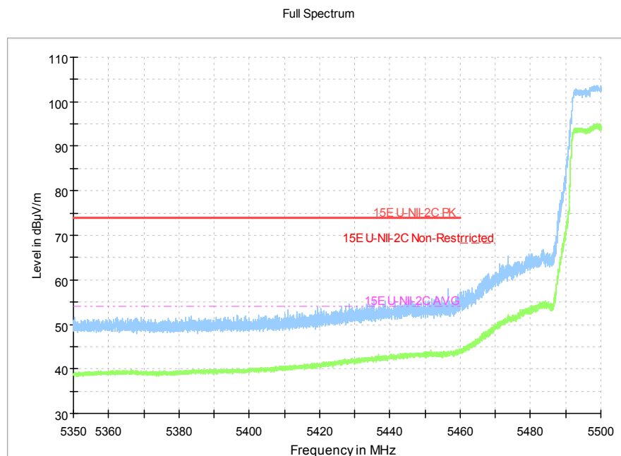
Fig.19 Band Edges (802.11ac-HT40, 5510MHz)
