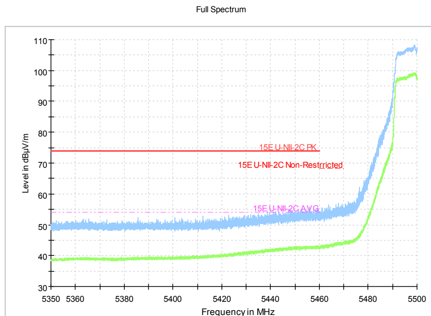
Fig.11 Band Edges (802.11ac-HT20, 5500MHz)
