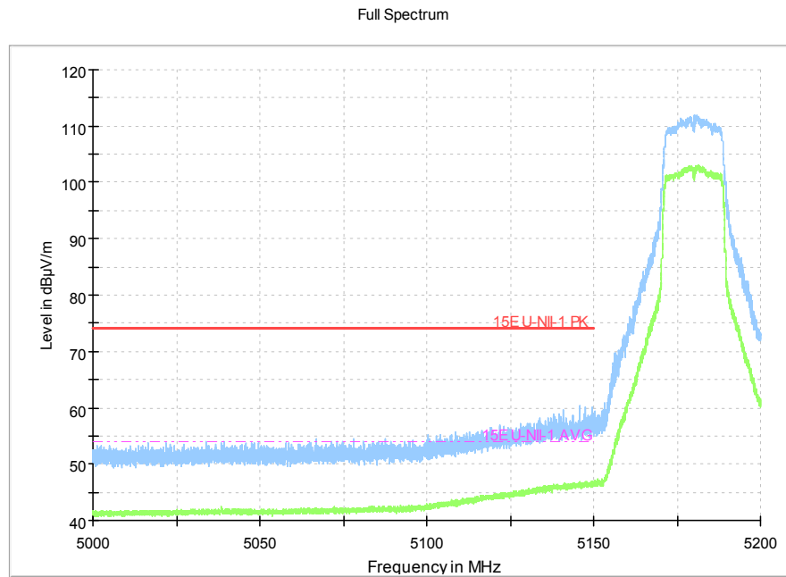
Fig.9 Band Edges (802.11ac-HT20, 5180MHz)
