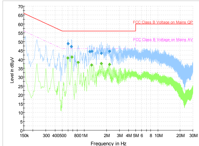
Fig.27 Conducted Emission (802.11a, RX)
