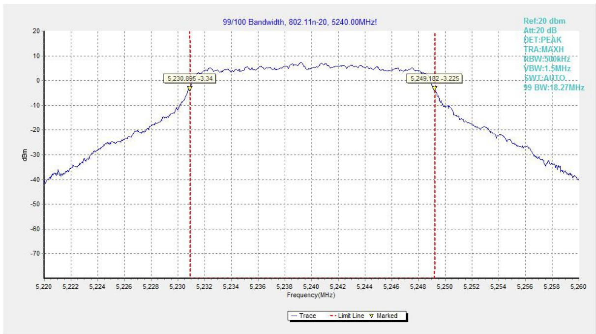
Fig.31 99% Occupied bandwidth (802.11n-HT20, 5240MHz)
