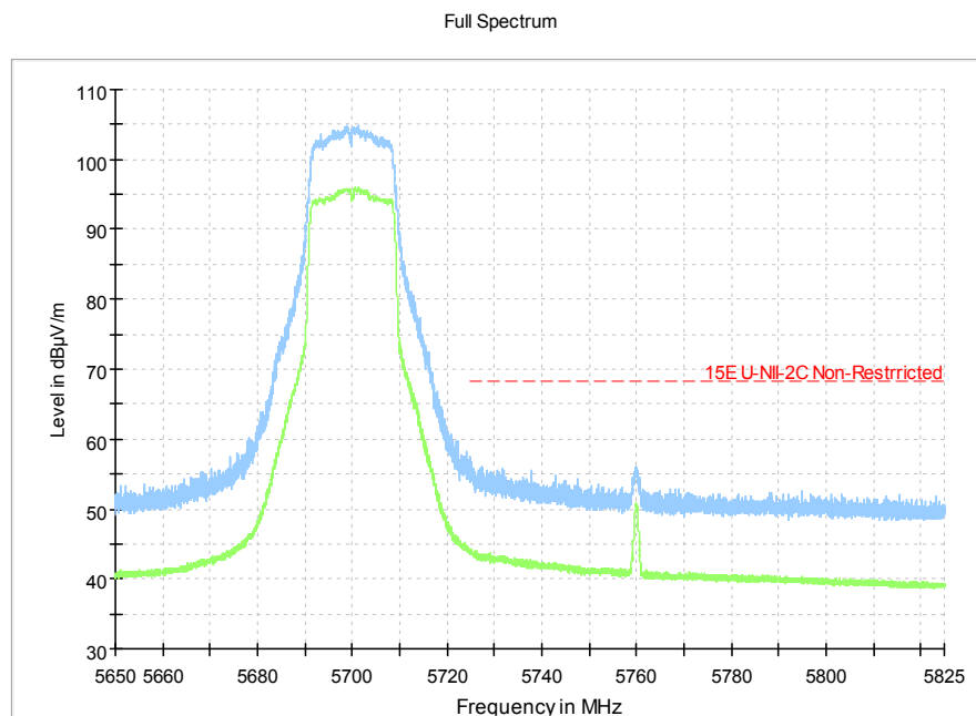
Fig.8 Band Edges (802.11n-HT20, 5700MHz)
