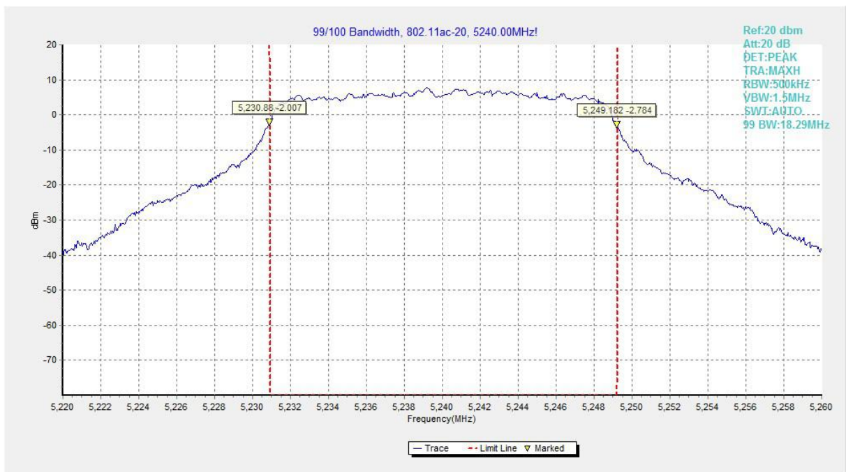
Fig.34 99% Occupied bandwidth (802.11ac-HT20, 5240MHz)
