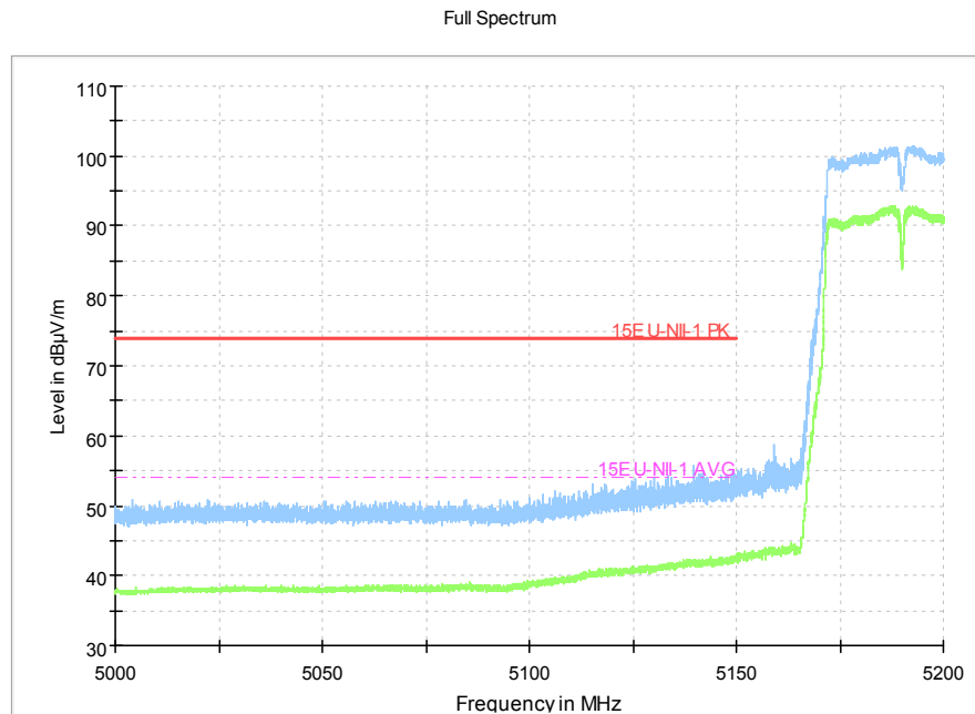
Fig.17 Band Edges (802.11ac-HT40, 5190MHz)
