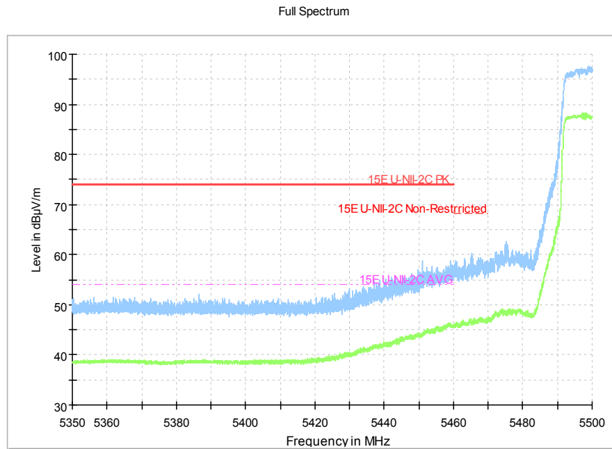
Fig.23 Band Edges (802.11ac-HT80, 5530MHz)
