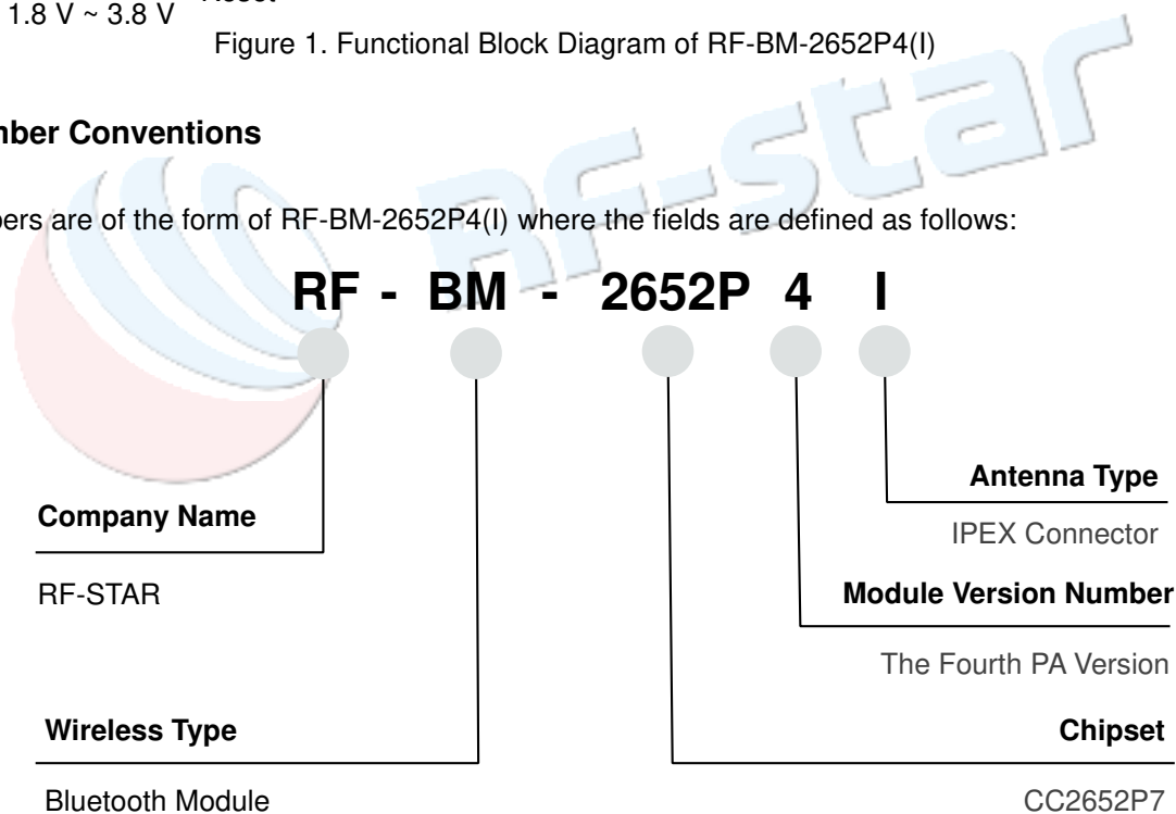
Figure 2. Part Number Conventions of RF-BM-2652P4(I)
