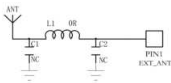
Figure 6. Reference Design of the External Antenna
