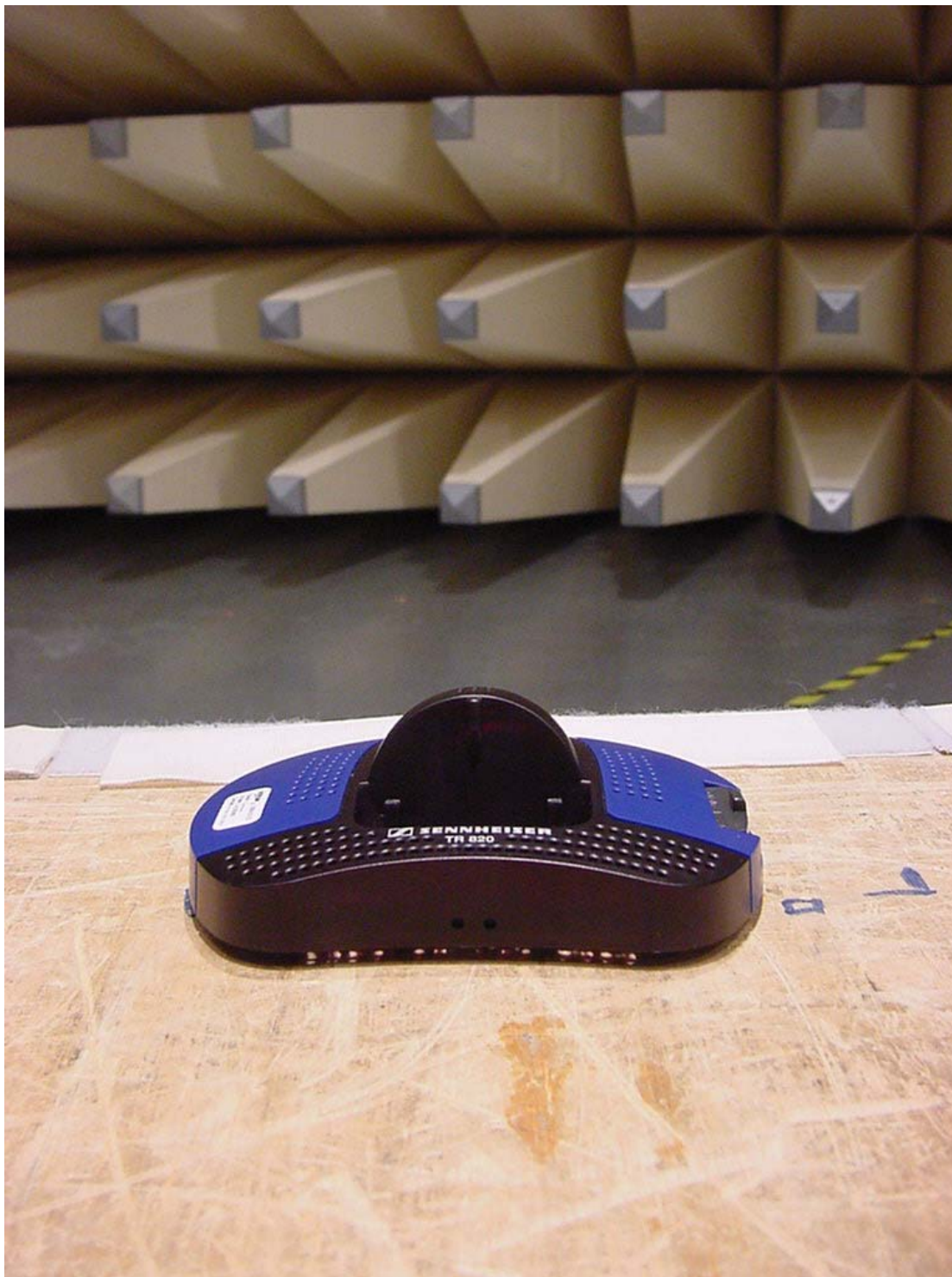
Photo 1 (Radiated Emissions): TR820
