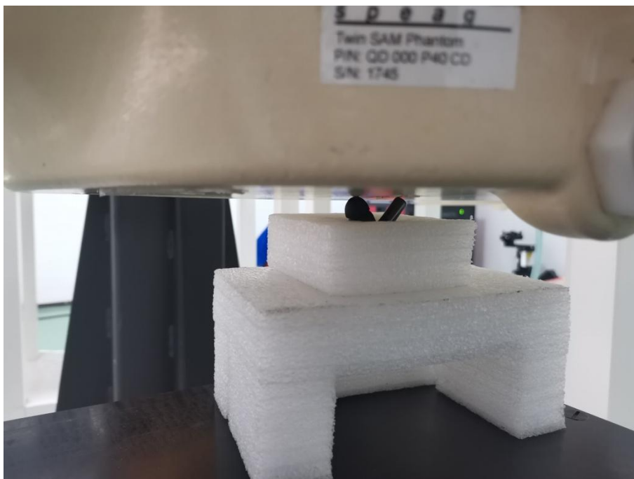
Right earphone-Front Side
