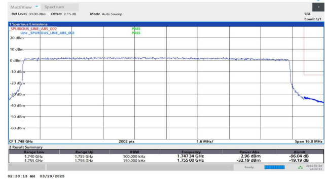
Band4-15MHz-QPSK-20325-75RB#0-PASS
