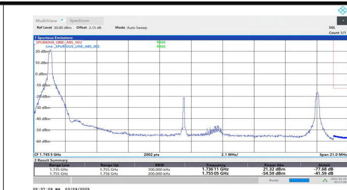
Band4-20MHz-QPSK-20300-1RB#0-PASS
