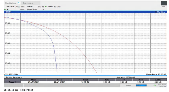
Band4-10MHz-16QAM-20175-27RB#0-PASS
