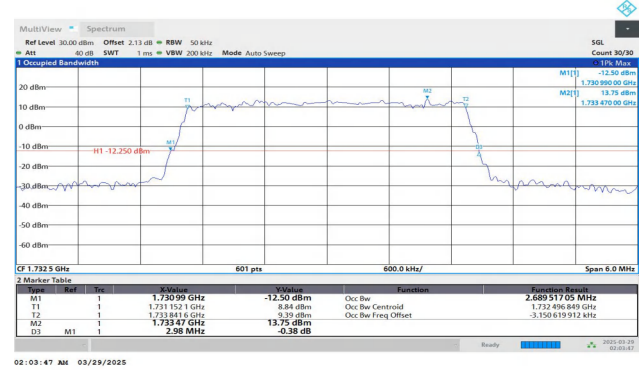
Band4-3MHz-16QAM-20175-15RB#0-PASS
