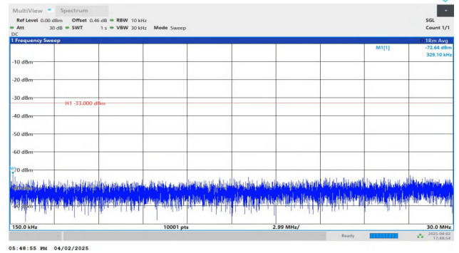
Band4-1.4MHz-QPSK-19957-1RB#0-0.15~30-PASS
