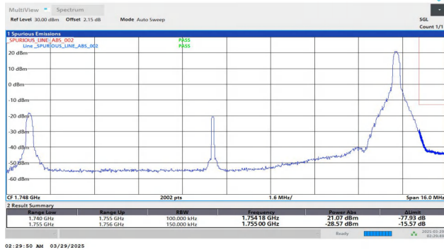
Band4-15MHz-QPSK-20325-1RB#74-PASS
