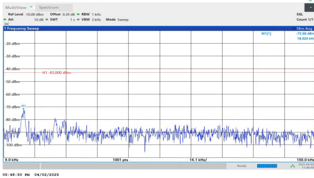
Band4-1.4MHz-QPSK-19957-1RB#0-0.009~0.15-PASS
