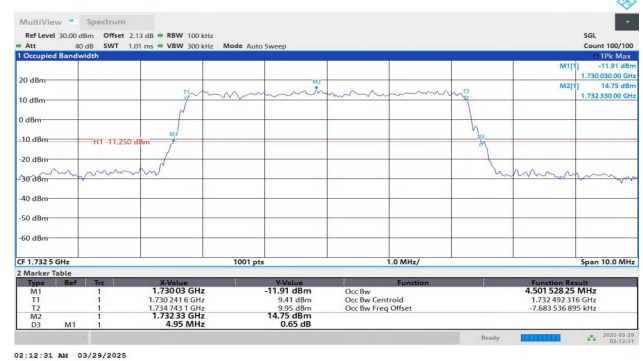
Band4-5MHz-16QAM-20175-25RB#0-PASS
