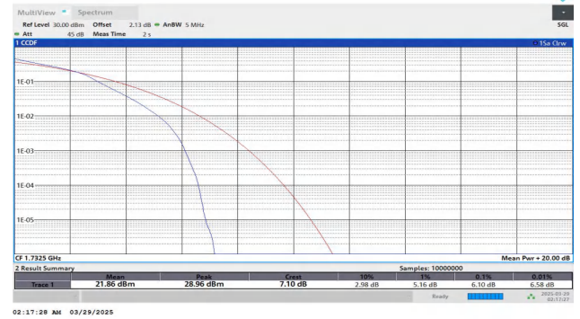
Band4-5MHz-16QAM-20175-25RB#0-PASS
