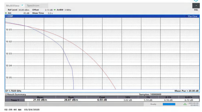
Band4-3MHz-16QAM-20175-15RB#0-PASS
