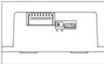
Auxiliary terminals R-SONR-REC-PXA
