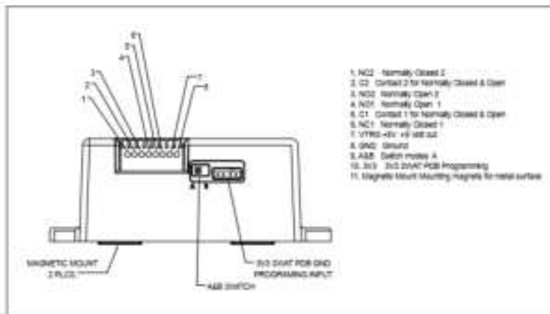
R-SONR-REC-PXA System Connections
