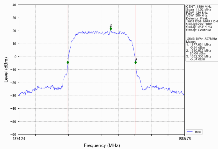
Band2_RMC_MCH_1880MHz_12.2kbps_RMC_NTNV
