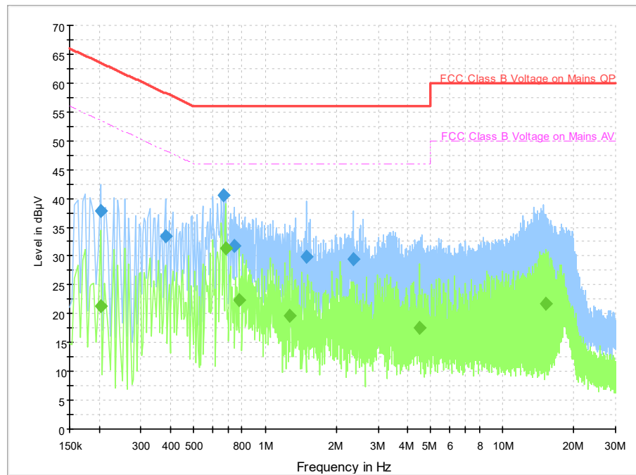
Fig.A.8.2 AC Powerline Conducted Emission-Ide
