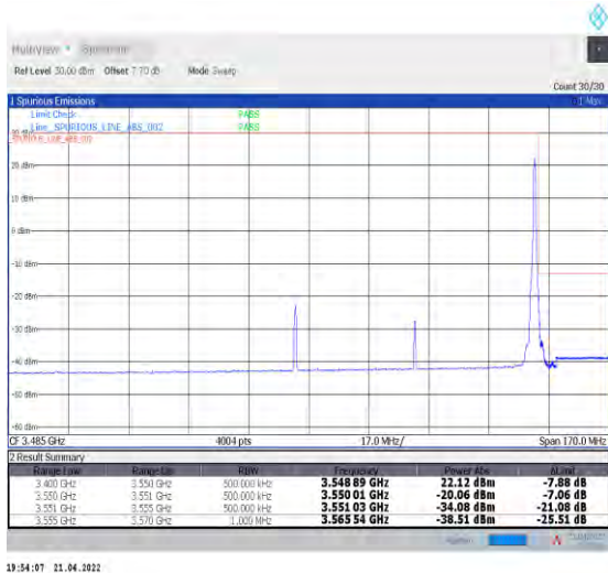
1-N78-3450-3550--30-70-H-5-CP-QPSK-Edge_1RB_Right-1@188-Ant0-PASS-see graph
