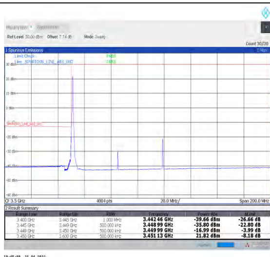
1-N78-3450-3550--30-70-L-1-DFT-PI2BPSK-Edge_1R_B_Left-1@0-Ant0-PASS-see graph
