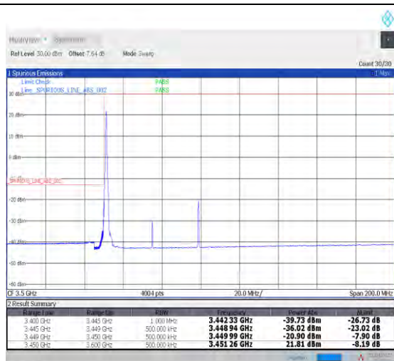
1-N78-3450-3550--30-50-L-1-DFT-PI2BPSK-Edge_1R_B_Left-1@0-Ant0-PASS-see graph
