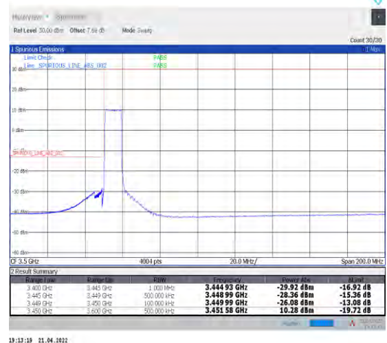
1-N78-3450-3550--30-10-L-6-CP-QPSK-Outer_Ful l-24@0-Ant0-PASS-see graph
