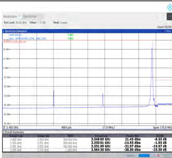
1-N78-3450-3550--30-100-H-2-DFT-PI2BPSK-Edge_1 RB_Right-1@272-Ant0-PASS-see graph
