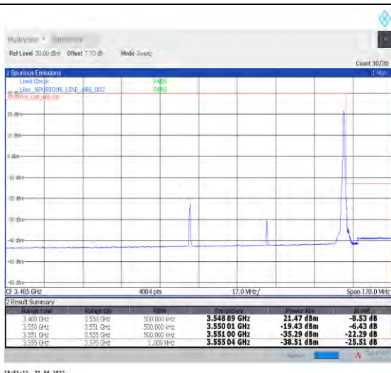
1-N78-3450-3550--30-70-H-2-DFT-PI2BPSK-Edge_1R_B_Right-1@188-Ant0-PASS-see graph
