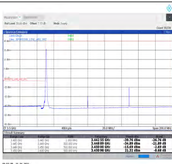
1-N78-3450-3550--30-100-L-1-DFT-PI2BPSK-Edge_1 RB_Left-1@0-Ant0-PASS-see graph
