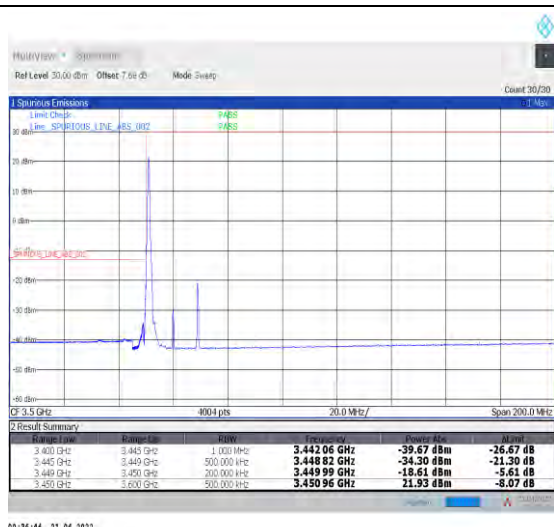
1-N78-3450-3550--30-20-L-1-DFT-PI2BPSK-Edge_1R B_Left-1@0-Ant0-PASS-see graph
