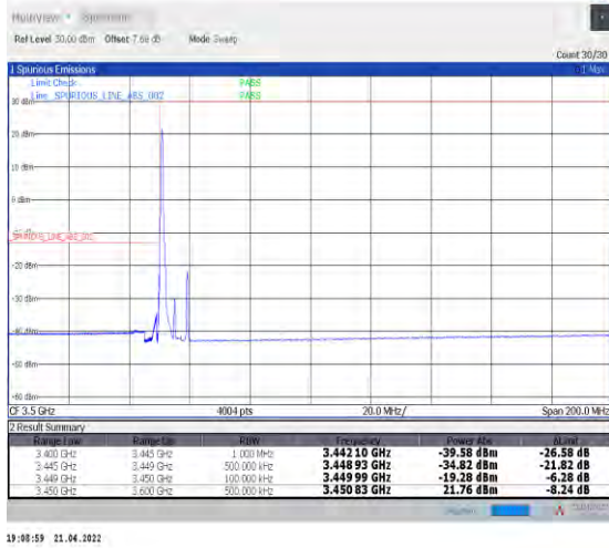
1-N78-3450-3550--30-10-L-1-DFT-PI2BPSK-Edge_1R B_Left-1@0-Ant0-PASS-see graph
