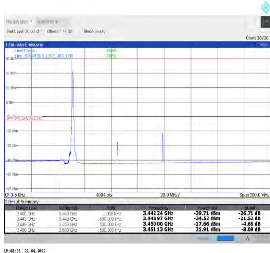
1-N78-3450-3550--30-70-L-4-CP-QPSK-Edge_1RB_L_eft-1@0-Ant0-PASS-see graph
