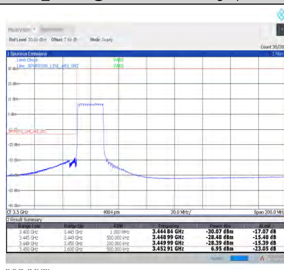
1-N78-3450-3550--30-20-L-6-CP-QPSK-Outer_Ful l-51@0-Ant0-PASS-see graph
