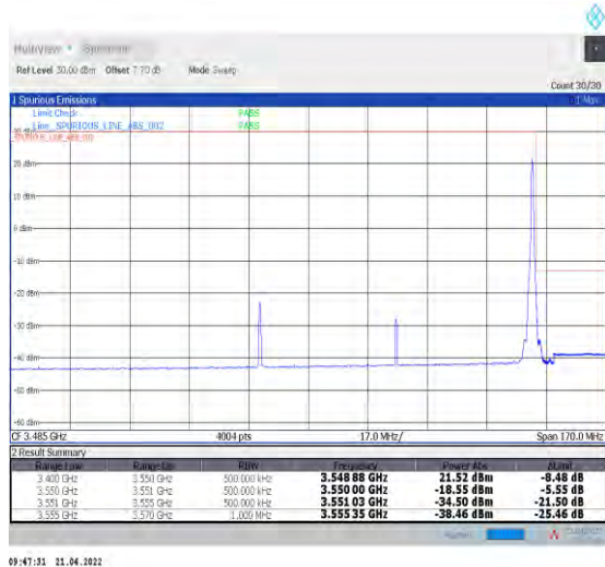
1-N78-3450-3550--30-80-H-5-CP-QPSK-Edge_1RB_Right-1@216-Ant0-PASS-see graph
