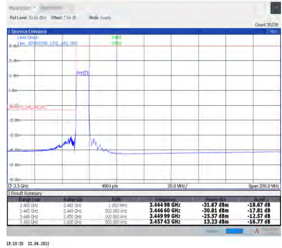
1-N78-3450-3550--30-10-L-3-DFT-PI2BPSK-Outer _Full-24@0-Ant0-PASS-see graph
