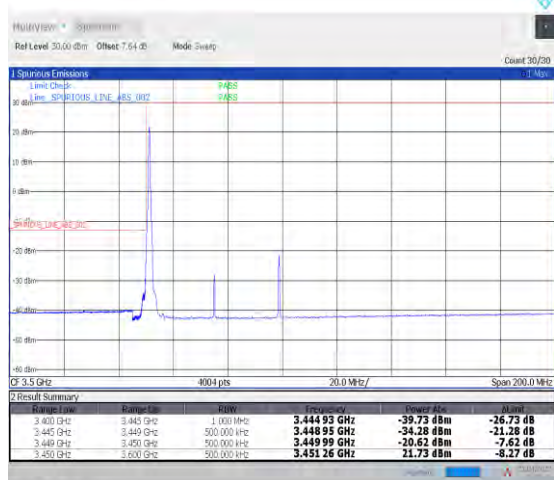
1-N78-3450-3550--30-50-L-4-CP-QPSK-Edge_1RB_L_eft-1@0-Ant0-PASS-see graph
