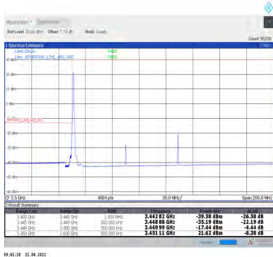
1-N78-3450-3550--30-80-L-4-CP-QPSK-Edge_1RB_L_eft-1@0-Ant0-PASS-see graph
