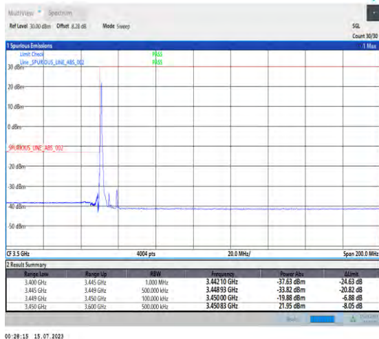
1-N78-3450-3550-PC1-30-10-L-1-DFT-PI2BPSK-Edge_1RB_Left-1@0-Ant0-1--PASS-see graph
