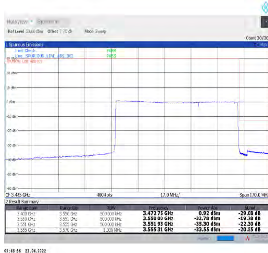
1-N78-3450-3550--30-80-H-6-CP-QPSK-Outer_Full-217@0-Ant0-PASS-see graph
