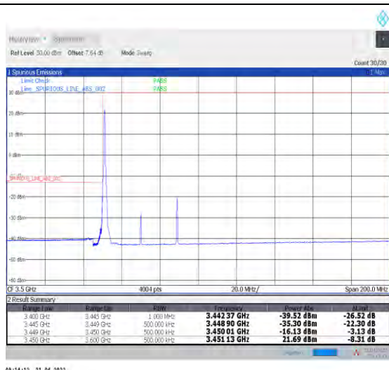
1-N78-3450-3550--30-40-L-1-DFT-PI2BPSK-Edge_1R_B_Left-1@0-Ant0-PASS-see graph
