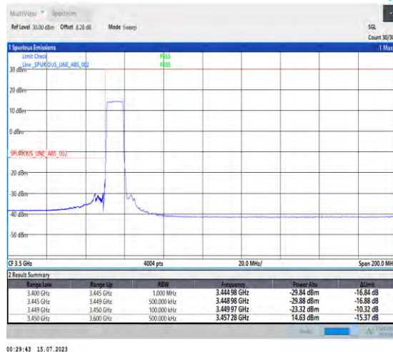
1-N78-3450-3550-PC1-30-10-L-3-DFT-PI2BPSK-Outer_Full-24@0-Ant0-1--PASS-see graph
