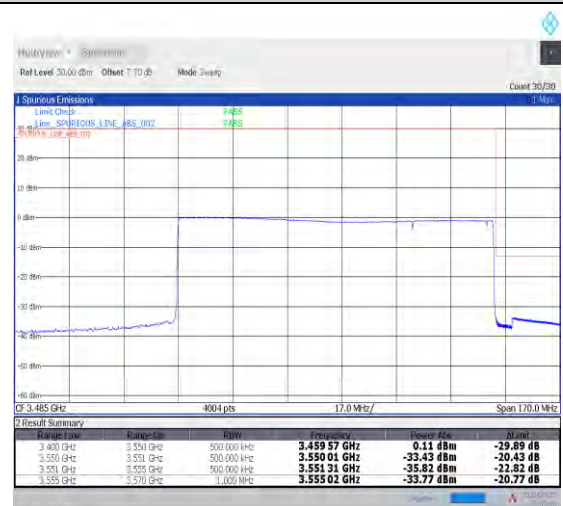
1-N78-3450-3550--30-100-H-3-DFT-PI2BPSK-Out er_Full-270@0-Ant0-PASS-see graph
