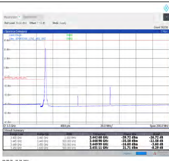
1-N78-3450-3550--30-80-L-1-DFT-PI2BPSK-Edge_1R_B_Left-1@0-Ant0-PASS-see graph
