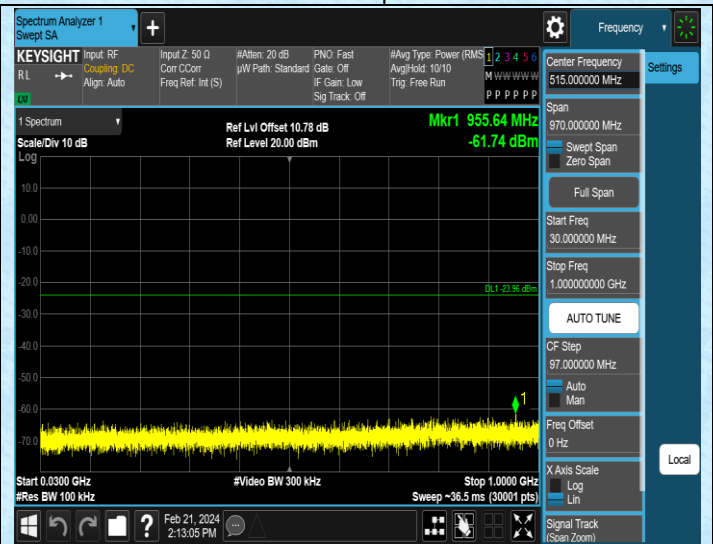
11AX20SISO-Ant1-2412-30-1000-PASS
