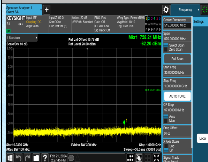
11AX20SISO-Ant2-2412-30-1000-PASS
