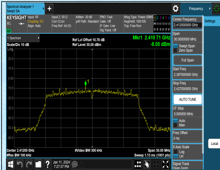
11N20MIMO-Ant1-2412-0~Reference-PASS
