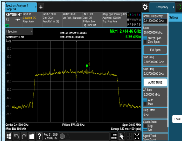
11AX20SISO-Ant1-2412-0-Reference-PASS
