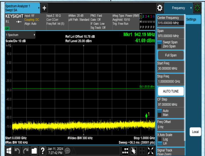
11N20MIMO-Ant1-2412-30~1000-PASS
