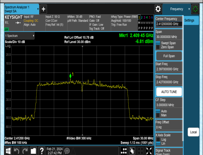
11AX20SISO-Ant2-2412-0-Reference-PASS
