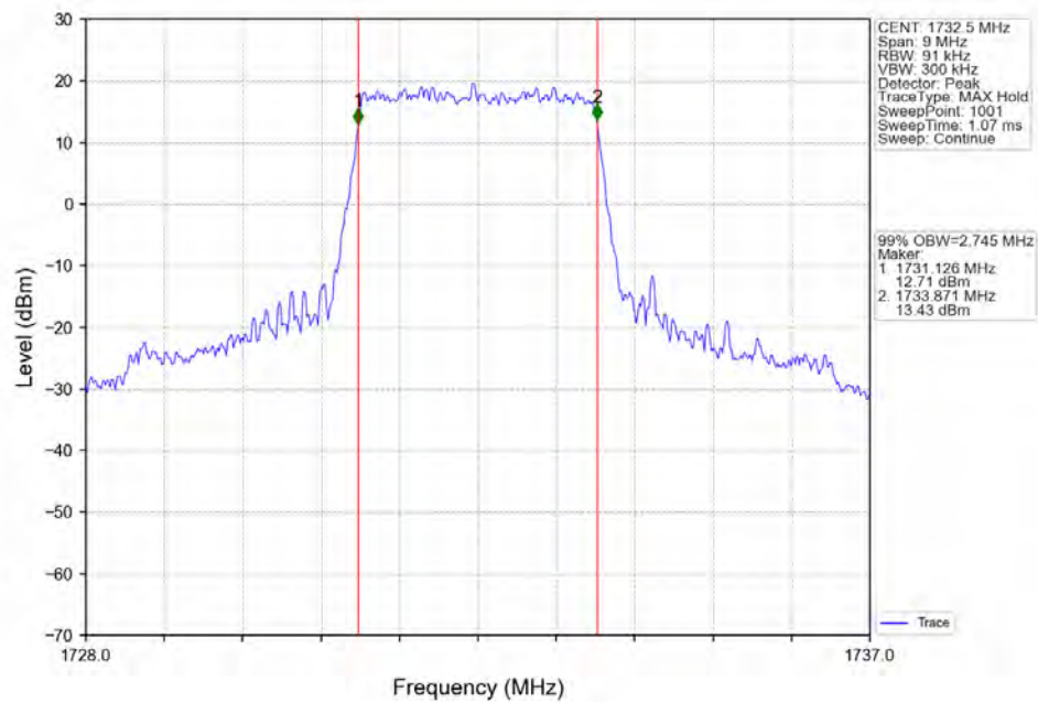
Band4_3MHz_16QAM_MCH_1732.5MHz_RB_15_0_NTNV
