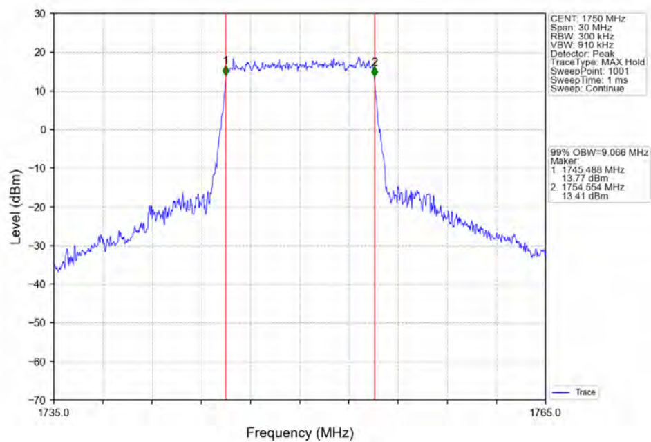
Band4_10MHz_64QAM_HCH_1750MHz_RB_50_0_NTNV
