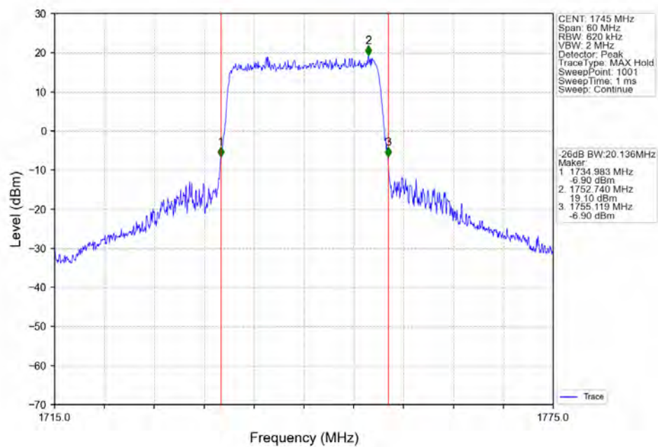
Band4_20MHz_64QAM_HCH_1745MHz_RB_100_0_NTNV
