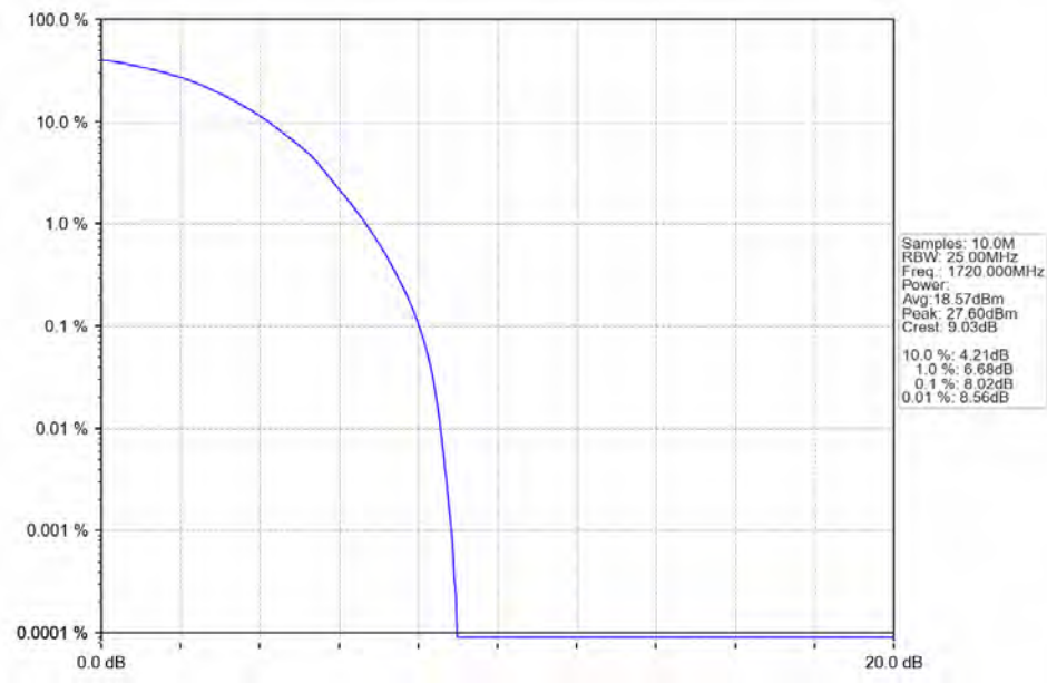
Band4_20MHz_64QAM_LCH_1720MHz_RB_100_0_NTNV
