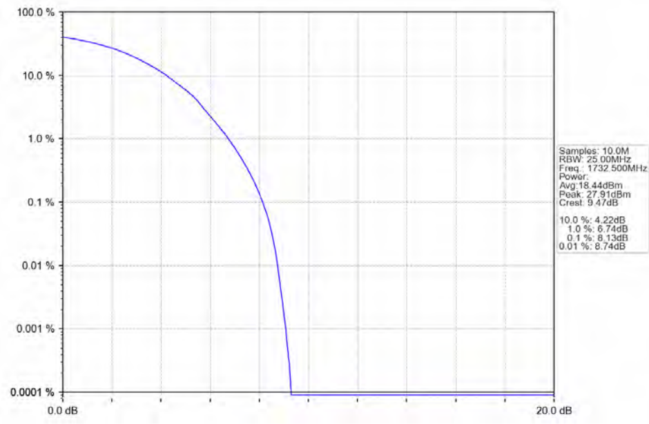
Band4_20MHz_64QAM_MCH_1732.5MHz_RB_100_0_NTNV
