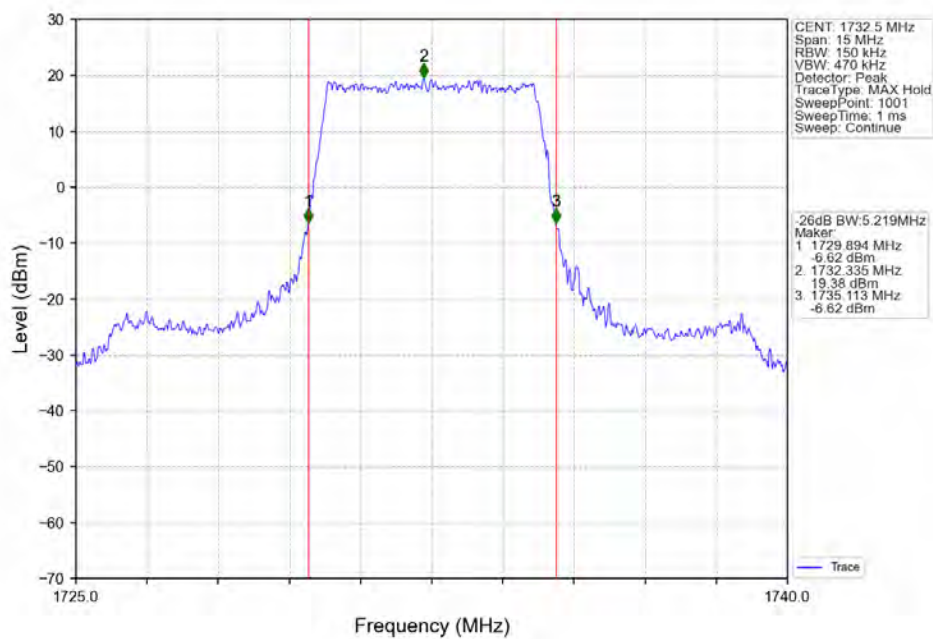
Band4_5MHz_QPSK_MCH_1732.5MHz_RB_25_0_NTN
