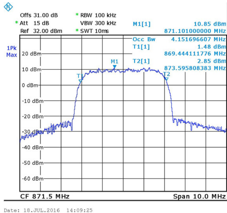
Figure 35. — W-CDMA - Output 871.5MHz
