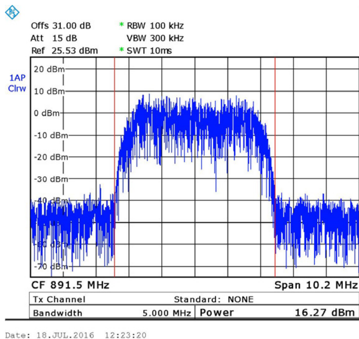
Figure 19. — W-CDMA - 891.5 MHz
