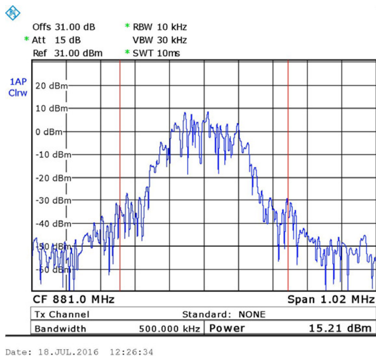
Figure 15. — GSM - 881.0 MHz
