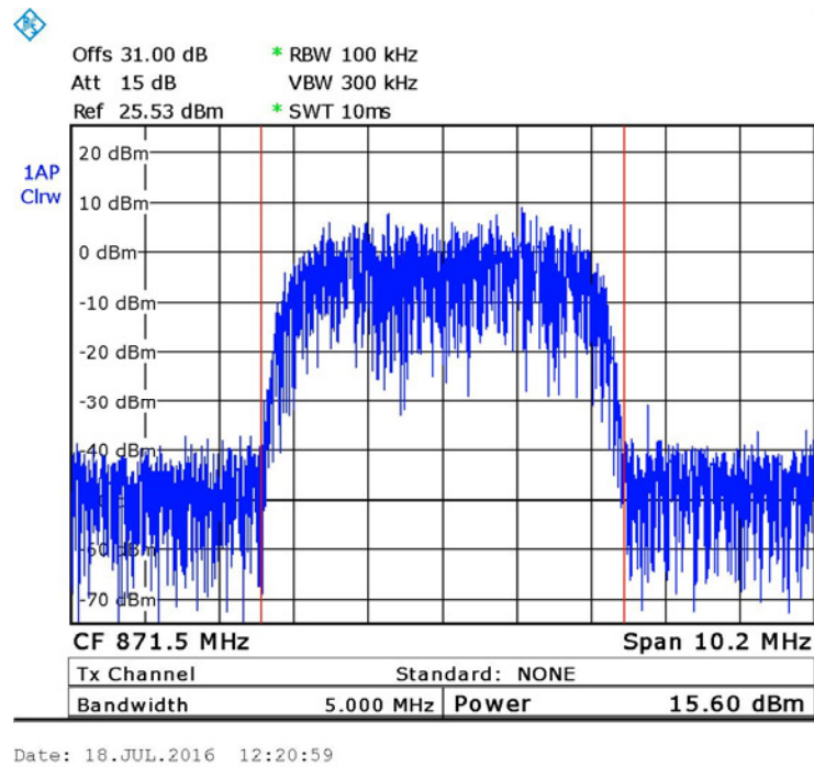
Figure 17. — W-CDMA - 871.5 MHz
