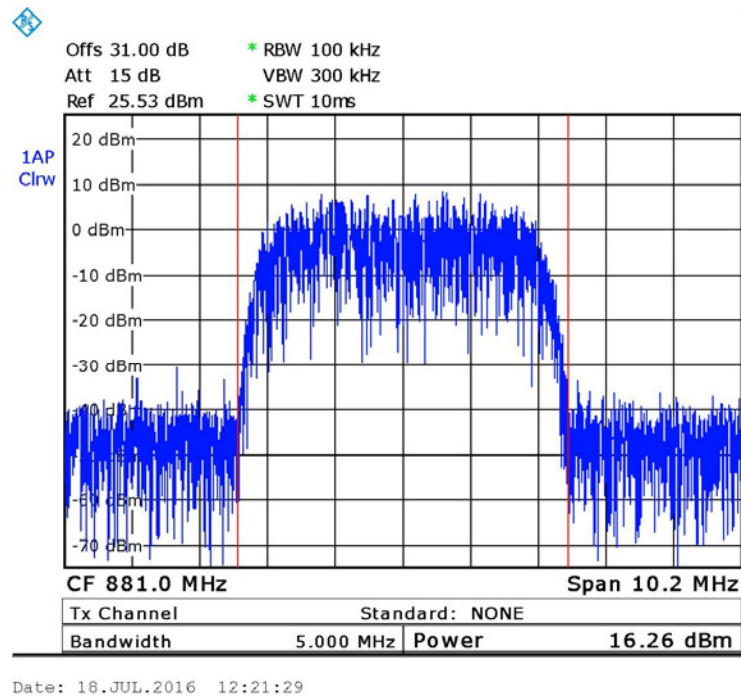
Figure 18. — W-CDMA - 881.0 MHz
