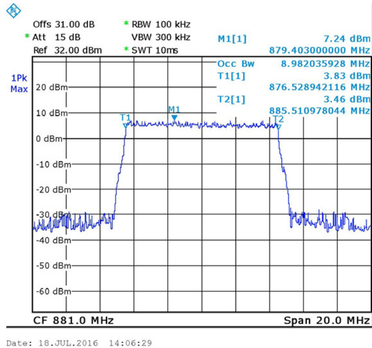
Figure 25. — LTE 64QAM Output 881.0MHz
