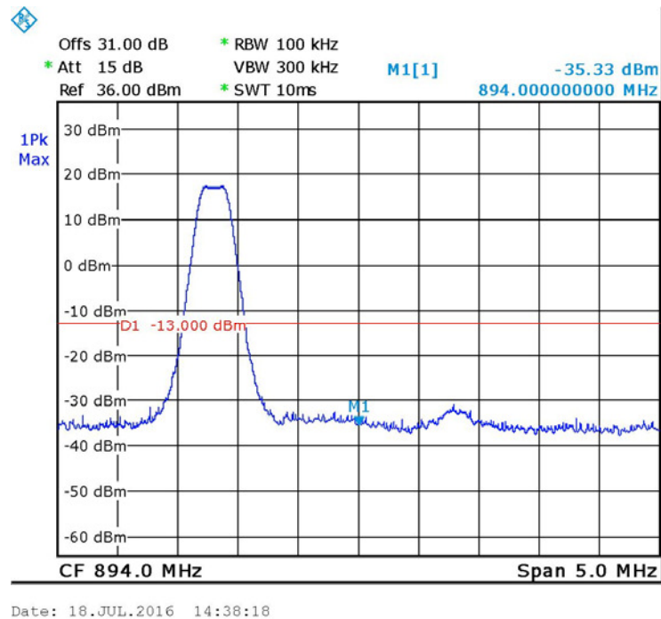
Figure 55. — GSM - 892.8 MHz
