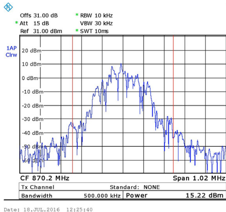
Figure 14. — GSM - 870.2 MHz
