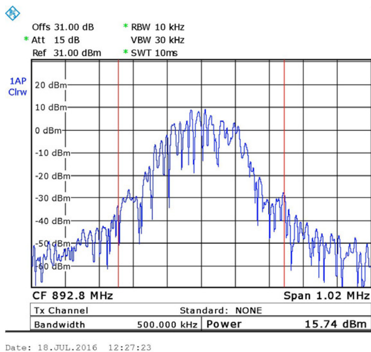
Figure 16. — GSM - 892.8 MHz
