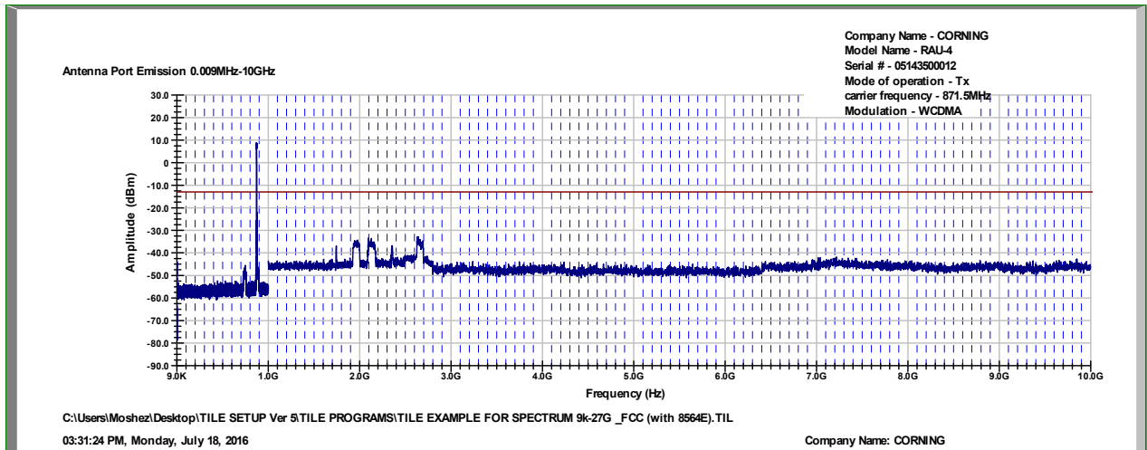
Figure 47. — W-CDMA - 871.5 MHz
