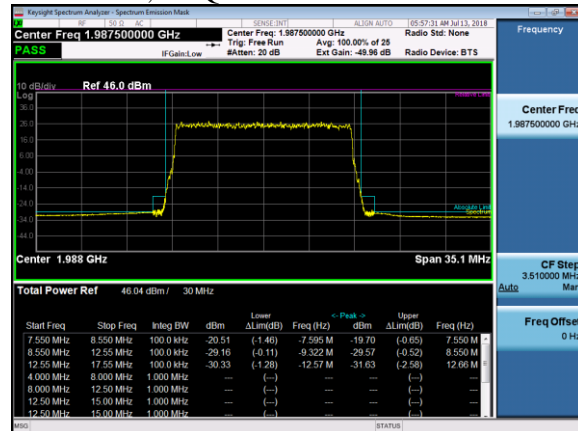
1987.5 MHz, 256QAM
