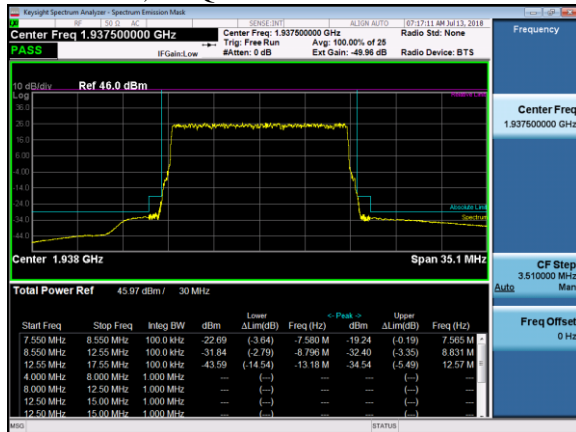
1937.5 MHz, 256QAM
