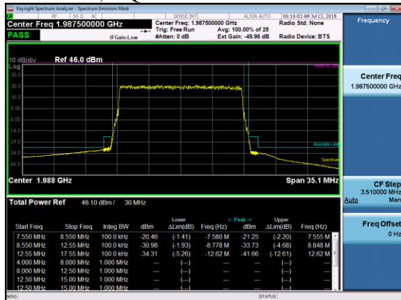
1987.5 MHz, 64QAM
