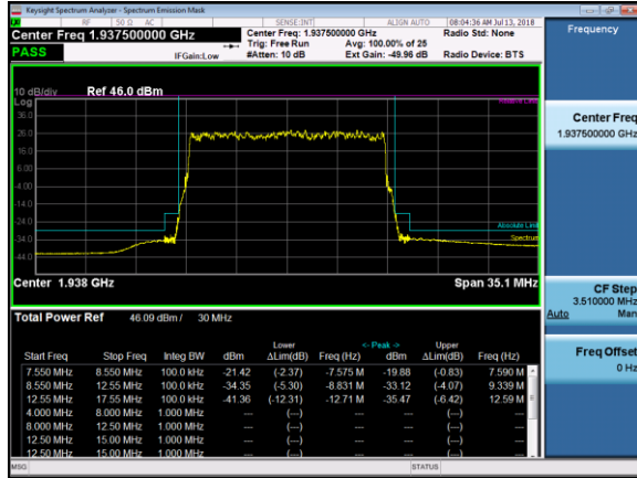
1937.5 MHz, QPSK+16QAM
