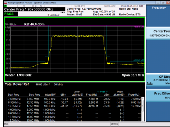
1937.5 MHz, 64QAM
