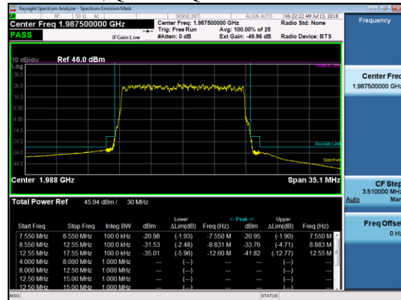
1987.5 MHz, QPSK+16QAM
