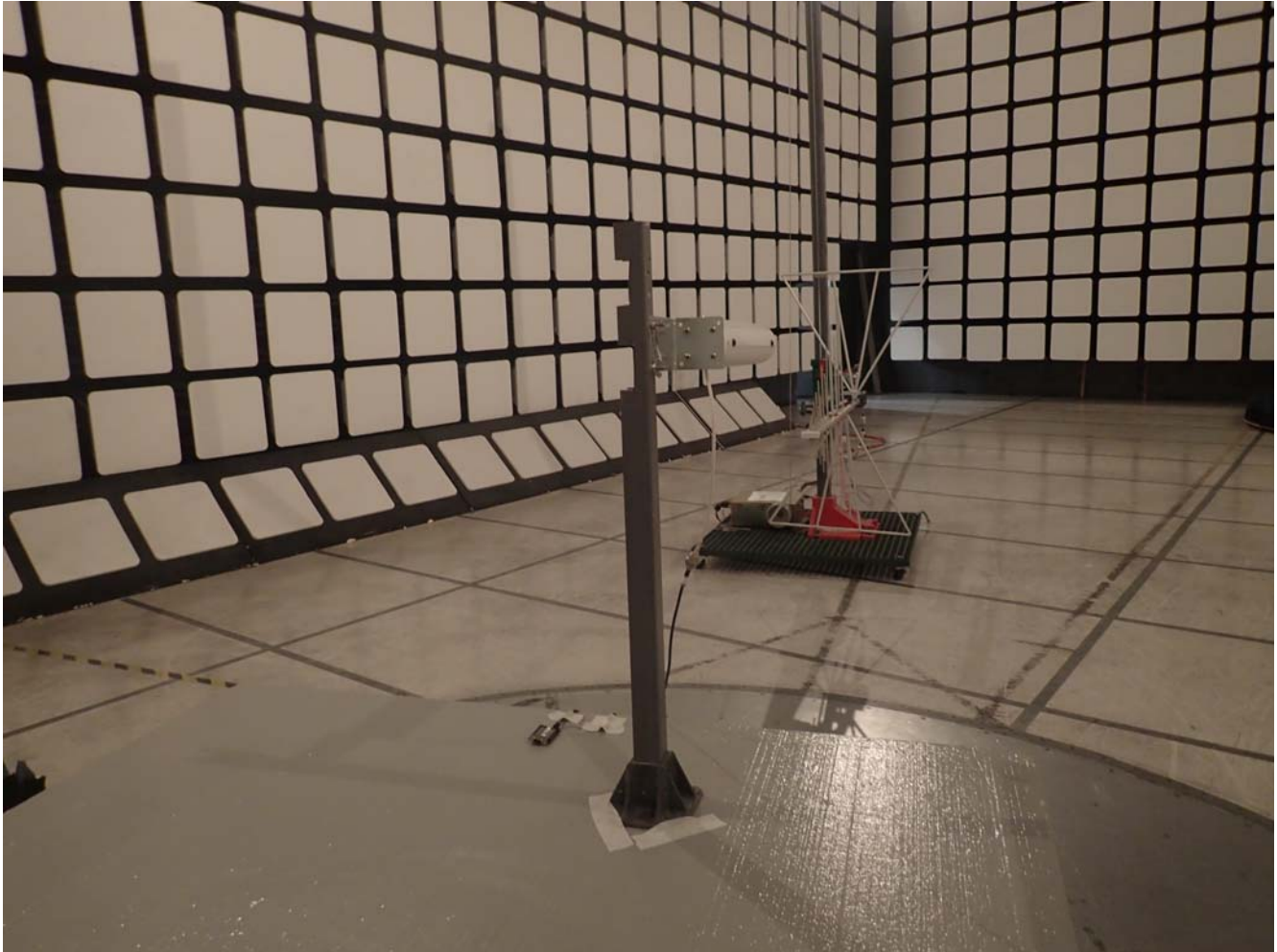
Radiated Emissions @ 3 m EUT with 14.5 dBi Yagi Antenna, Orthogonal Position 1
