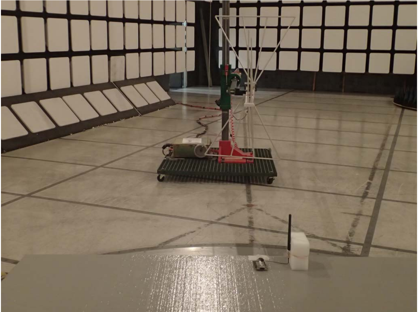
Radiated Emissions @ 3 m EUT with 2.5 dBi Dipole Antenna, Orthogonal Position 1
