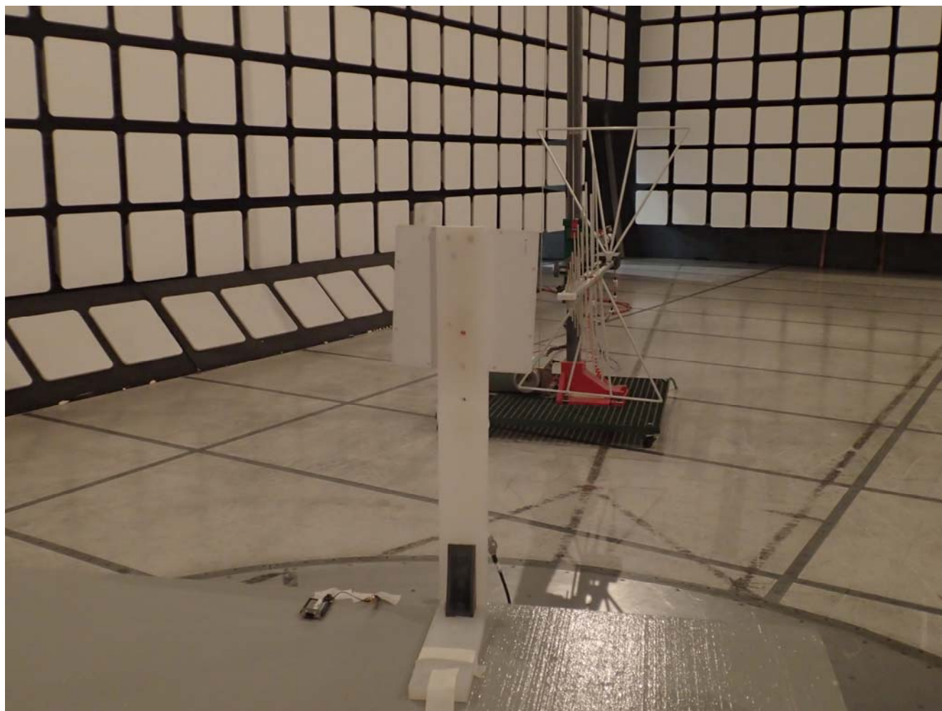
Radiated Emissions @ 3 m EUT with 14 dBi Patch Antenna, Orthogonal Position 1
