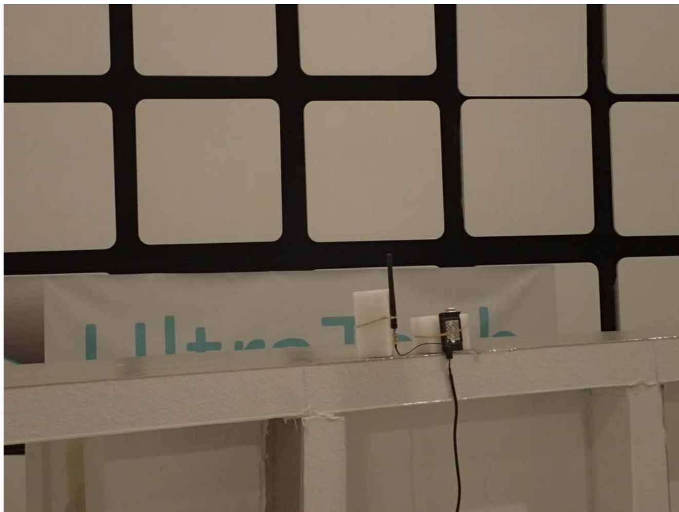
Radiated Emissions @ 3 m EUT with 2.5 dBi Dipole Antenna, Orthogonal Position 3
