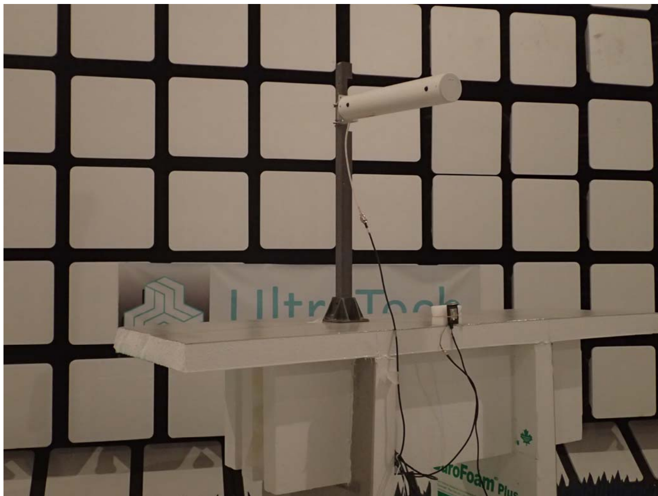
Radiated Emissions @ 3 m EUT with 14.5 dBi Yagi Antenna, Orthogonal Position 3
