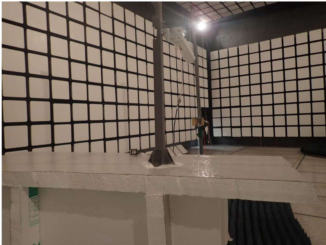
Radiated Emissions @ 3 m EUT with 14.5 dBi Yagi Antenna, Orthogonal Position 2
