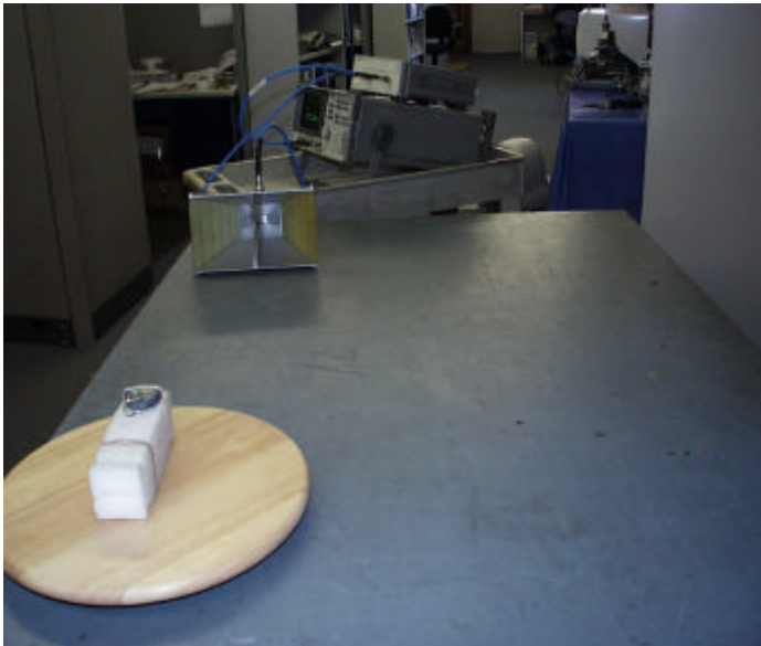
Radiated Open Site Test Set-up
