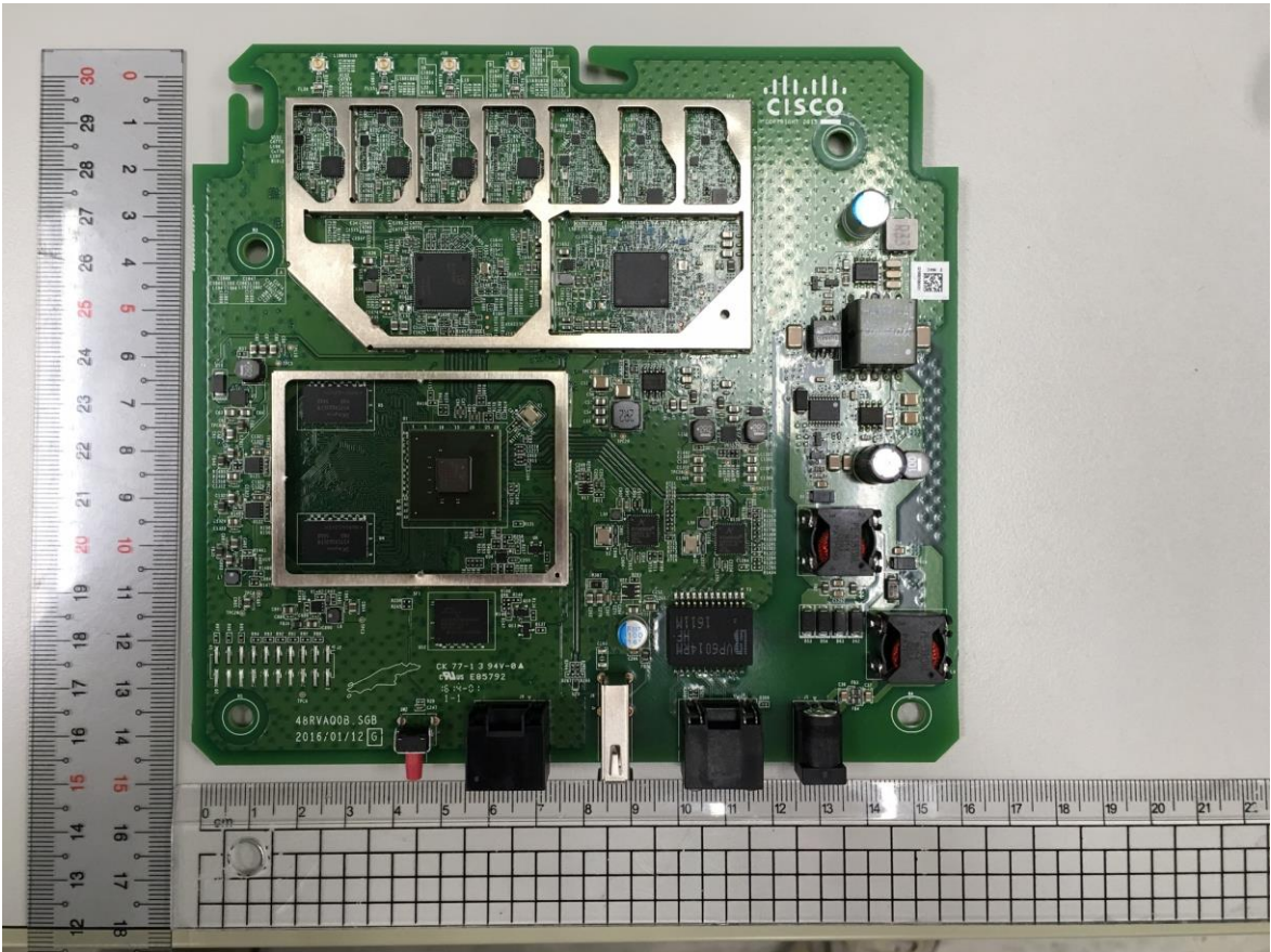
Top Side Board without Shields
