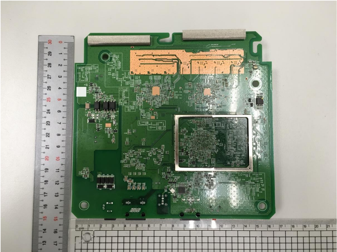
Bottom Side Board Without Shield
