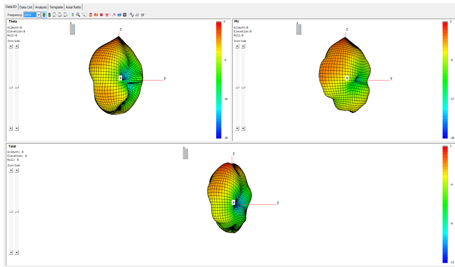
Fig. 4 antenna radiation pattern diagram
