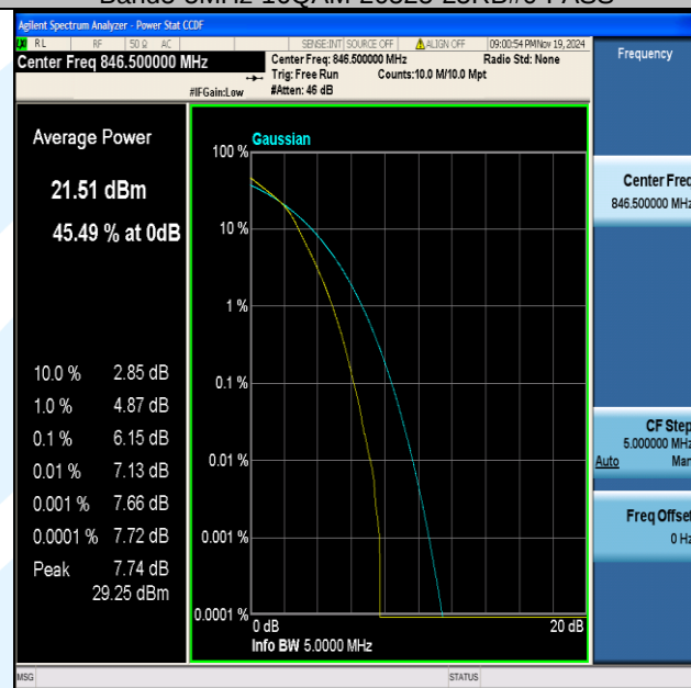
Band5-5MHz-16QAM-20625-25RB#0-PASS
