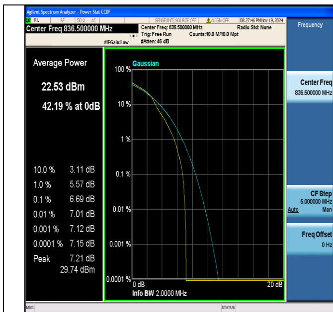
Band5-1.4MHz-16QAM-20525-1RB#0-PASS
