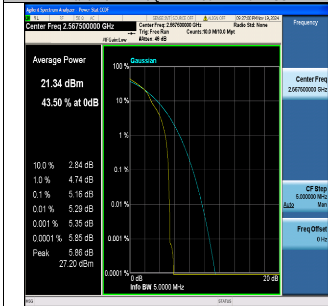
Band7-5MHz-16QAM-21425-1RB#0-PASS
