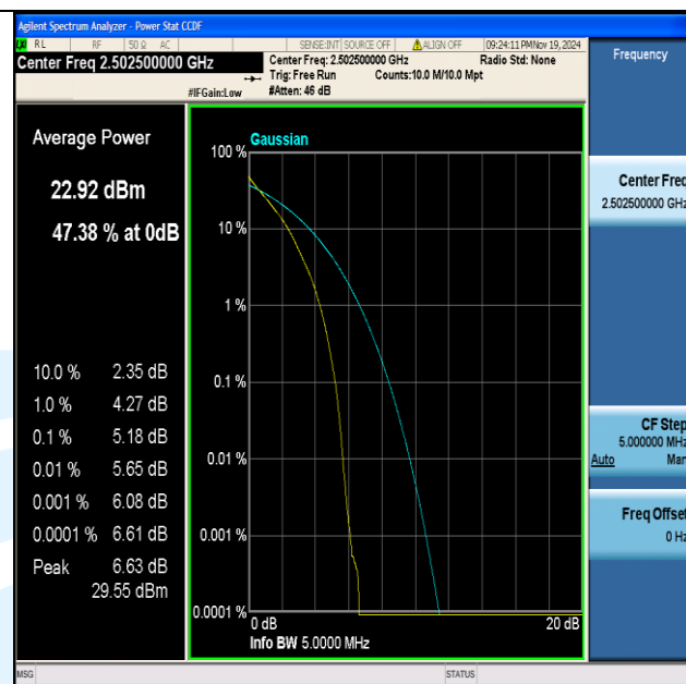
Band7-5MHz-QPSK-20775-25RB#0-PASS
