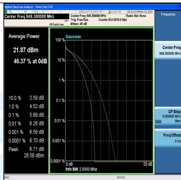
Band5-1.4MHz-QPSK-20643-6RB#0-PASS
