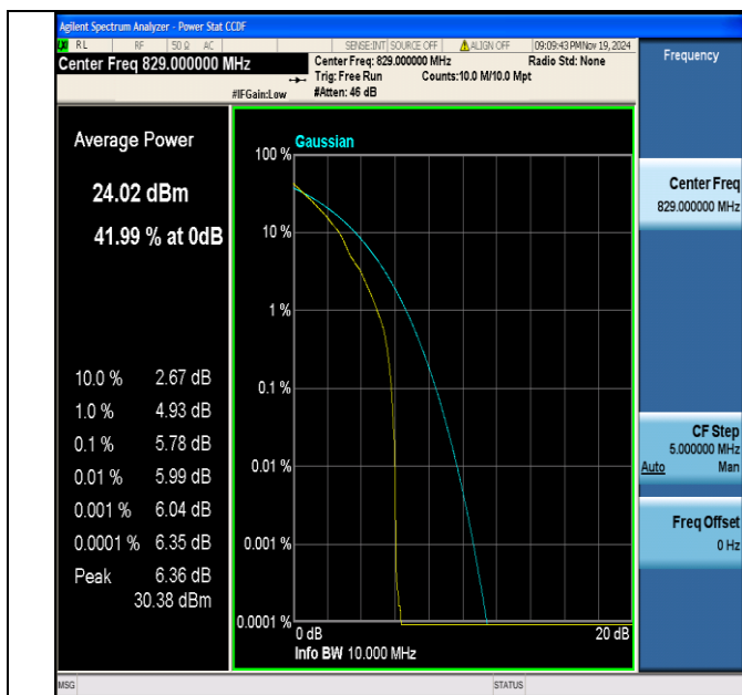
Band5-10MHz-QPSK-20450-1RB#0-PASS
