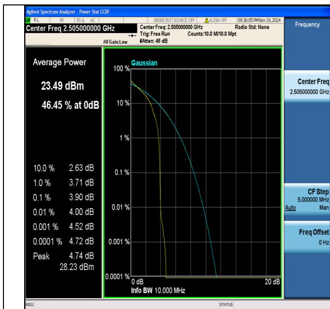
Band7-10MHz-QPSK-20800-1RB#0-PASS
