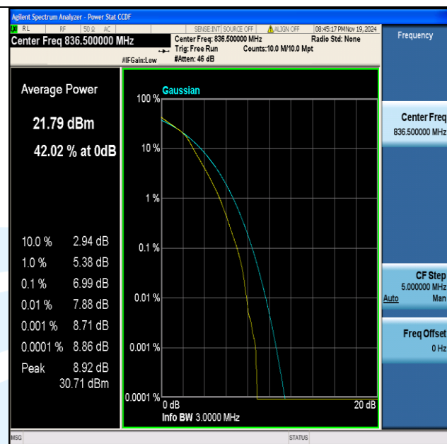
Band5-3MHz-16QAM-20525-15RB#0-PASS
