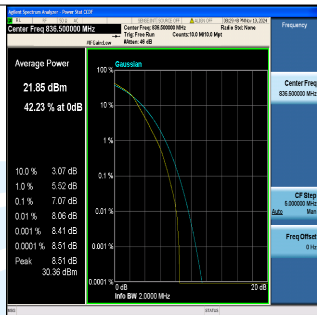
Band5-1.4MHz-16QAM-20525-6RB#0-PASS
