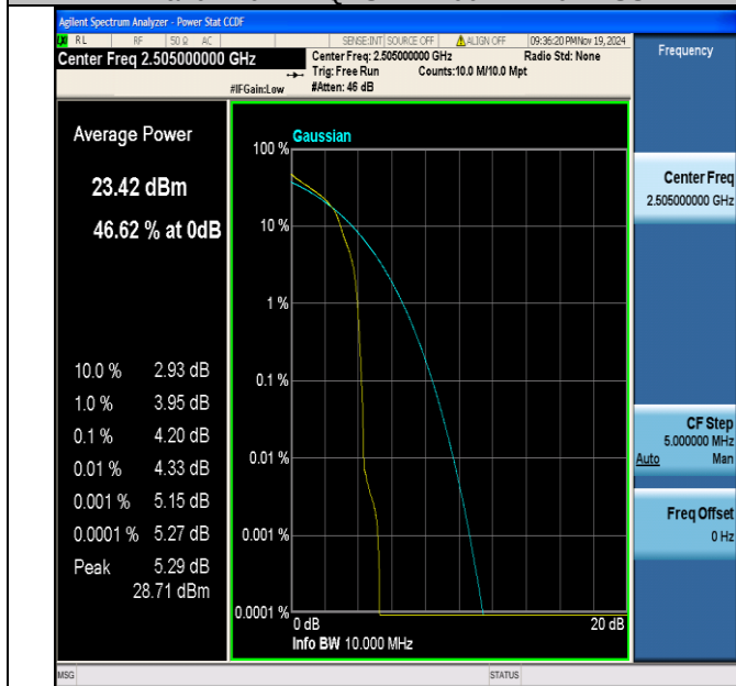
Band7-10MHz-16QAM-20800-1RB#0-PASS
