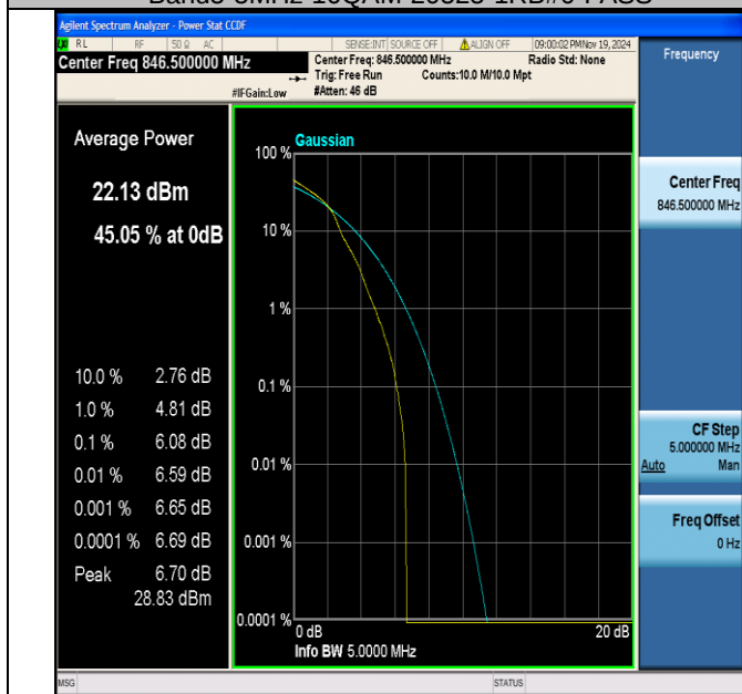
Band5-5MHz-16QAM-20625-1RB#0-PASS
