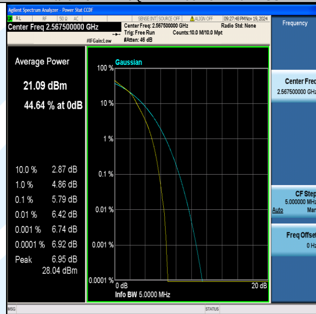
Band7-5MHz-16QAM-21425-25RB#0-PASS
