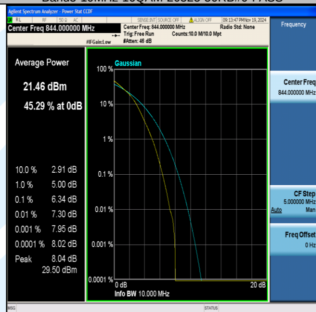
Band5-10MHz-16QAM-20600-50RB#0-PASS
