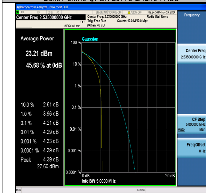
Band7-5MHz-QPSK-21100-1RB#0-PASS
