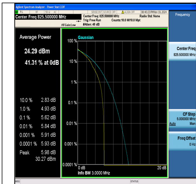
Band5-3MHz-QPSK-20415-1RB#0-PASS
