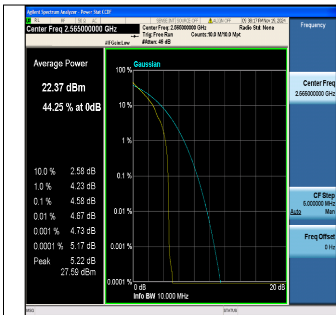
Band7-10MHz-QPSK-21400-1RB#0-PASS
