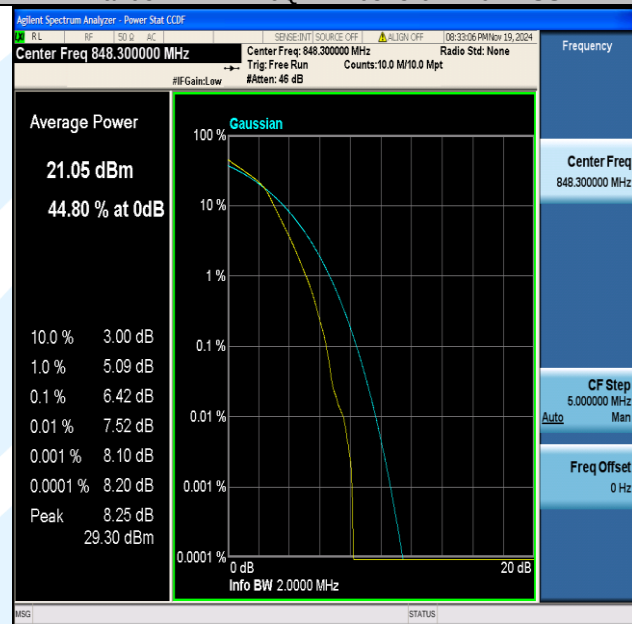
Band5-1.4MHz-16QAM-20643-6RB#0-PASS
