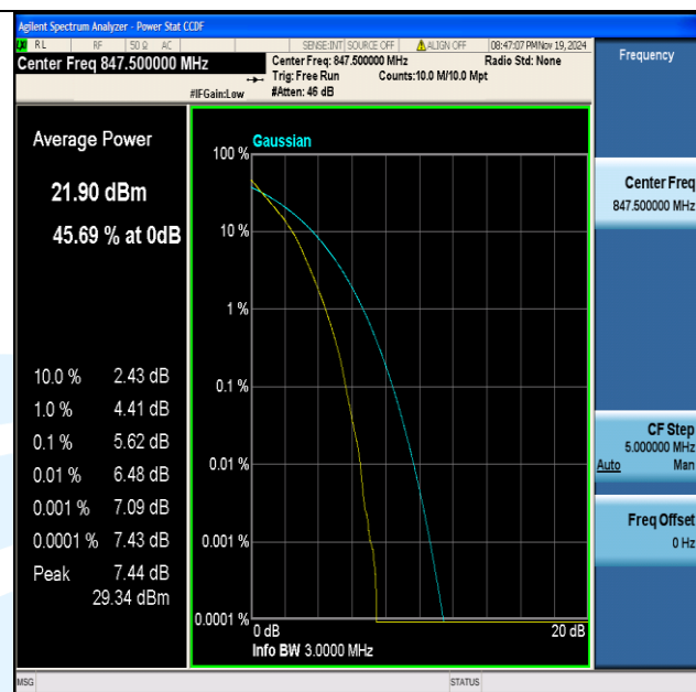
Band5-3MHz-QPSK-20635-15RB#0-PASS
