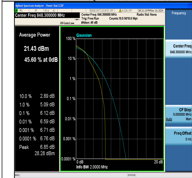
Band5-1.4MHz-16QAM-20643-1RB#0-PASS
