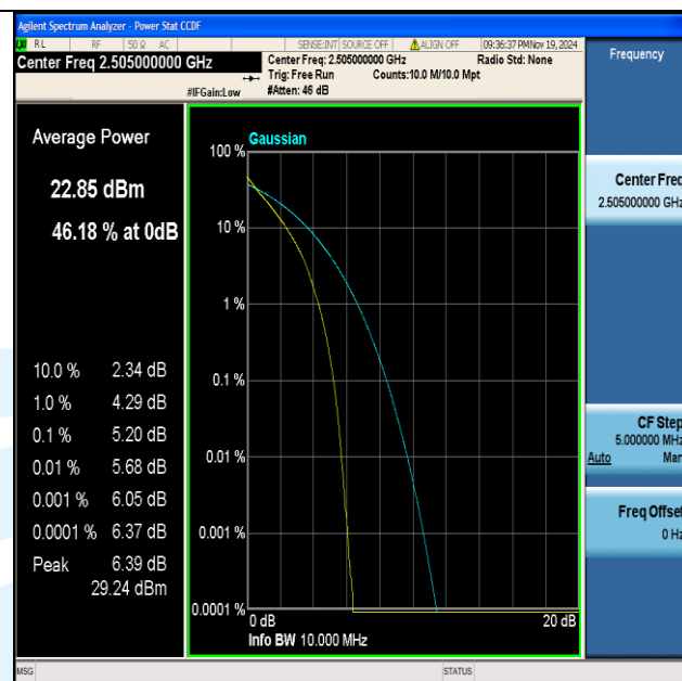
Band7-10MHz-QPSK-20800-50RB#0-PASS
