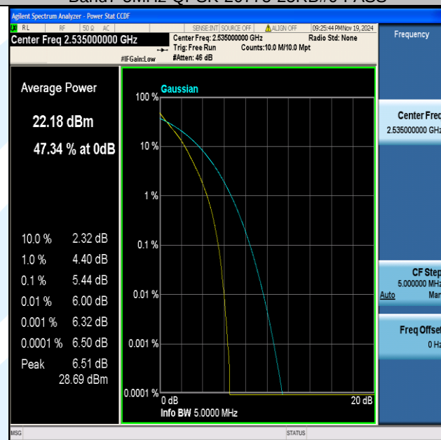
Band7-5MHz-QPSK-21100-25RB#0-PASS
