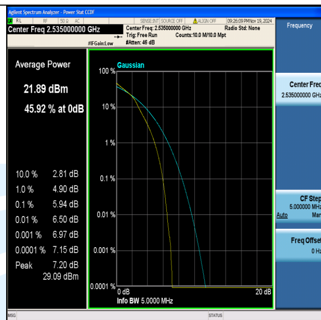
Band7-5MHz-16QAM-21100-25RB#0-PASS
