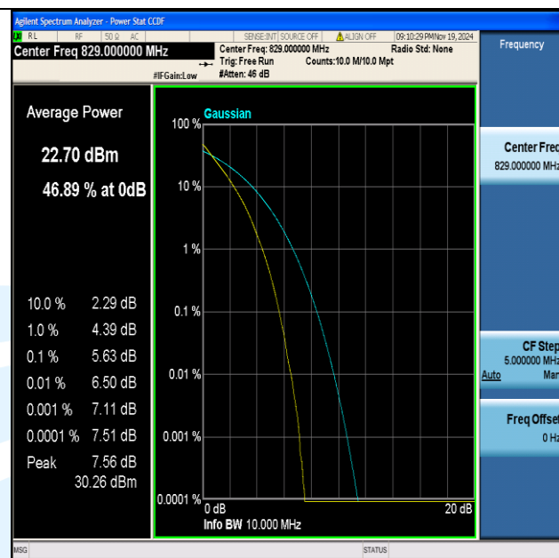
Band5-10MHz-QPSK-20450-50RB#0-PASS
