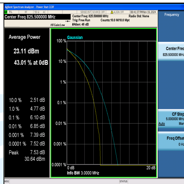
Band5-3MHz-QPSK-20415-15RB#0-PASS
