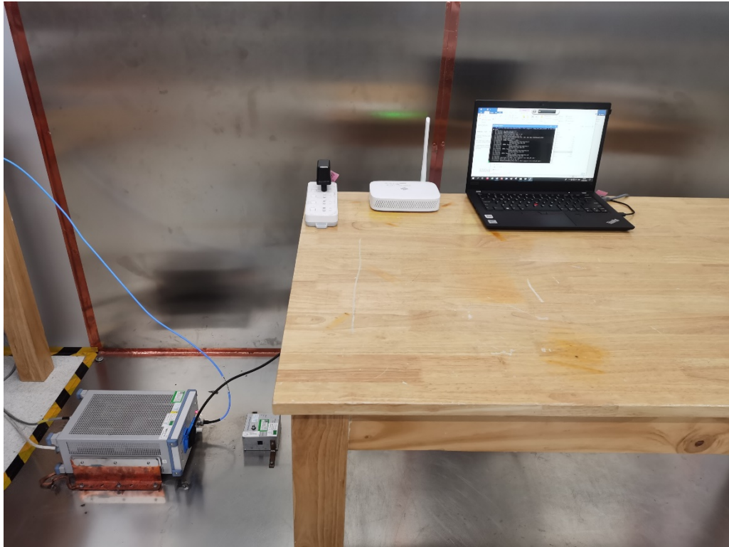
Photograph 3: Set-up for Conducted Emissions, AC Mains
