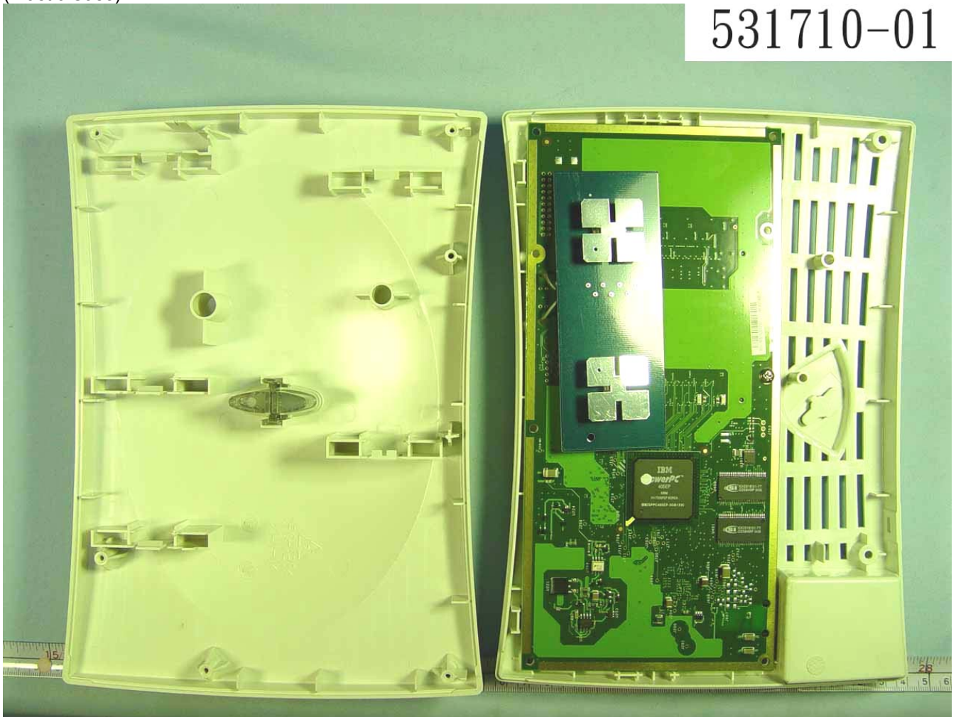
Plastic Housing (Plastic Case)
