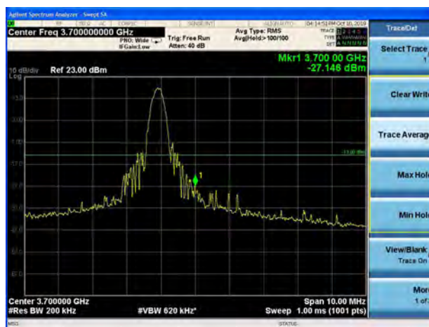
LTE Band 48 20MHz QPSK 100%RB CH-High
