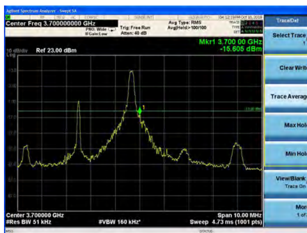
LTE Band 48 5MHz 16QAM 1RB CH-High
