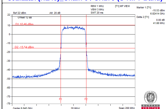
802.11ax (HE40)_Chain 0 / CH179 (U-NII-7 Band)
