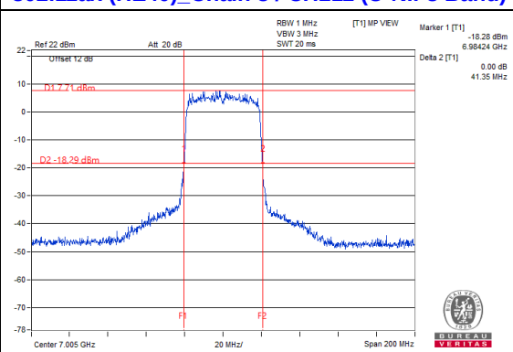
802.11ax (HE40)_Chain 3 / CH211 (U-NII-8 Band)
