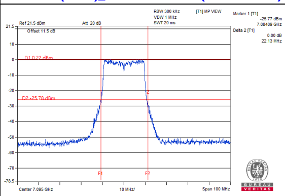
802.11ax (HE20)_Chain 1 / CH229 (U-NII-8 Band)
