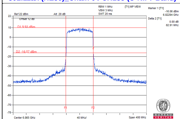
802.11ax (HE80)_Chain 0 / CH183 (U-NII-7 Band)
