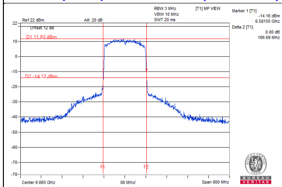
802.11ax (HE160)_Chain 3 / CH143 (U-NII-7 Band)
