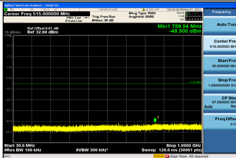
Band25-5MHz-QPSK-26365-1RB#0-30~1000MHz
