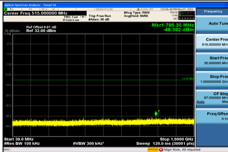
Band25-10MHz-16QAM-26090-1RB#0-30~1000MHz
