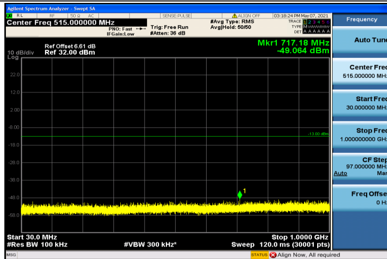
Band25-20MHz-16QAM-26140-1RB#0-30~1000MHz
