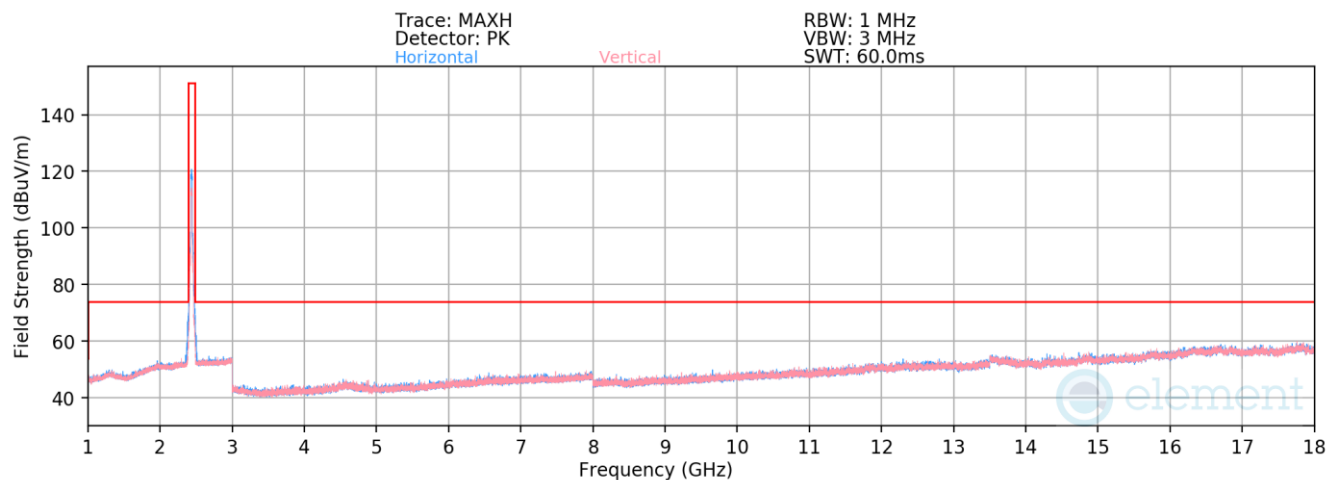
Plot 7-454. Radiated Spurious Emissions above 1GHz CDD (802.11ax (SU) – Ch. 6)
