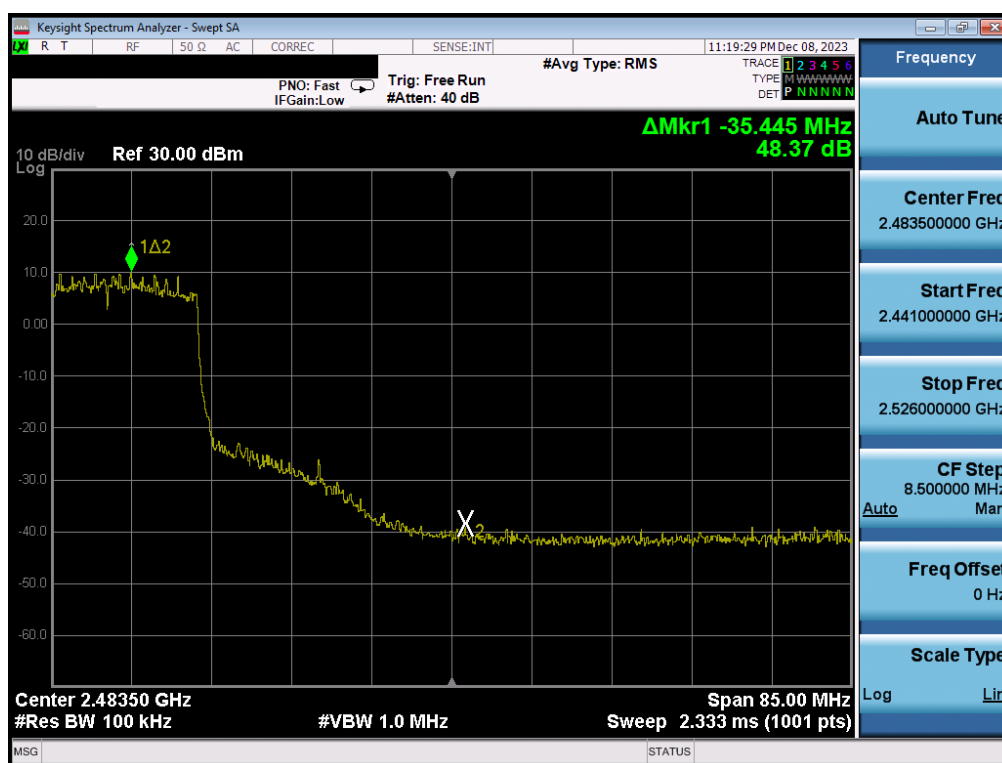
Plot 7-375. Band Edge Plot Antenna WF2b (802.11ax(SU) - (2.4GHz) - Ch. 8) - MCS4
