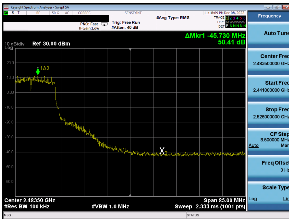
Plot 7-361. Band Edge Plot Antenna WF2b (802.11n (2.4GHz) – Ch. 8) – MCS4
