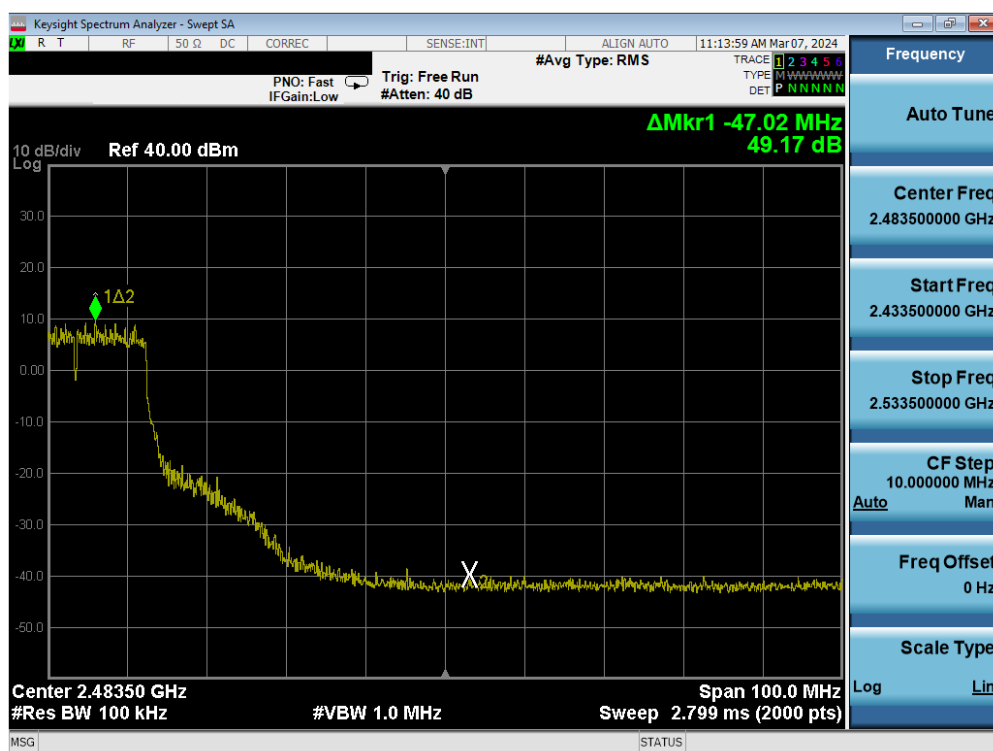
Plot 7-404. Band Edge Plot Antenna WF2b (802.11n (2.4GHz) – Ch. 6 (high)) – MCS7
