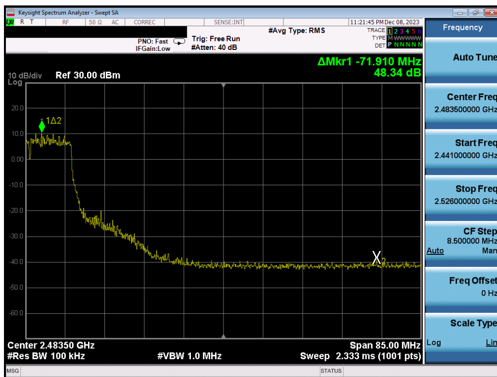
Plot 7-405. Band Edge Plot Antenna WF2b (802.11n (2.4GHz) – Ch. 7) – MCS7
